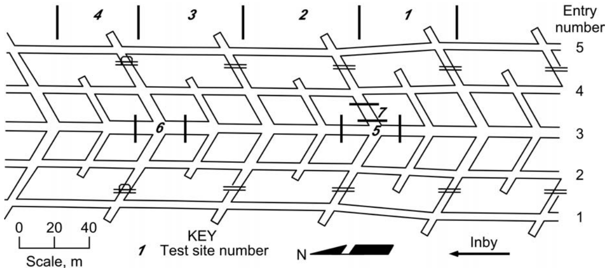
Figure 3.—Plan view of test sites.
