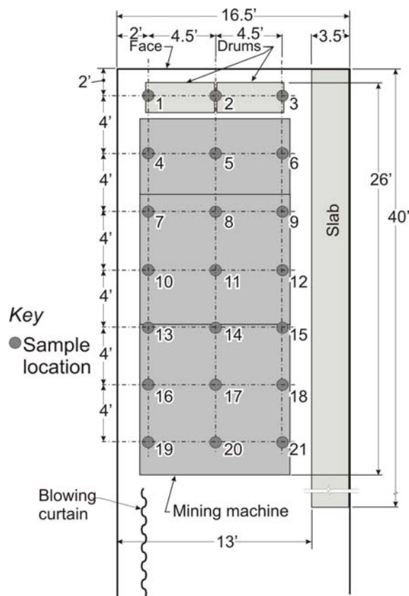
Figure 5. Ventilation gallery methane sampling locations above mining machine.
