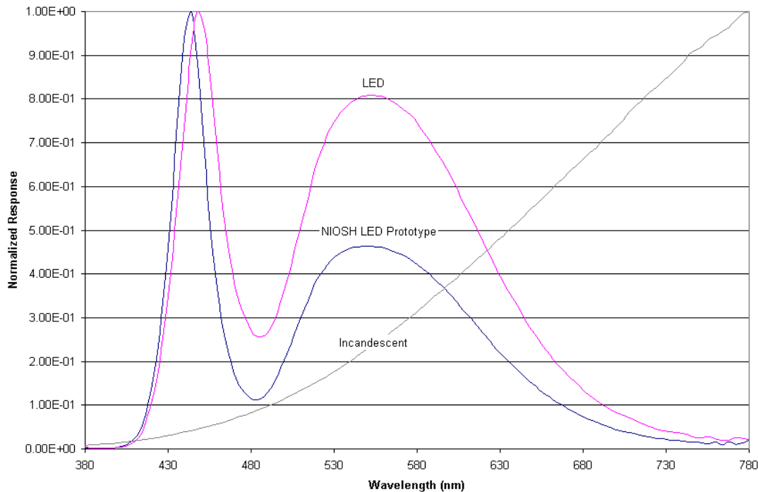
Figure 3. The spectral power distributions for each cap lamp as normalized at their maximum values. The diffusion filters, used to normalize target illuminance, were on each cap lamp.
