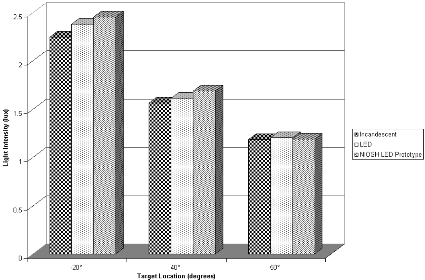
Figure 4. The average target illuminance from each cap lamp when applying a diffusion filter to the cap lamps.
