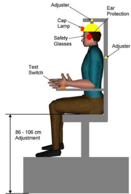
Figure 2. The observation station used for human subject testing.
