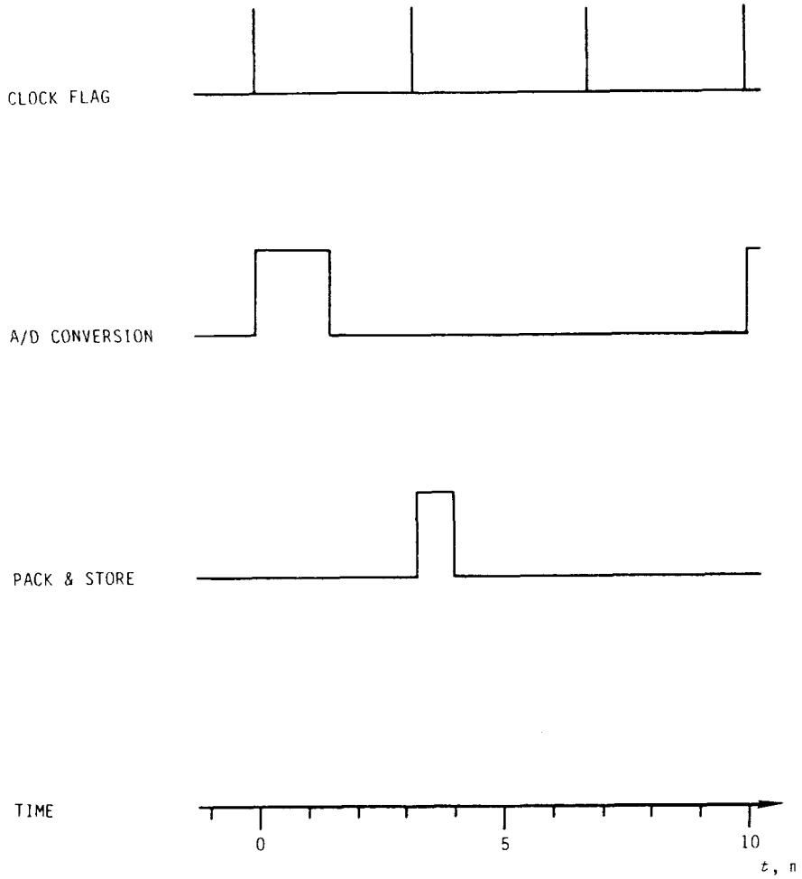
Figure 2-4. Timing.
