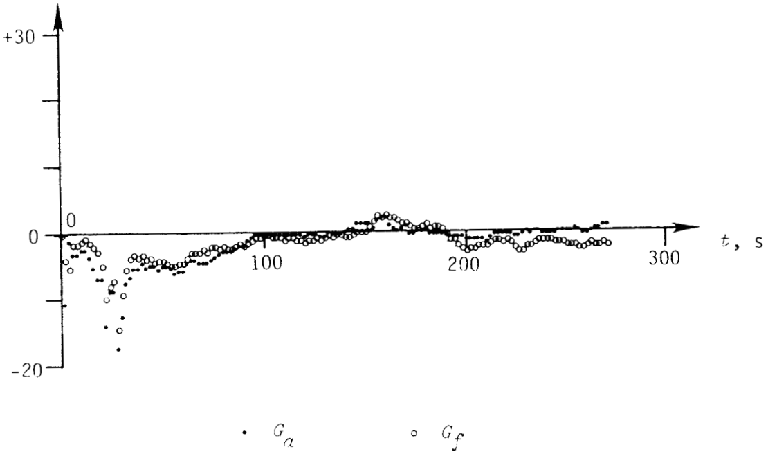
Figure 5-3. Convergence plot for data set #6-2A (Z axis).
