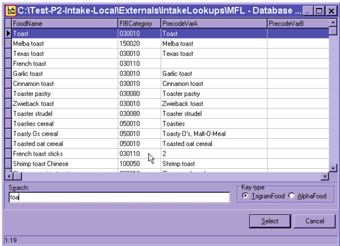
Exhibit 6-10. Trigram search
