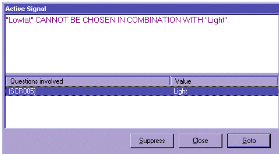
Exhibit 6-60. Edit messages
