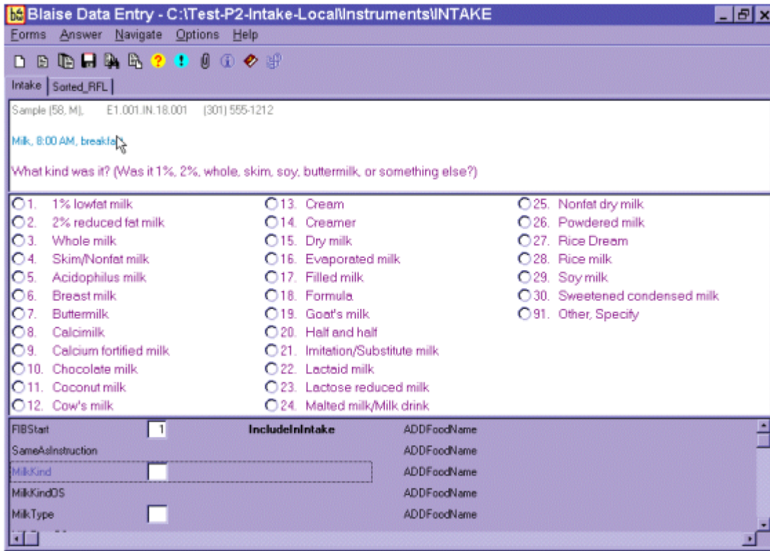
Exhibit 6-44. Response items
