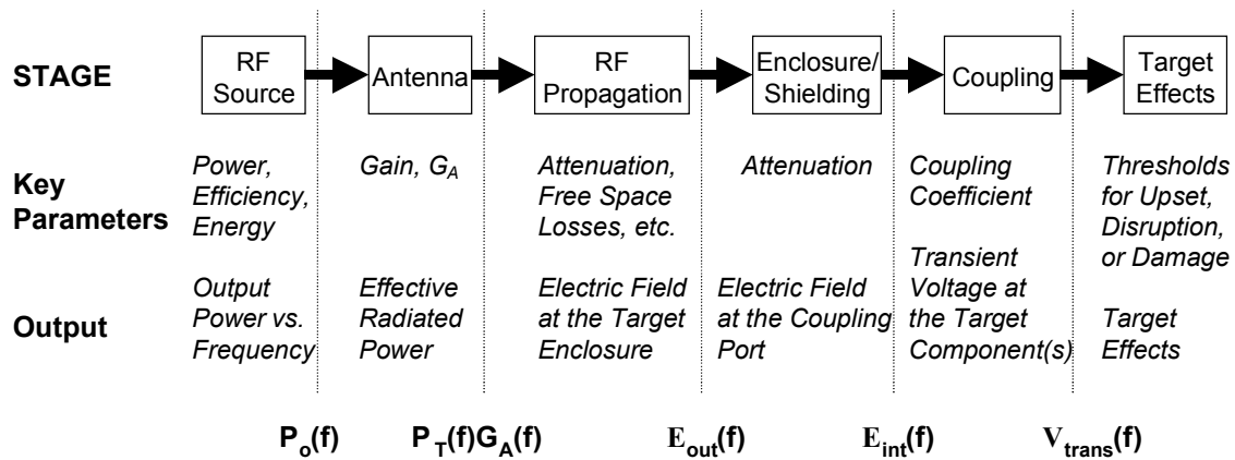
Figure 1: Stages in a HPRF/HPM Engagement
