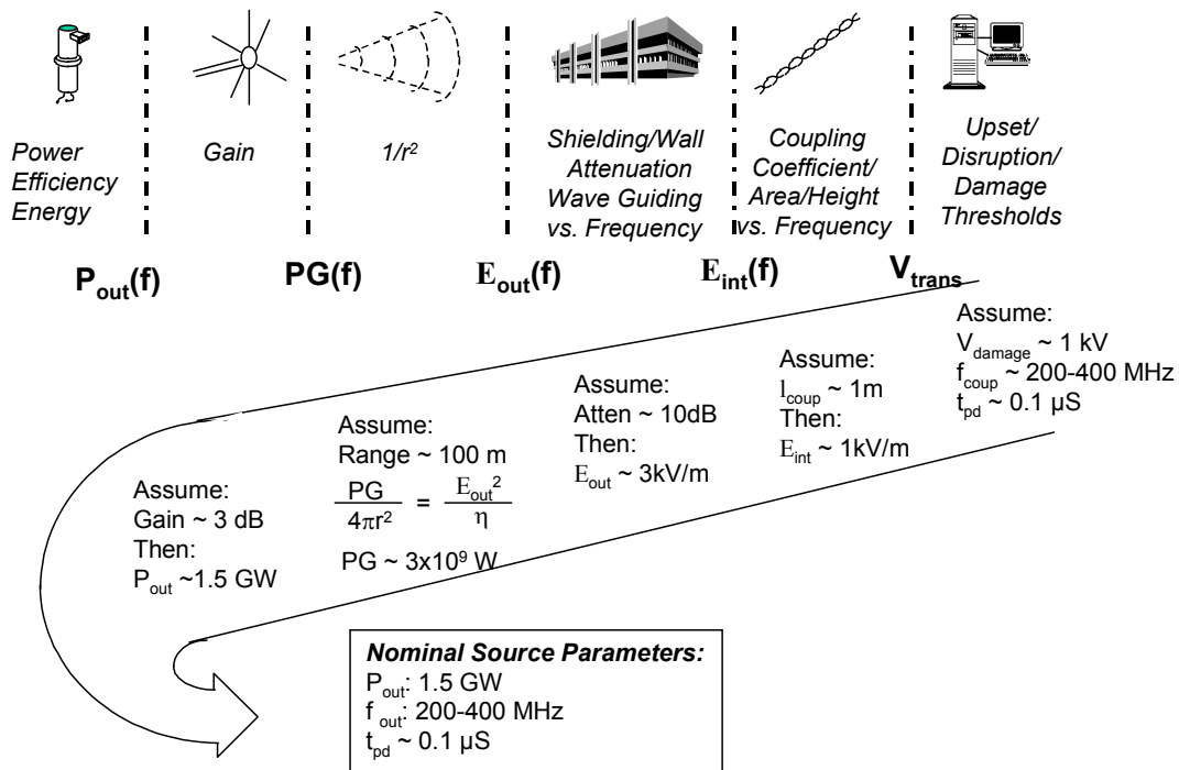
Figure 2. Notional Example of End-to-End Analysis, Working Backward from Required Induced Transient Voltage to Estimated Source Parameters
