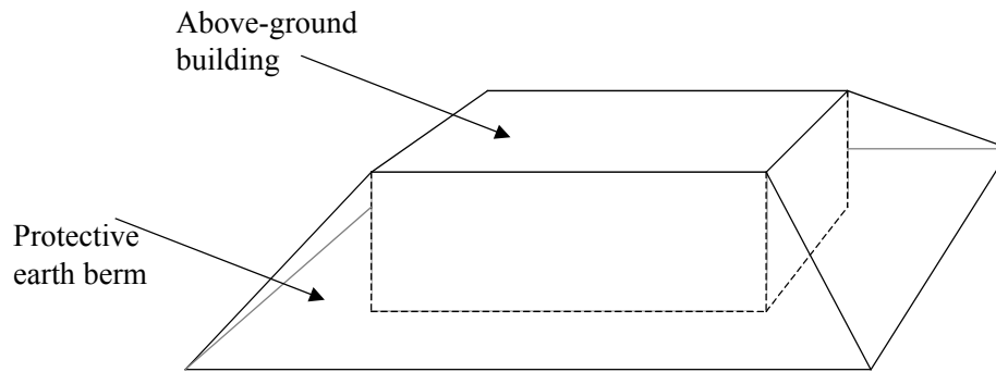
Figure 6: Slanted Earth Berms Protecting an Above-Ground Building from Blast Effects
