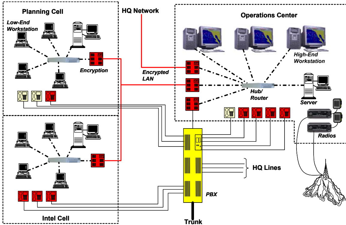
Figure 4. Notional Command and Control Node
