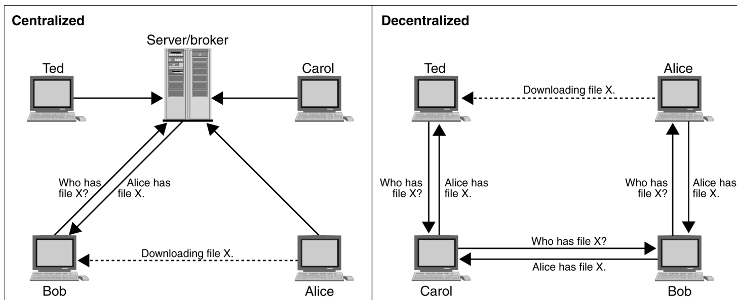
Figure 4: Peer-to-Peer Models
