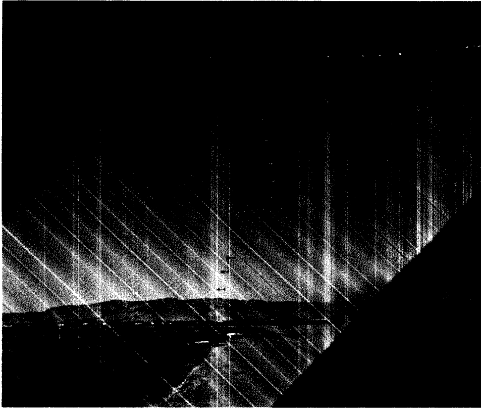
The time-displacement record of a V/TOL aircraft, the X-14, was made with a Fairchild Photographic Flight Analyzer Camera. The camera is arranged so that the entire background and fixed scene are properly exposed, but each element of the scene is exposed at the particular time when the aircraft passes over it. This time is determined by the tracking mechanism and the individual time of each image is recorded on the edge of a strip on the originally exposed film.
