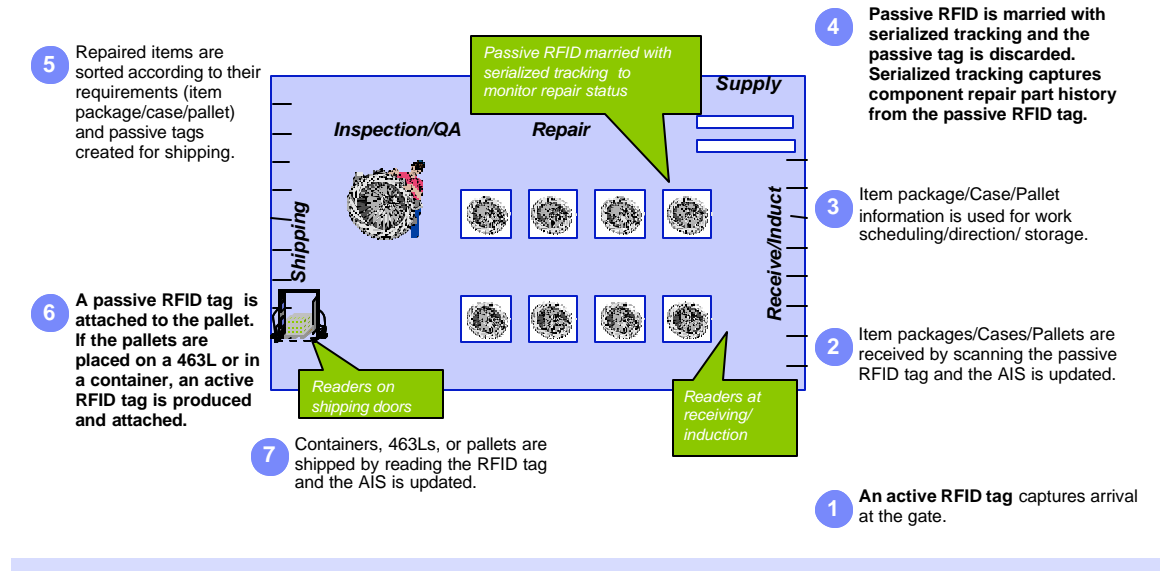
Figure 18 Repair Depots
