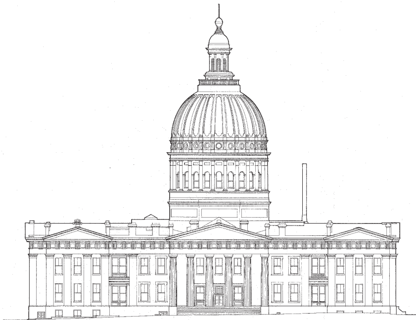
WEST ELEVATION B ROADWAY
