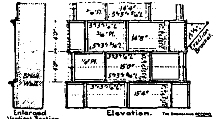
DETAILS OF CASING.
