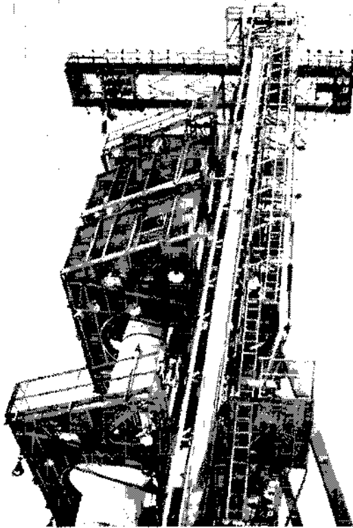
Mercury/Redstone spacecraft and service structure, Air Force Space Museum (complex 26B), Cape Canaveral Air Force Station, 1981
