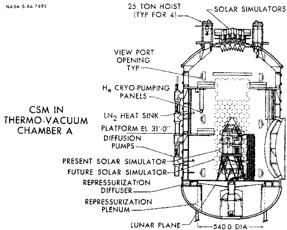
Space environment simulation laboratory, chamber A diagram
