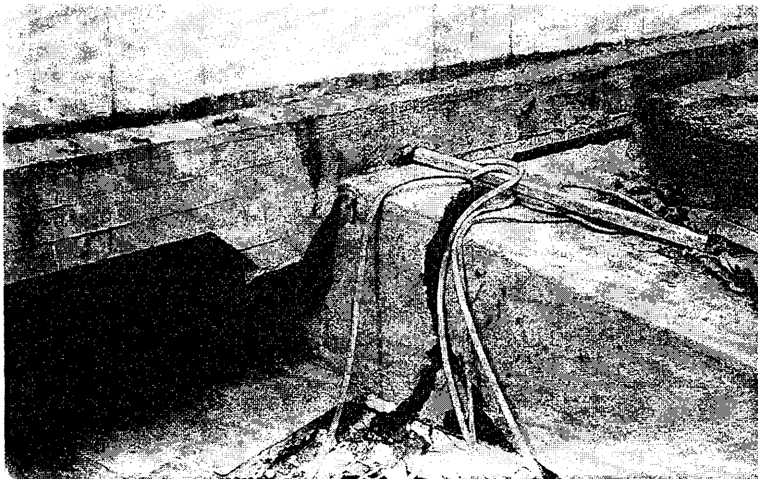
Reinforced concrete slab which originally supported the earthen terrace next to the Mnyami, showing damage by settlement before its foundation was carried to bedrock.
