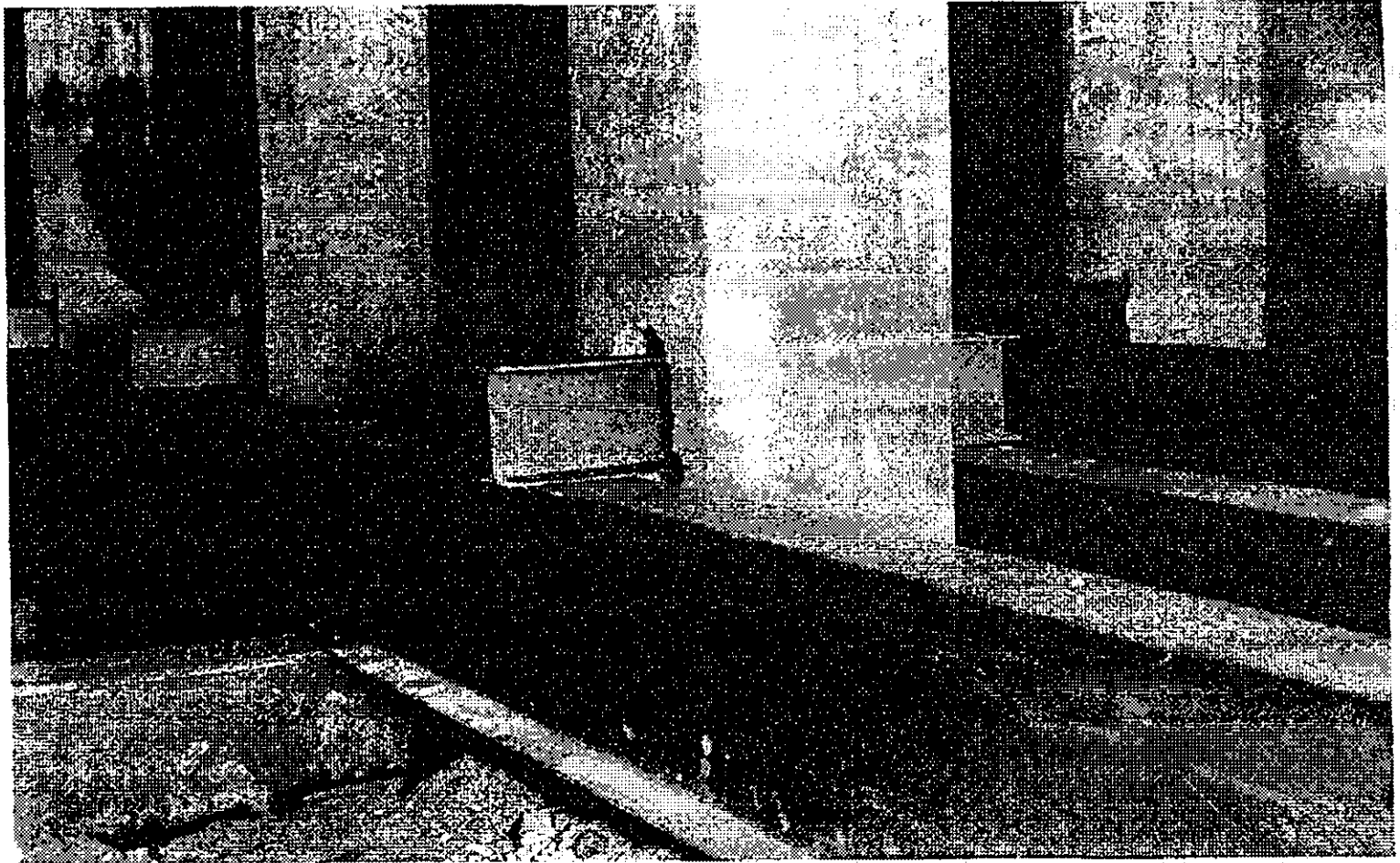
System of steel girders used to support the approach to the Lincoln Memorial when their foundations were strengthened
