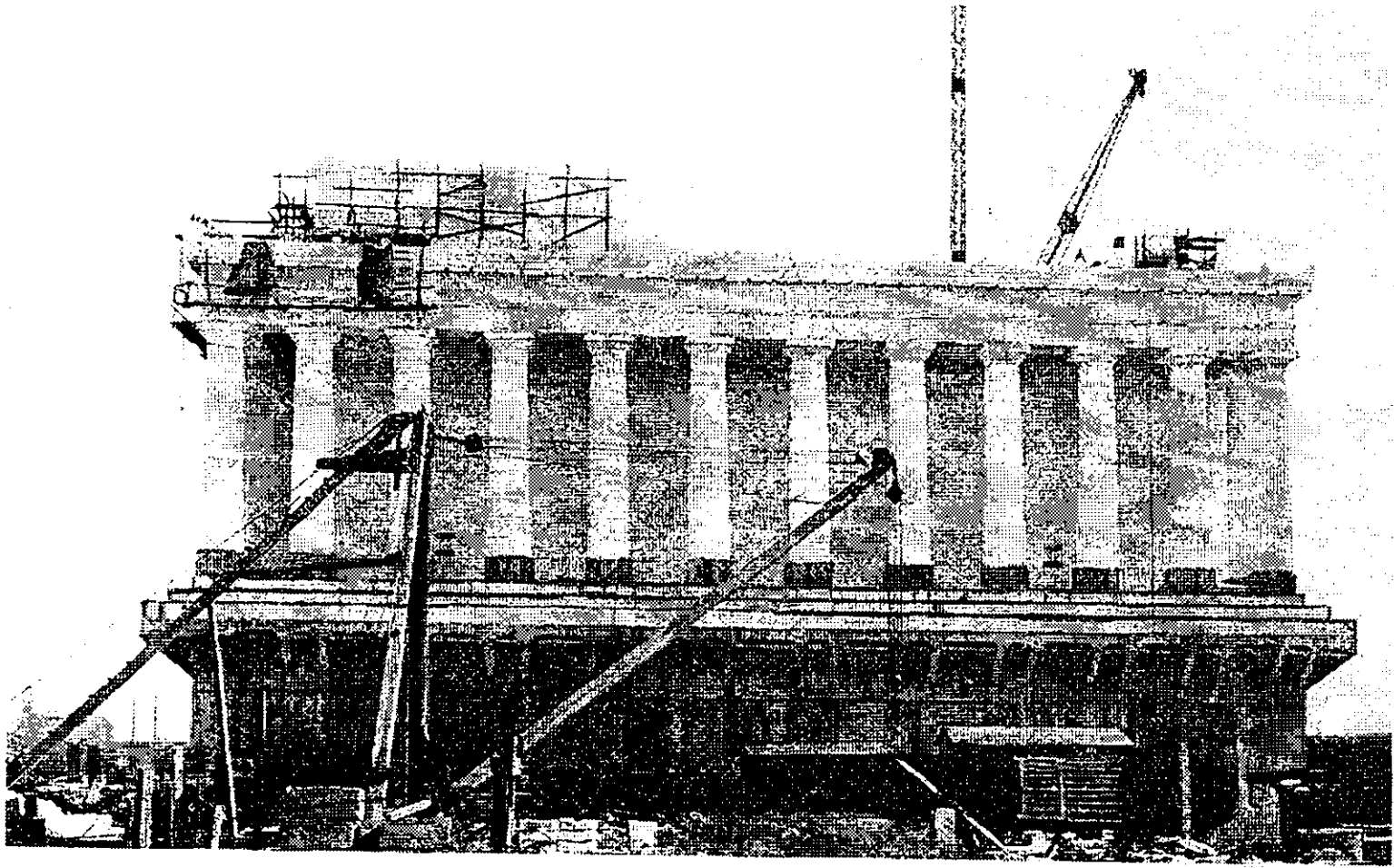
Setting steel work west front October 1, 1916
