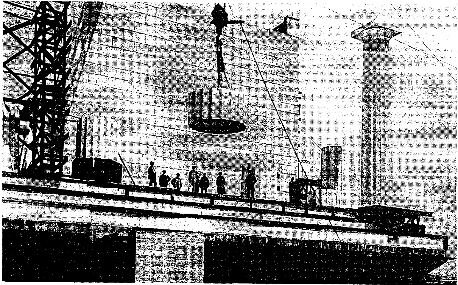
Setting exterior columns, south front
