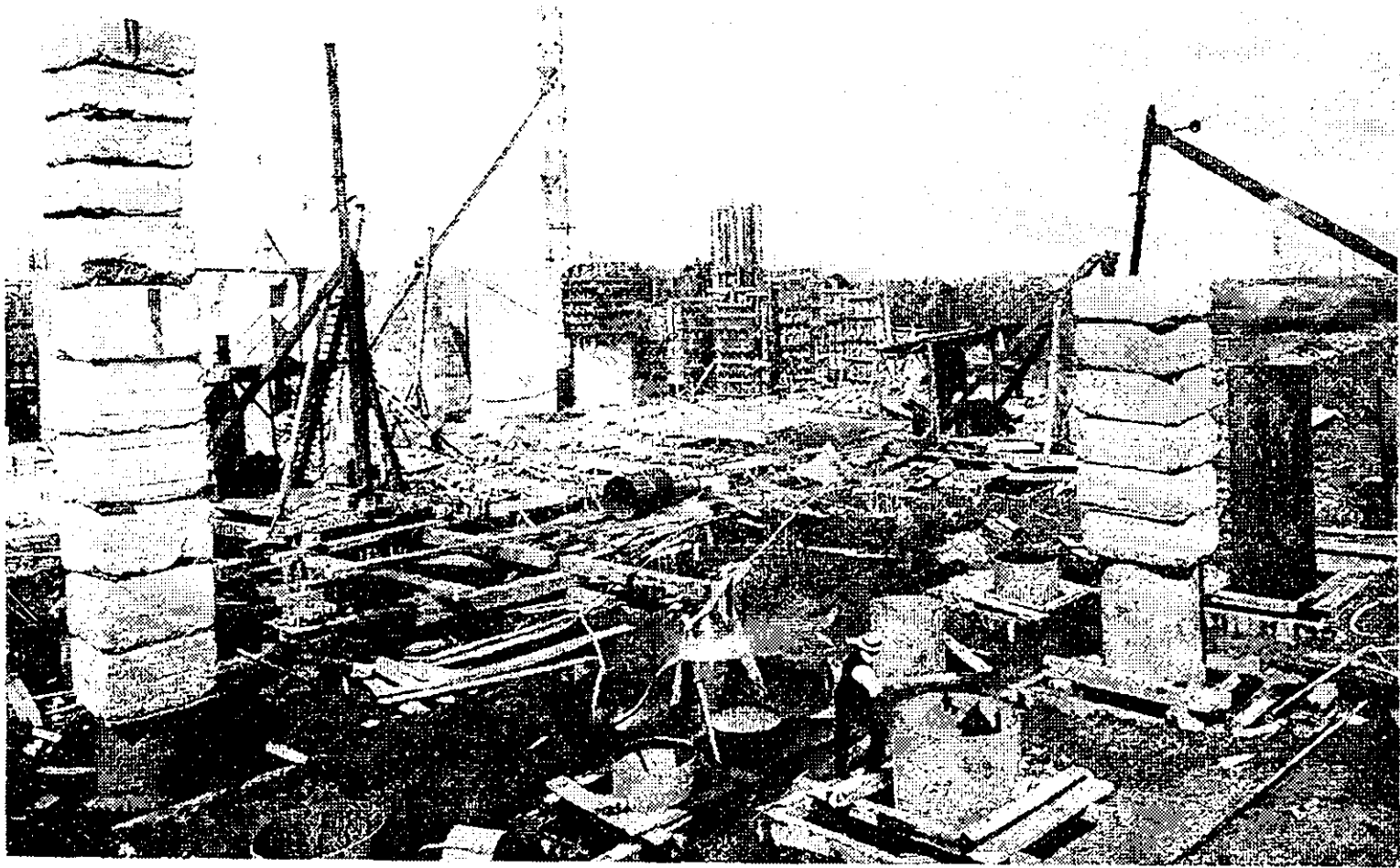
Weighting used in sinking cylinders for subfoundations; also constructing upper concrete foundation. (September 1, 1914)
