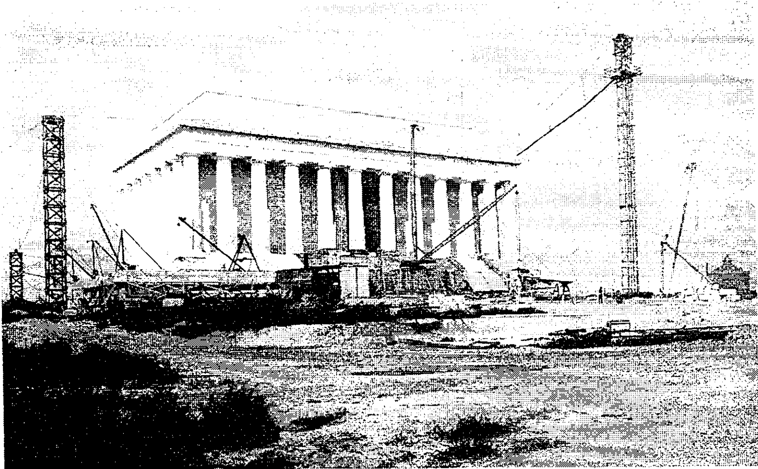
Setting retaining wall for terrace, south front. (November 1, 1915)
