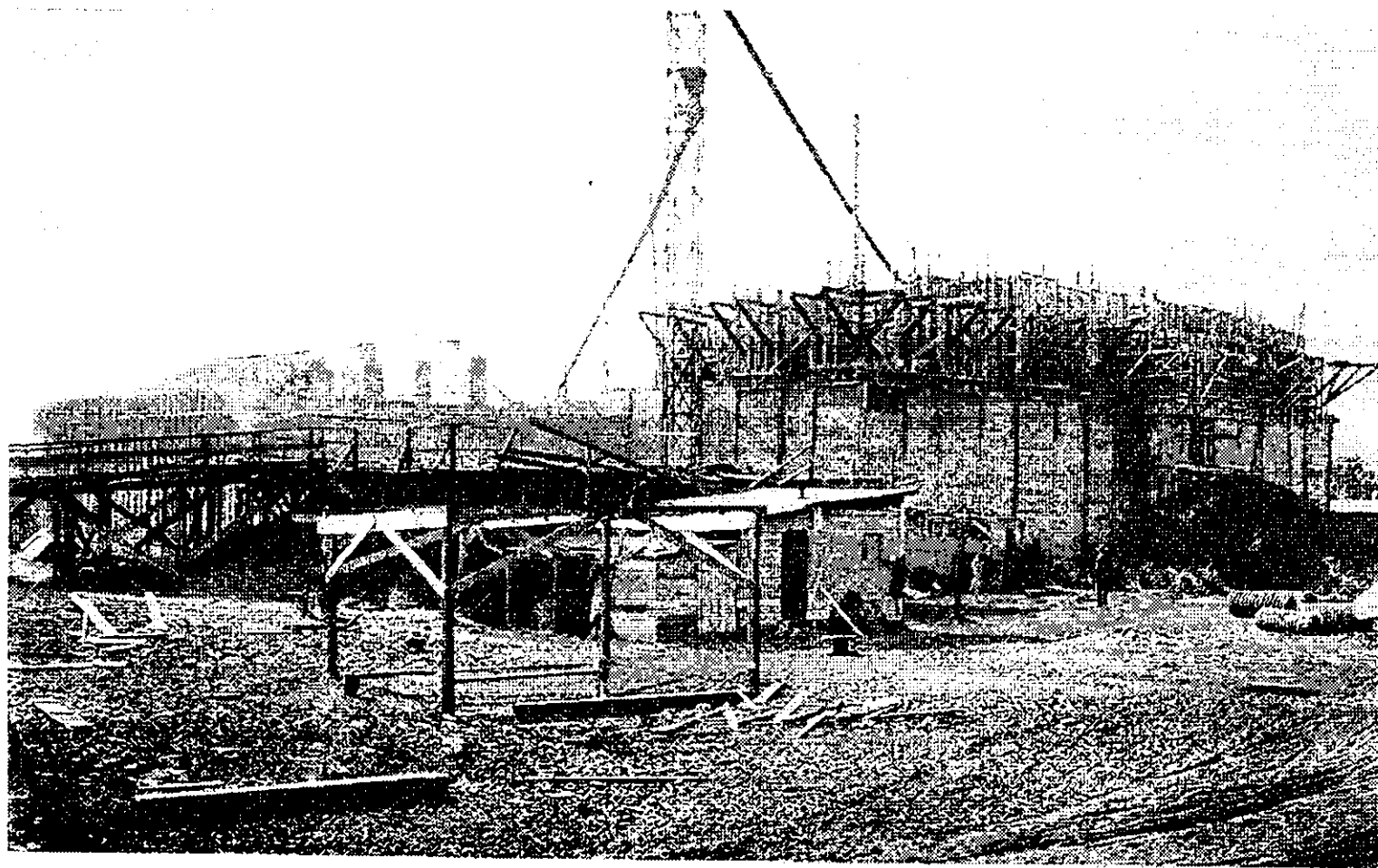
Constructing upper foundation. View showing east and north fronts. (November 2, 1914)
