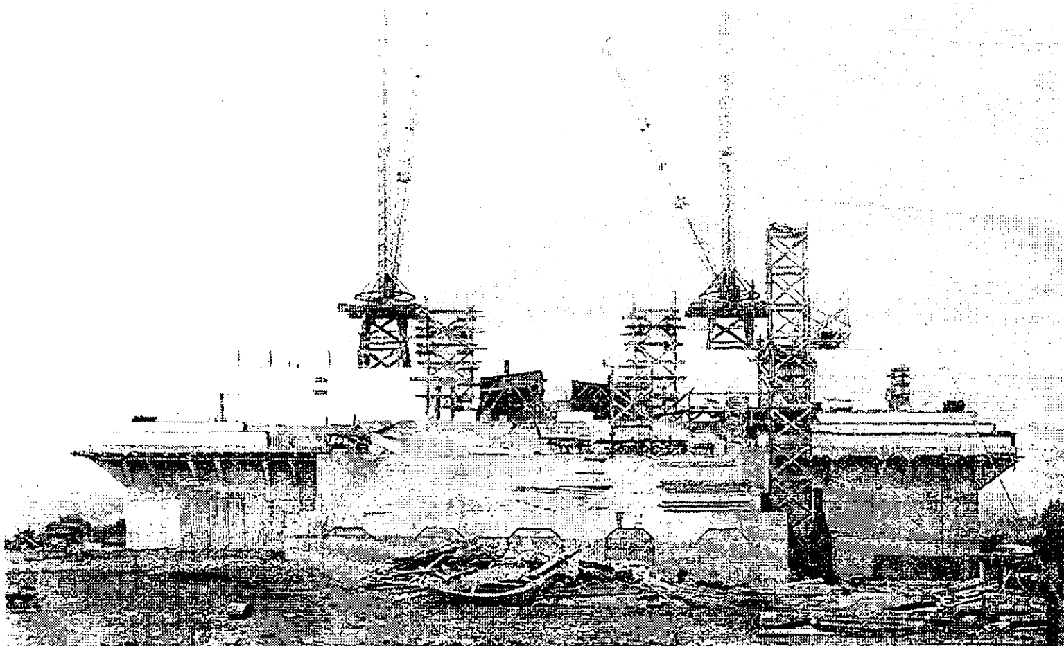
Setting the marble exterior walk of the superstructure, east front (June 1, 1915)
