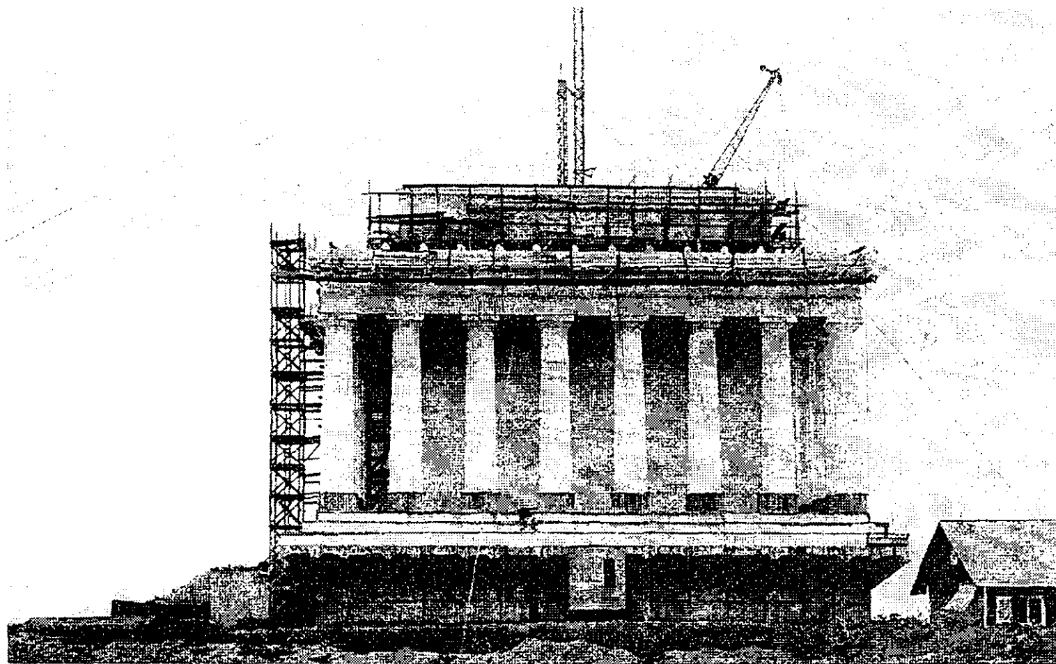
Carving the ornamentation on frieze and attic story, north front. (August 1, 1916)
