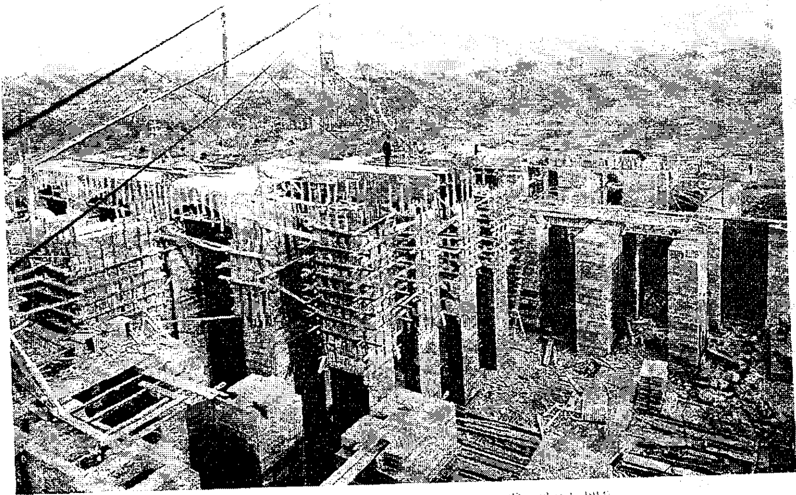
View from top of upper foundation looking northeast. (December 1, 1914)
