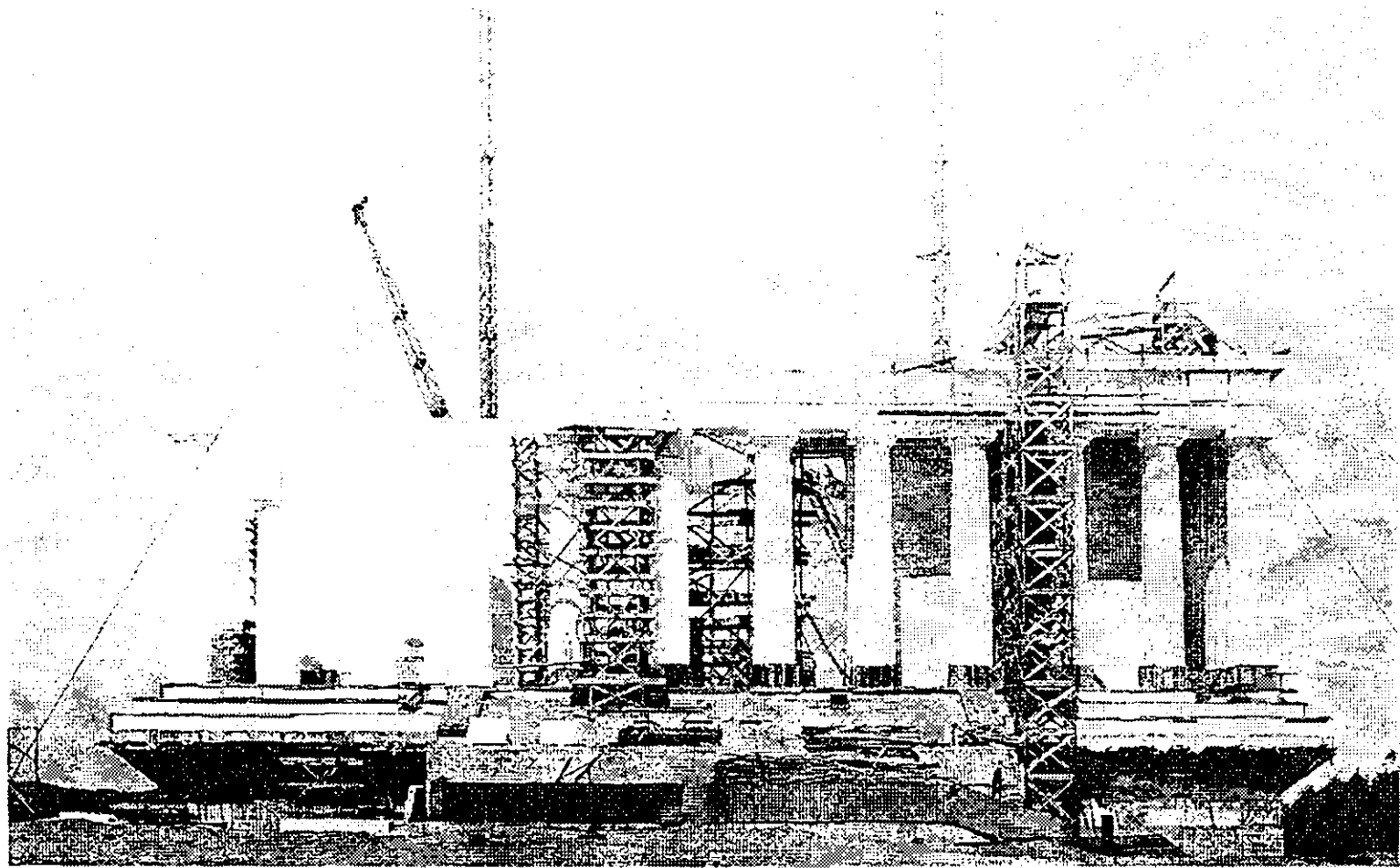
Scaffolding the columns and frieze, east front (June 1, 1916)
