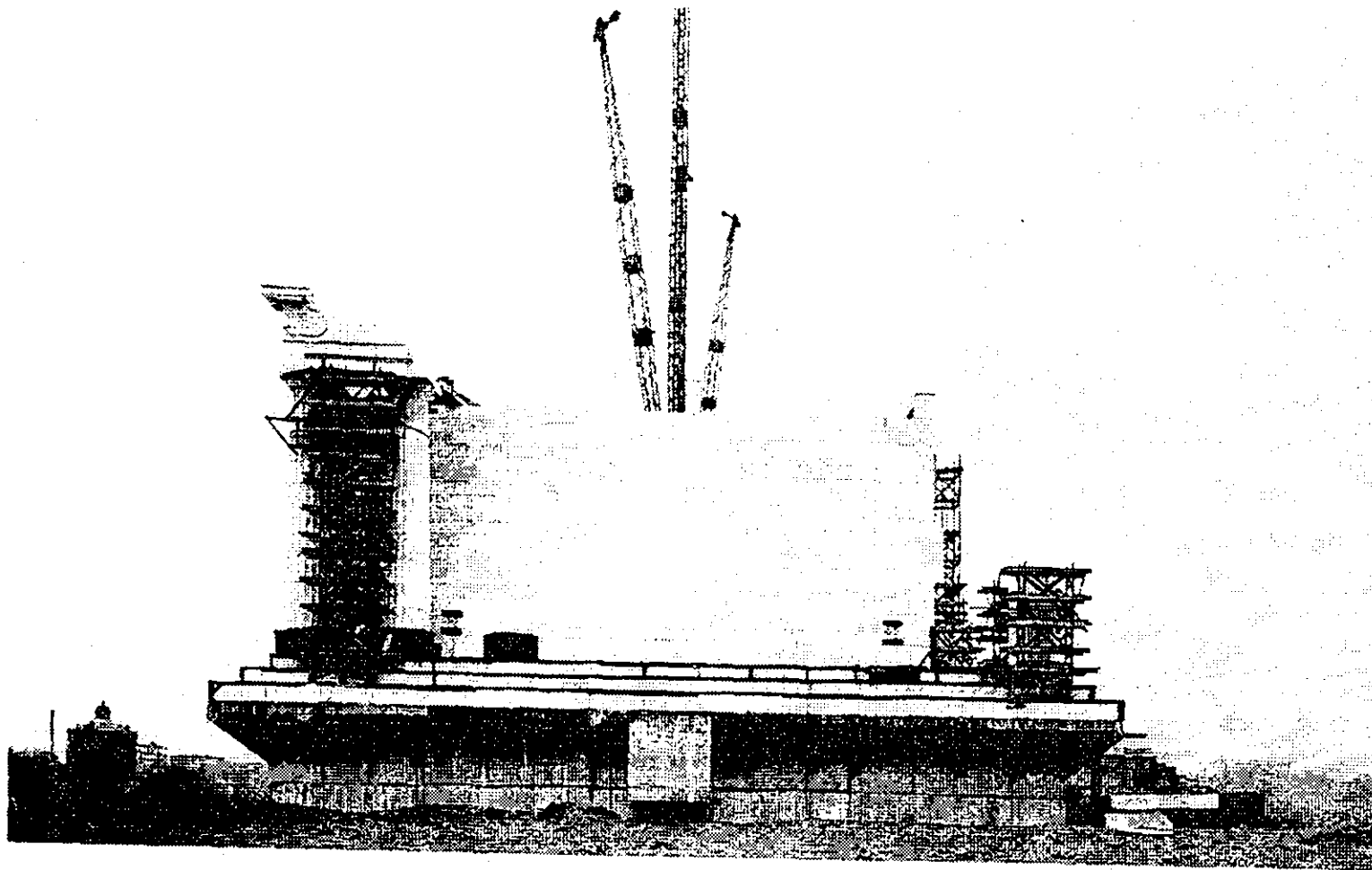
Setting the fins at the southwest corner of the Memorial (April 1, 1970)
