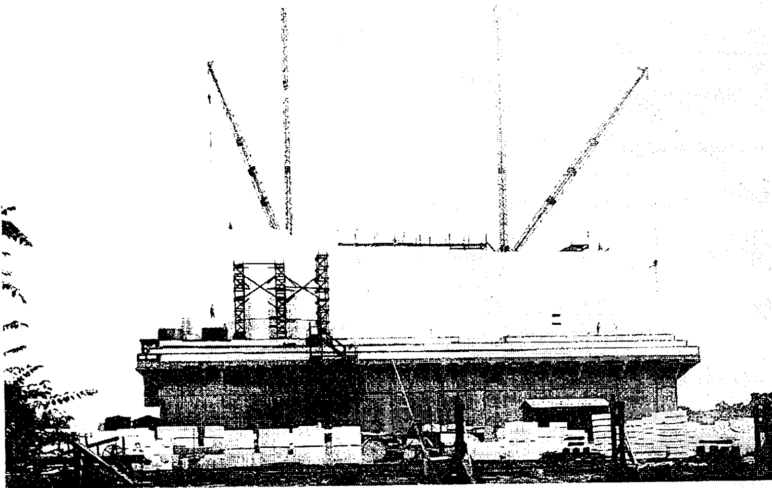
Setting exterior walls and columns - east front. July 31, 1915.
