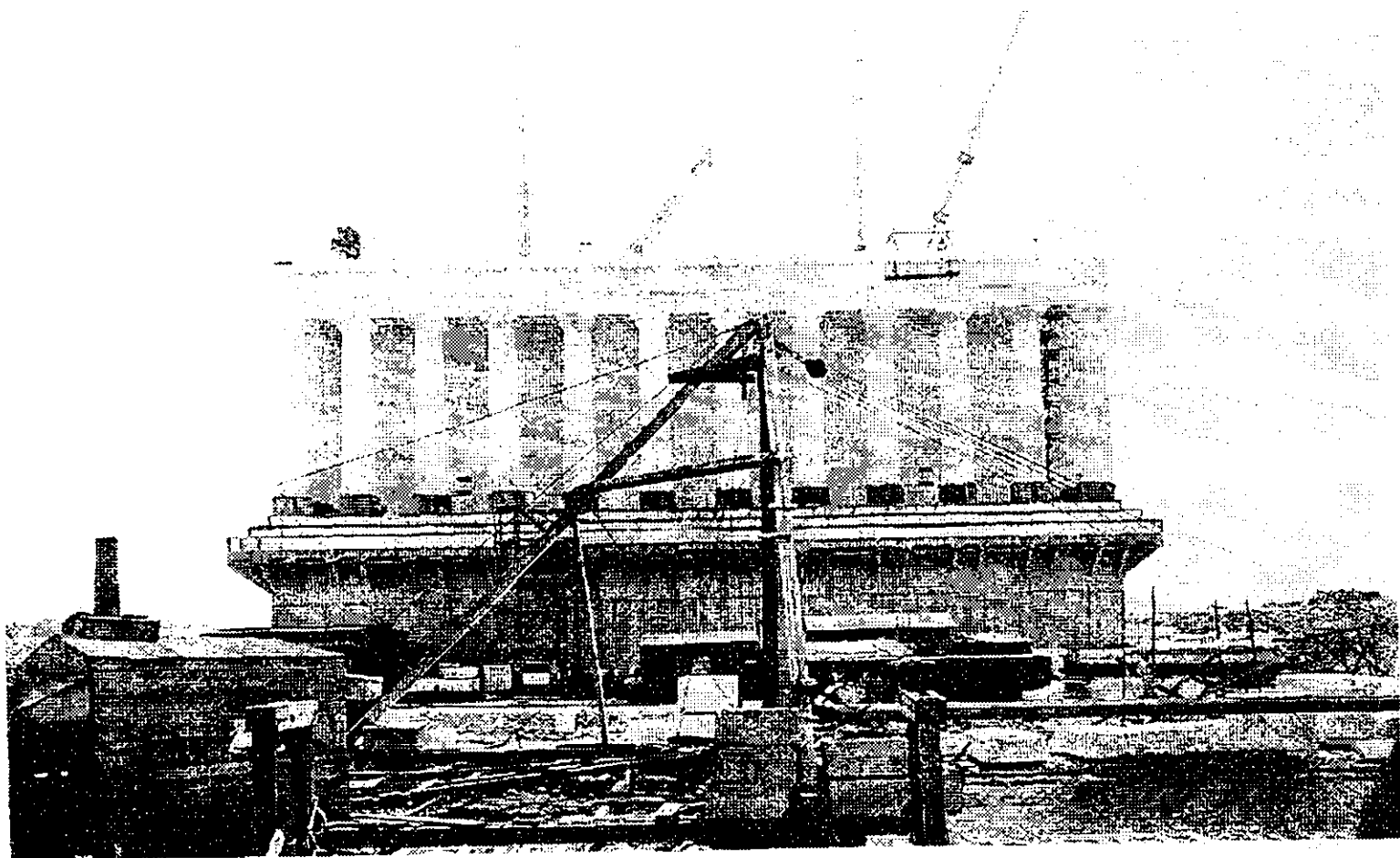
Compassing the setting of the attic story, west front. (June 1, 1916)
