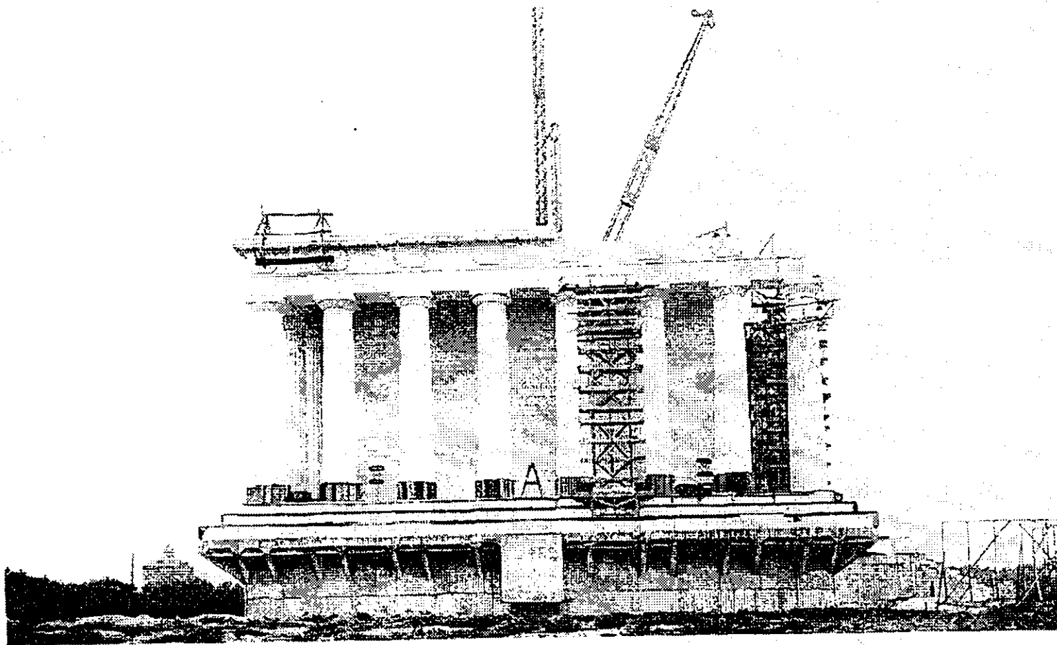
Setting the eaststones of the frieze, south front. (August 1, 1919)
