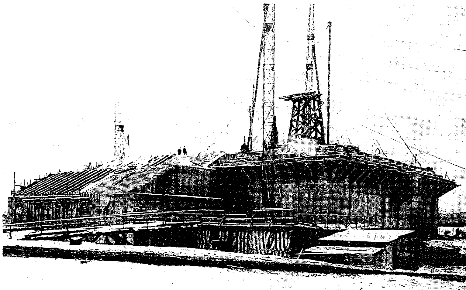
The reactor foundation east and north fronts. (February 4, 1953)
