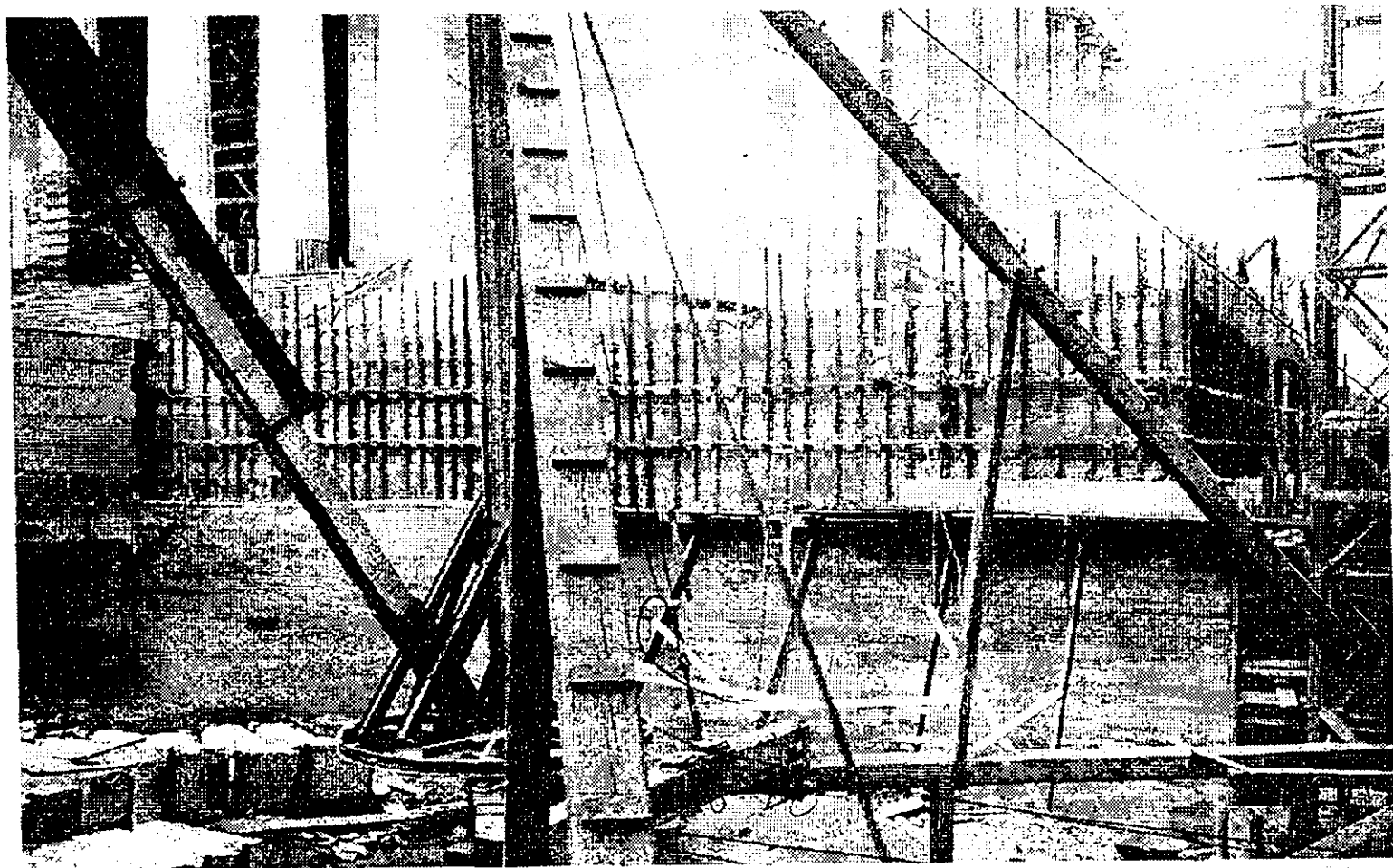
Setting temporary wall of terrace - northeast corner - April 1, 1949
