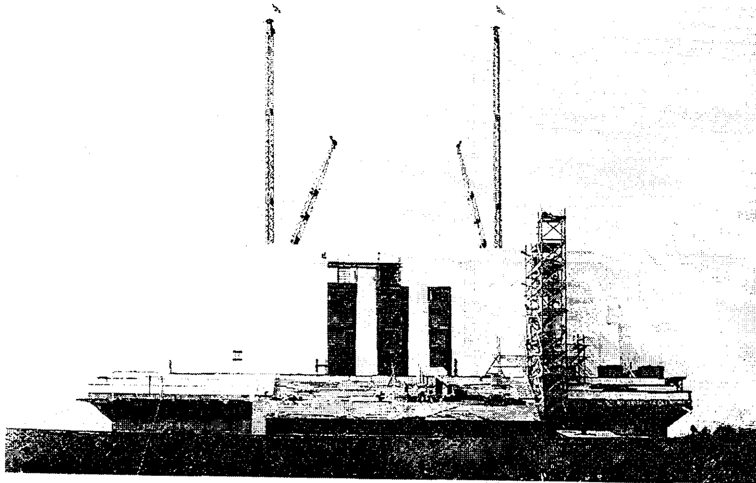
Setting exterior walls and columns, east front. (November 1, 1915)
