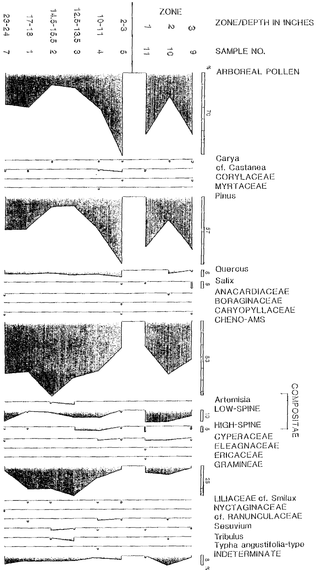
FIGURE 1. POLLEN DIAGRAM FROM THE DOUGLAS BEACH SITE, FLORIDA.
