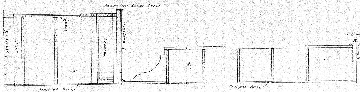
SECTION THRU CABINET IN KITCHEN. SEE ORIG. DRAWINGS. SCALE 1/2" = 1'-0"
