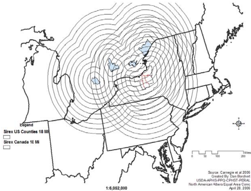
Figure 10. Estimated Spread of Sirex noctilio over 10 years. The above figure utilizes an 18 mile/year spread rate in the United States and Canadian counties currently reporting detection.
