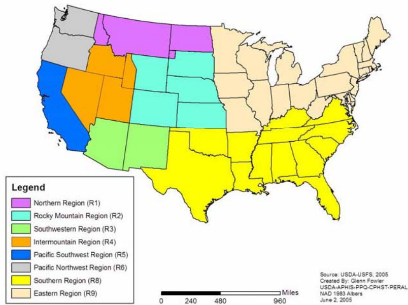
Figure 8. USFS Regions
