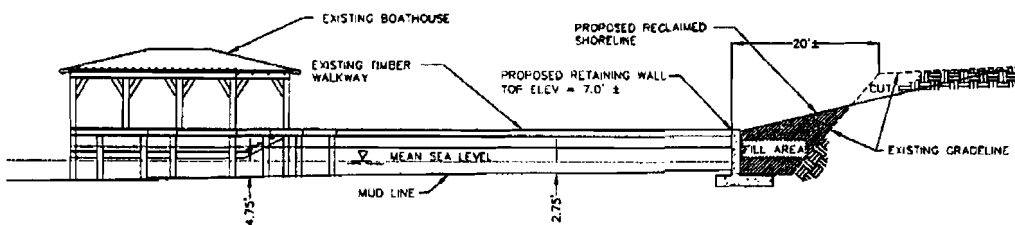
PROFILE OF PROPOSED SHORELINE IMPROVEMENTS
