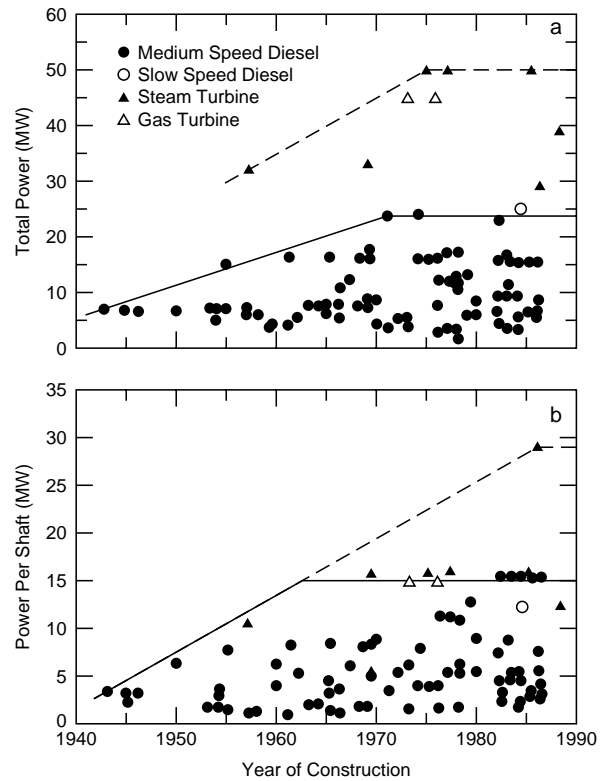
Figure 18. Prime movers installed on icebreaking ships: (a) total power vs. year of construction, and (b) power per shaft vs. year of construction (after Dick and Laframboise 1989).
