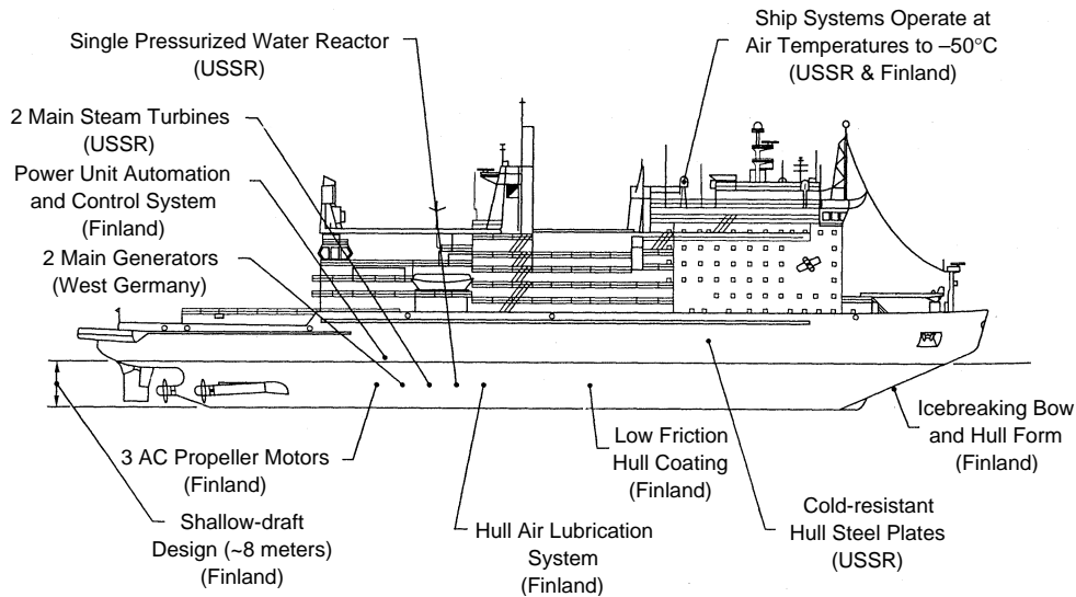
Figure 4. Taymyr-class shallow-draft nuclear icebreaker (after Brigham 1991).
