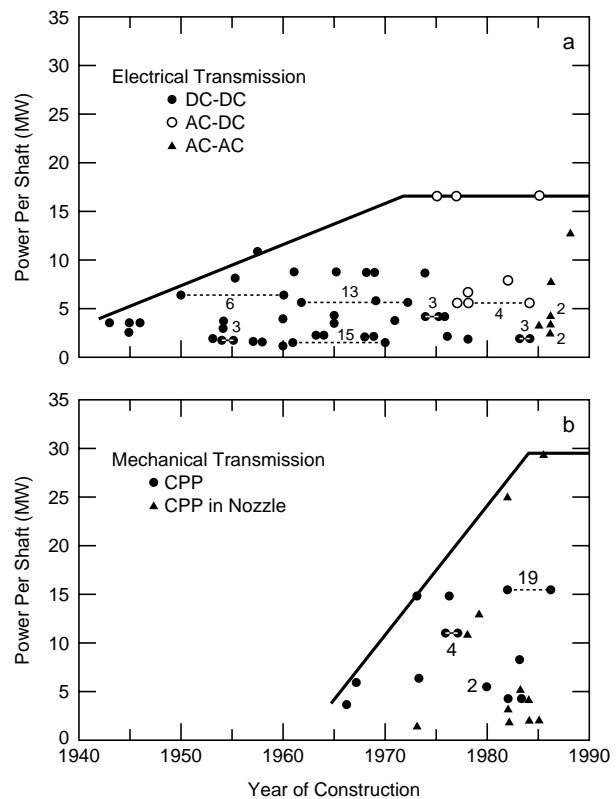
Figure 15. Shaft power vs. year of construction for icebreaking ships: (a) electrical transmission system, and (b) mechanical transmission system (after Dick and Laframboise 1989).
