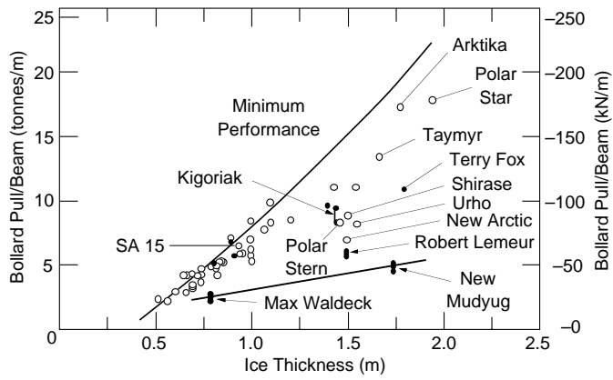
Figure 21. Icebreaking performance: bollard pull/beam vs. ice thickness. Bollard pull is measured or calculated; data are adjusted for a speed of 2 knots (after Dick and Laframboise 1989).
