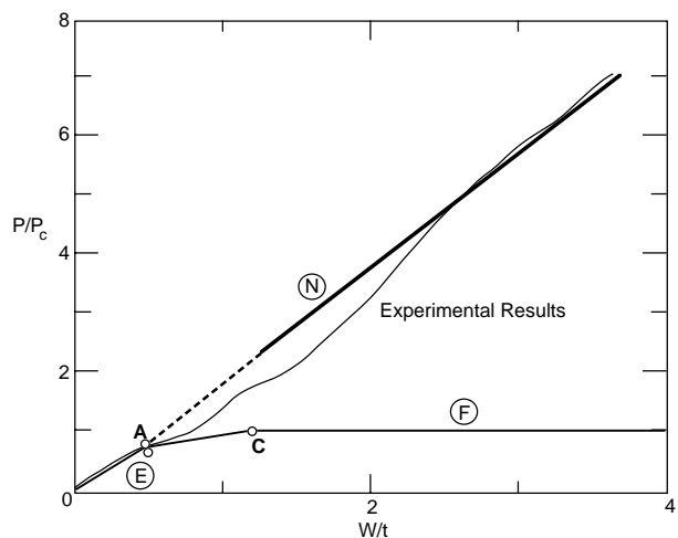
Figure 14. Pressure vs. deflection, showing domains of different behaviors from small to large deflection (after Ratzlaff and Kennedy 1986). Along the vertical axis, the applied pressure P is made nondimensional by P_c , the pressure at which collapse (point C) is assumed to take place by formation of three hinges without membrane action. Along the horizontal axis, the maximum deflection W is made nondimensional by the plate thickness t . The curve labeled E represents elastic flexure with an elastic membrane up to the complete formation of an edge hinge. The curve labeled F represents elastic flexure without membrane action, followed by the formation of the first hinge and then three hinges. The curve labeled N represents ideal membrane action.
