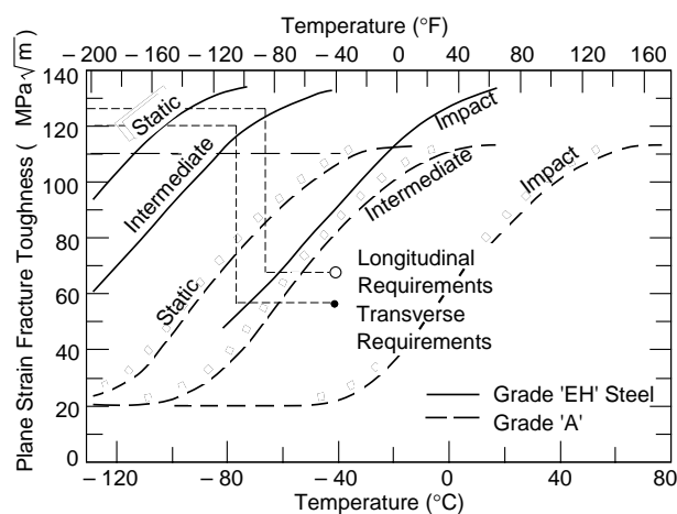
Figure 13. Plane strain fracture toughness vs. temperature for two grades of steel ("A" and "EH") (after Dick et al. 1987).
