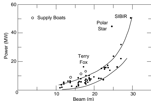
Figure 20. Power vs. beam for icebreakers (after Dick and Laframboise 1989).
