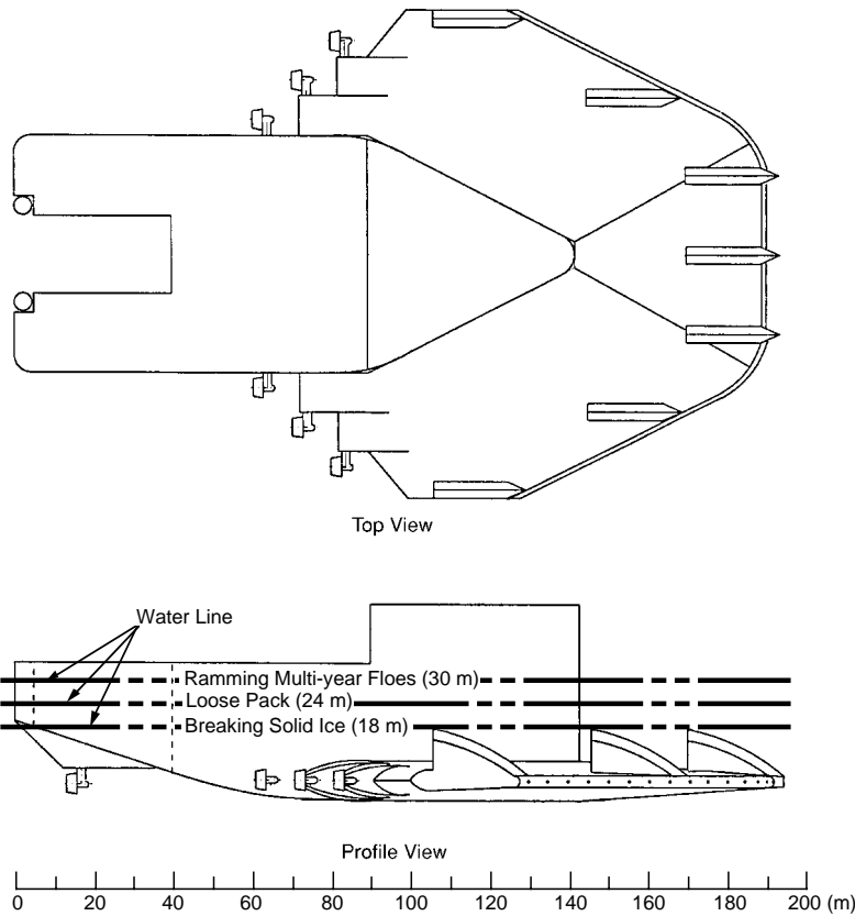
Figure 25. New "iceraking" concept, as proposed by Johansson et al. (1994).
