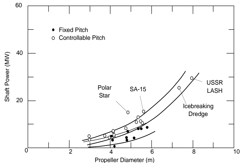
Figure 16. Shaft power vs. propeller diameter for icebreaking ships (after Dick and Laframboise 1989).
