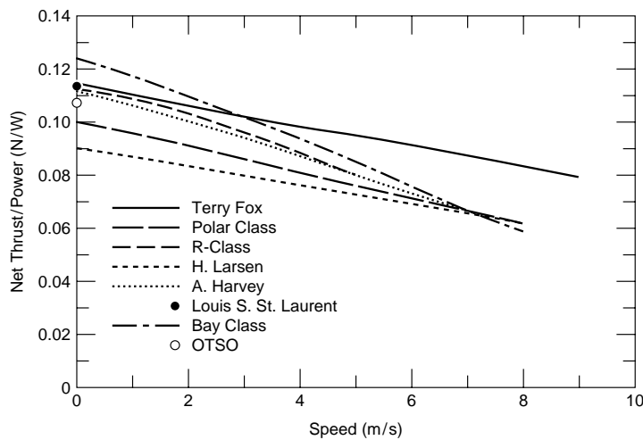
Figure 24. Specific net thrust vs. speed at maximum shaft power, indicating propulsive performance (after Keinonen et al. 1991).
