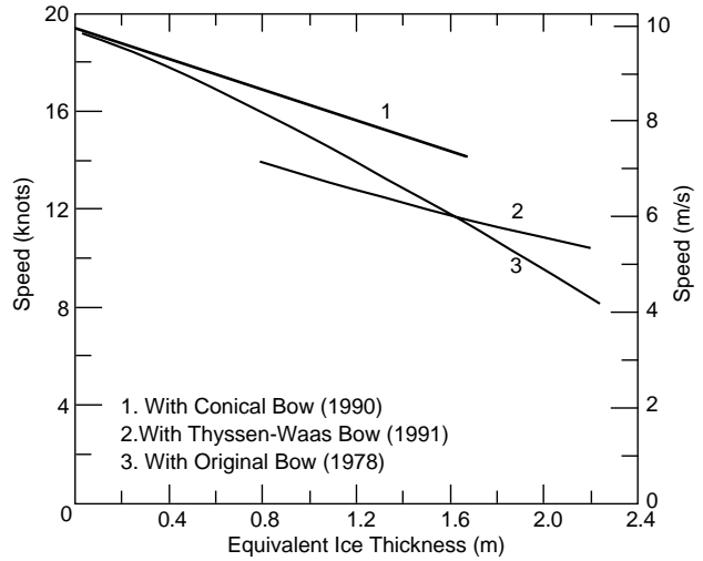
Figure 11. Ship speed vs. equivalent ice thickness during tests in broken ice with three sister ships having different bow shapes. The ships were tested in their own channels (after Ierusalimsky and Tsoy 1994).
