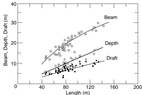
a. Icebreakers (cargo ships not included) (after Dick and Laframboise 1989).
