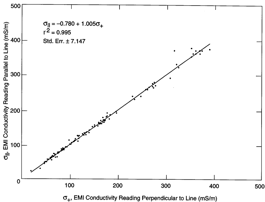
Figure 5. EMI conductivity reading vs. instrument boom orientation (parallel vs. perpendicular) to the survey line.
