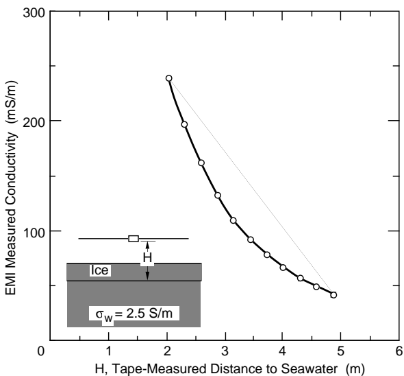
Figure 2. EMI-determined conductivity vs. instrument height above the seawater (from Kovacs and Morey 1992) \sigma_w = seawater conductivity.
