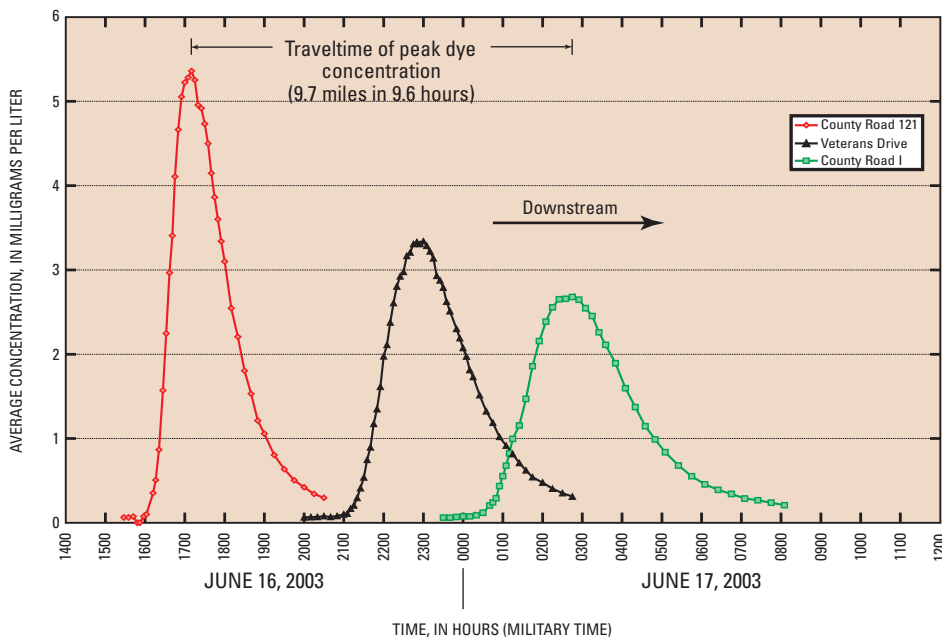
Figure 4. Measured tracer-response curve for three Sauk River locations.
