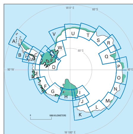
Figure 2. Index map showing the locations and names of the 23 published and planned 1:1,000,000-scale coastal-change and glaciological maps of Antarctica. The dates (2004) of published maps are shown that are available in print and digital formats. Web access to digital data is as follows: http://pubs.usgs.gov/imap/2600/G for the Saunders Coast map (I-2600-G), for example.
