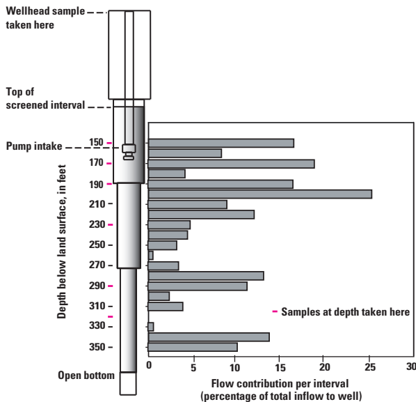
Inflow at different depths within a public-supply well. The aerial photo shows an approximately 63-square-mile area near the well. Water entering the well screen is associated with different potential sources of contaminants because of the different land-use activities in the areas contributing recharge to various intervals along the well screen, as well as the different aquifer materials through which water flows between the recharge areas and the well. The amount of contamination that might be contributed by any given interval is related to the volume of water that flows into the well along the interval and the concentration of any associated contaminants. Depth-dependent samples are a composite of all intervals beneath the sampling point; these samples are being analyzed for chemical quality and ground-water age and then compared to samples collected from the wellhead.
