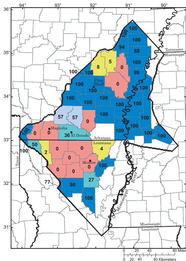
Percentage of 1990-97 withdrawal from Sparta aquifer that is sustainable by county (Sparta model).
