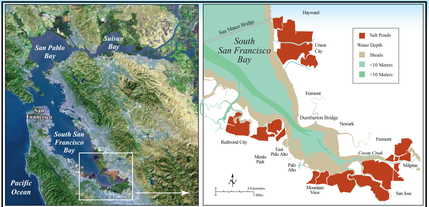
Satellite image of San Francisco Bay and inset map showing the location of salt ponds that are the focus of the restoration.
