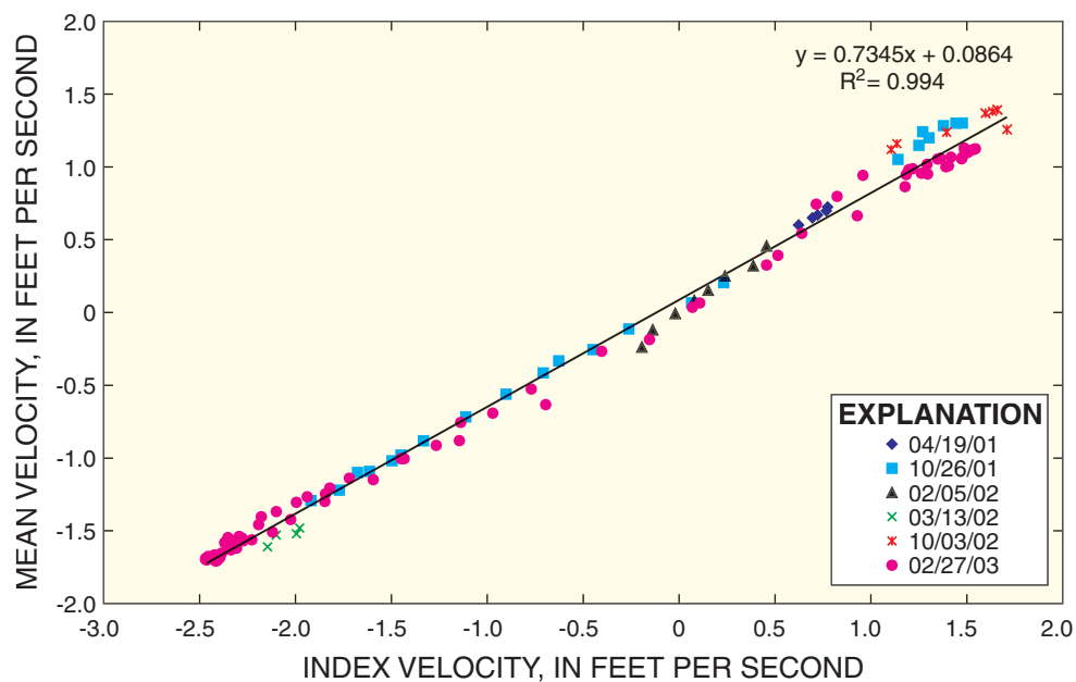
Figure 4. Velocity index rating for Chatham River (located north of Lostmans River).
