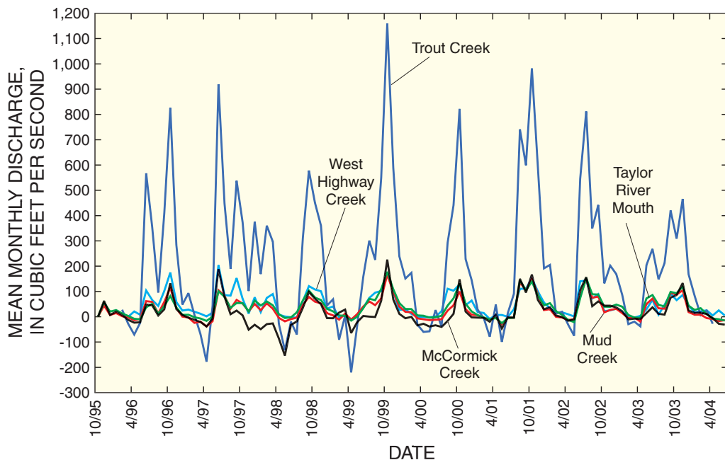
Figure 6. Mean monthly values of discharge in northeastern Florida Bay. Positive values indicate flow into Florida Bay.
