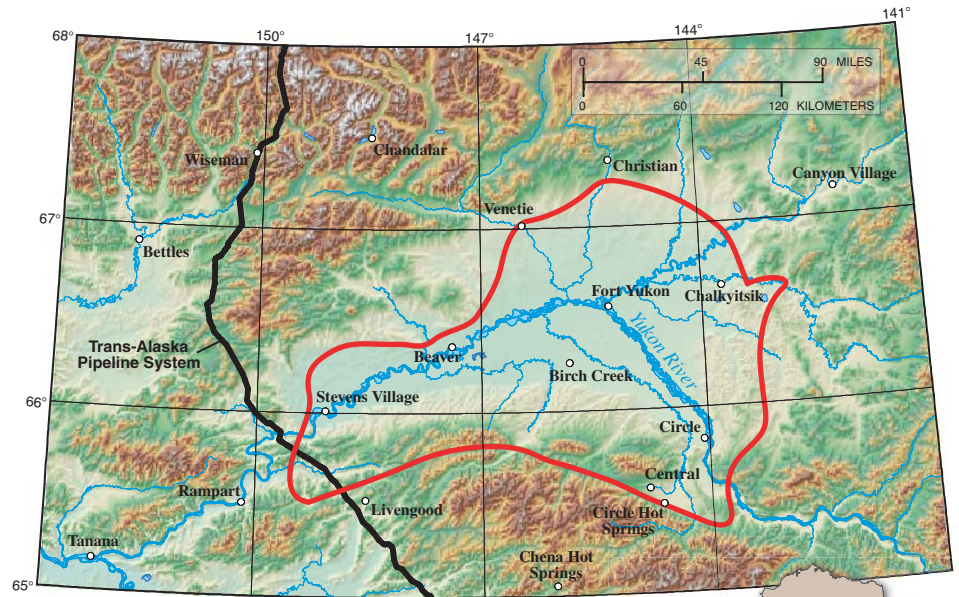
U.S. Geological Survey scientists recently finished their first detailed assessment of the undiscovered oil and gas potential of the Yukon Flats Tertiary Composite Total Petroleum System (red outline) of east-central Alaska. The assessment indicates the probable existence of technically recoverable oil and gas resources.
