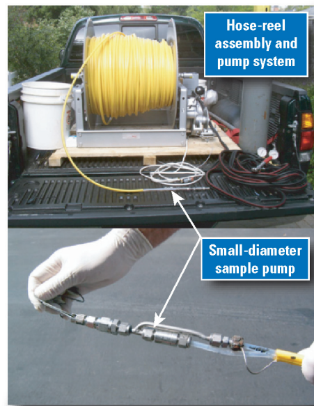
Figure 2. Photograph showing a) hose-reel assembly and b) small-diameter sample pump.
