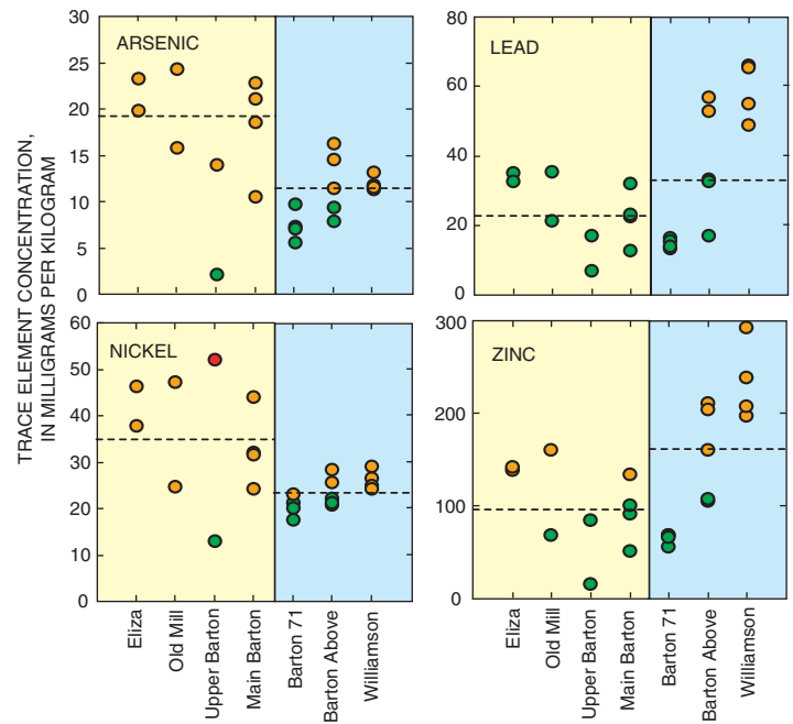
Figure 4. Concentrations of selected metals in suspended sediments discharging from springs (yellow background) and in surface streams (blue background) are compared. Only for lead and zinc, two metals with a strong urban source signal (Callender and Rice, 2000), were the median concentrations higher in surface-water sediments than in spring sediments. Relative magnitude of concentrations was compared to sediment-quality guidelines (MacDonald and others, 2000), as indicated by symbol color.
