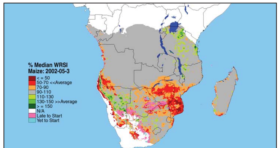
Figure 6. Crop water balance calculations, derived from remotely sensed data, are used to map the extent and severity of drought in Africa. This type of geographic analysis guides ground data collection to determine the number of people affected and the scope of the required response by the international community. This image shows Southern Africa in 2002, where 1.2 million metric tons of food aid are needed by over 12 million people in 6 countries. (Red, pink, and white areas are the most seriously affected.)
