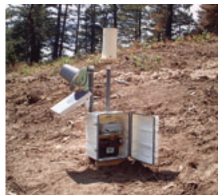
A. Precipitation gage (instrument detail) used in burned area at Missionary Ridge Complex Fire.
