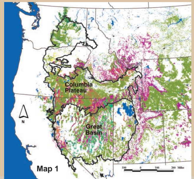
Sagebrush Landcover Types
