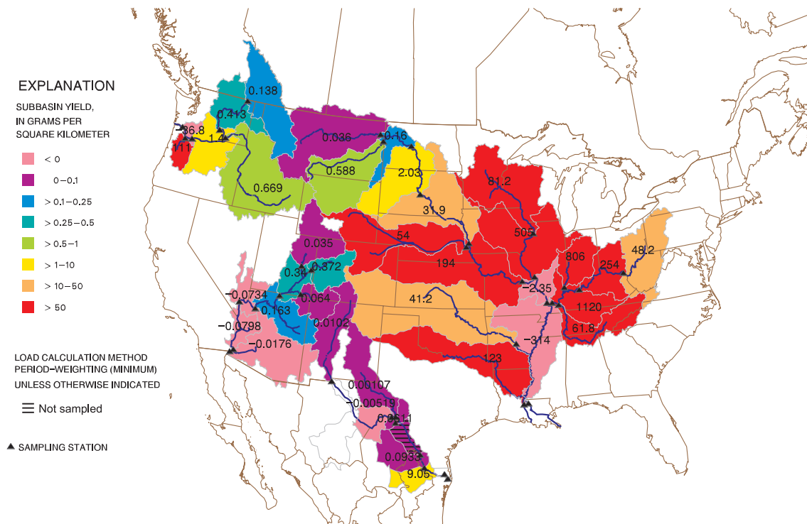
Figure 2. Atrazine yield from National Stream Quality Accounting Network (NASQAN) subbasins, 1997–2000.
