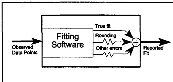
Figure 4 The forward error analysis model. The other errors include bias and sensitivity.
