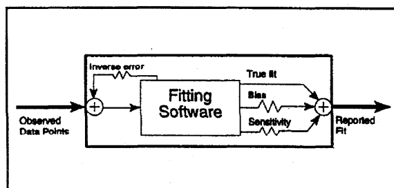
Figure 5 The inverse error analysis model.
