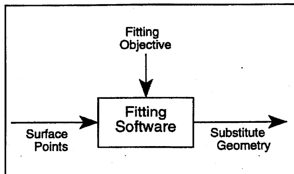
Figure 2 Ideal model of fitting.
