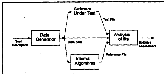
Figure 6 Architecture of the NIST Algorithm Testing System.
