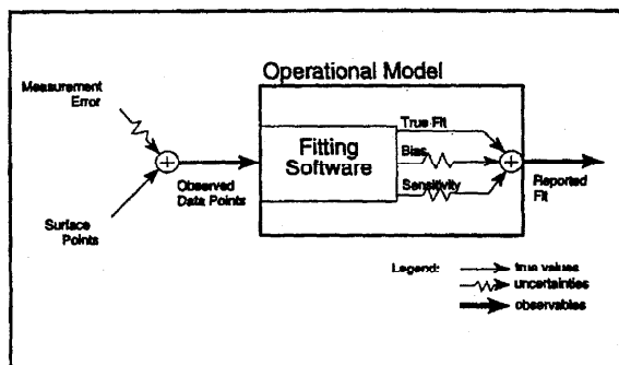
Figure 3 Operational model of fitting software, showing bias and sensitivity errors.
