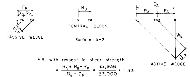
VECTOR DIAGRAM (Method of planes)
