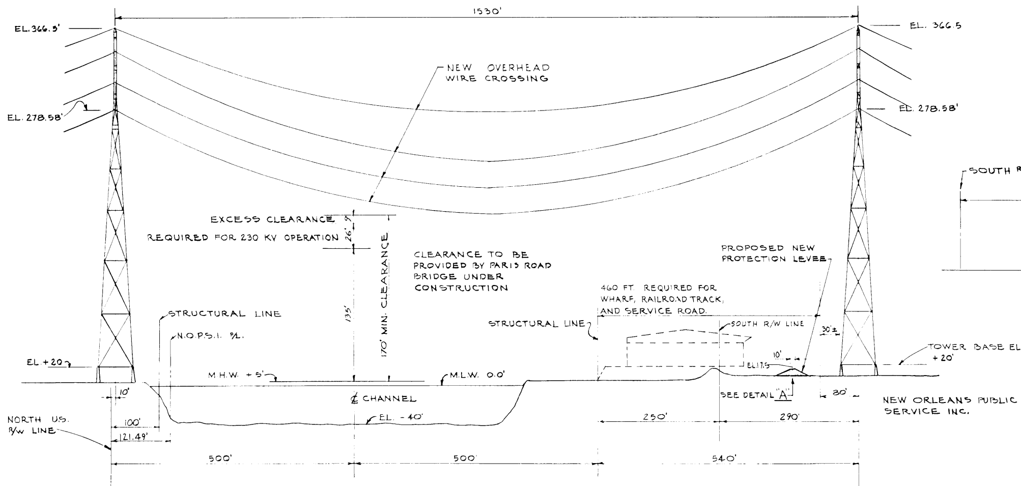
SECTION 11/A HOR. SCALE "c" VERT. SCALE "a"
