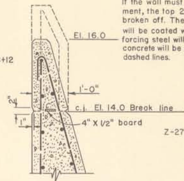
DETAIL FOR RAISING WALL (Sta. 67+94 to 79+62)
