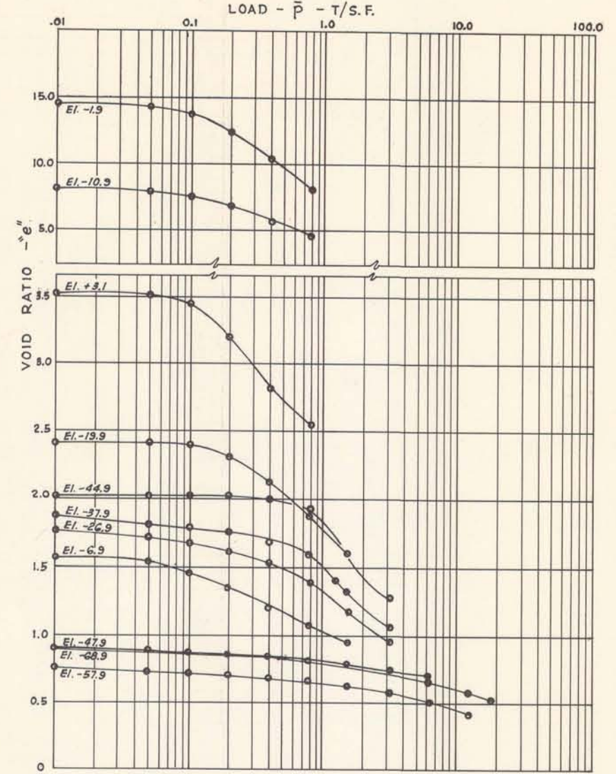
CONSOLIDATION DATA
