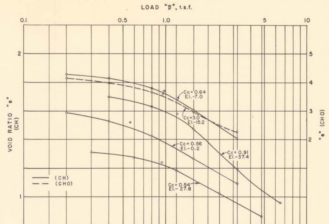
CONSOLIDATION DATA
