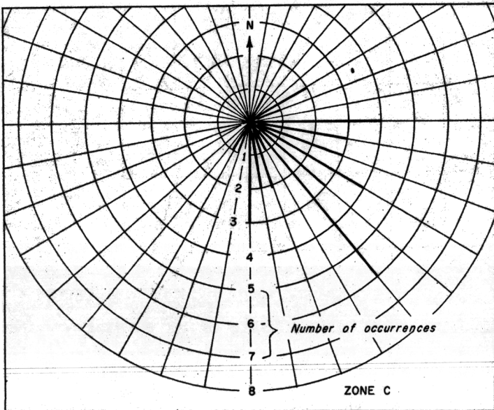
Figure 21. - Azimuth distribution of hurricane paths in zone, Gulf Coast, 1900-1956.
