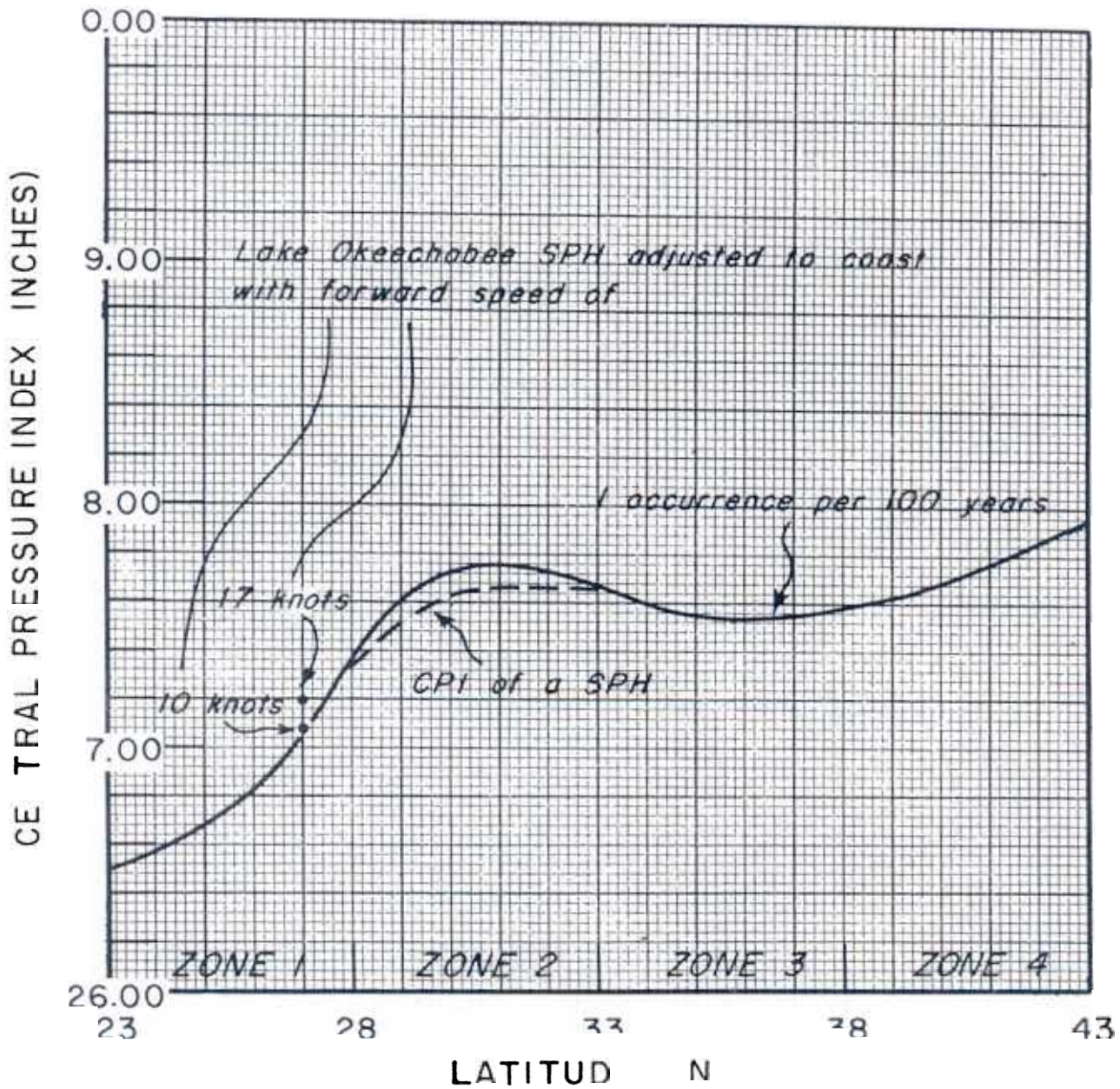
Figure 5a. Latitudinal variation of central pressure index CPI for standard project hurricane
