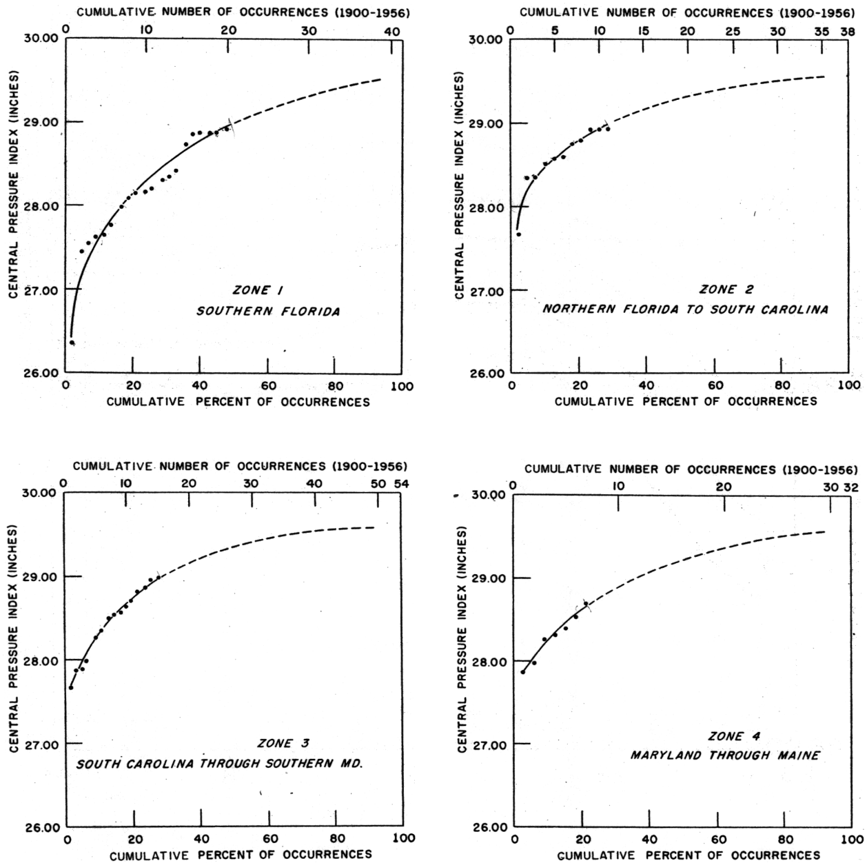
Figure 2. - Cumulative frequencies of hurricane central pressure index, Atlantic Coast United States, 1900-1956.
