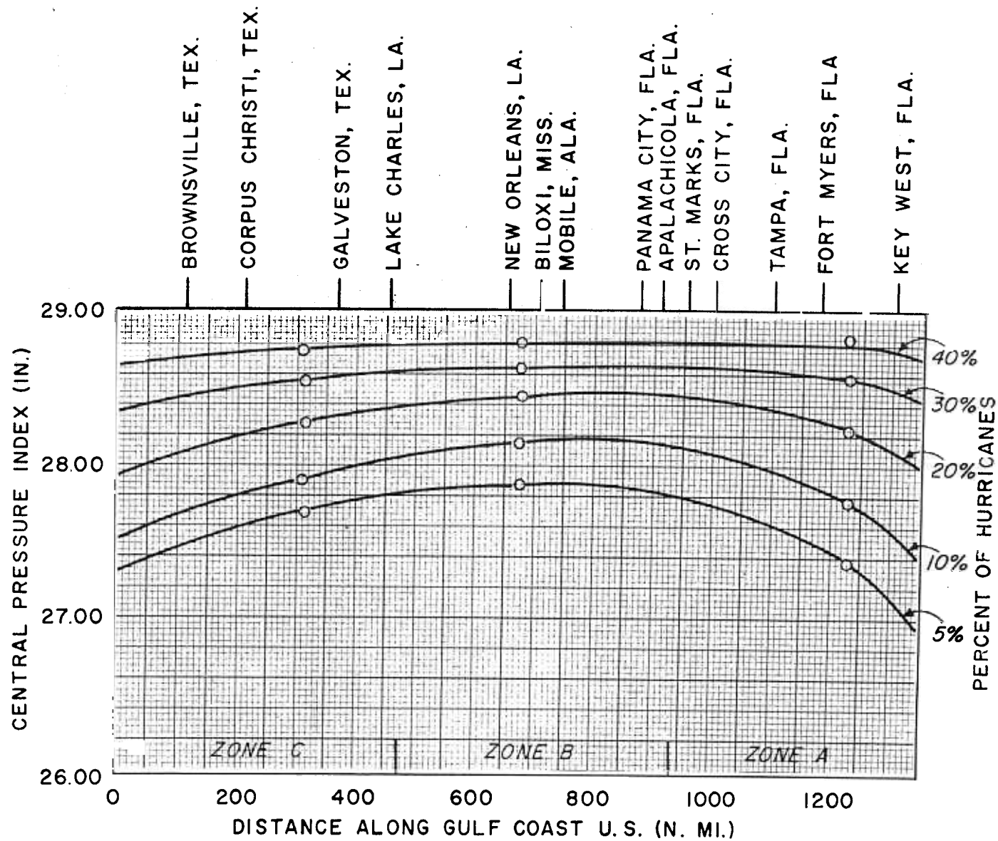
Figure 13. - Geographic variation of cumulative frequency of hurricane central pressure index, Gulf Coast (1900-1956) over zones A, B, and C of approximately 80,000 square miles.
