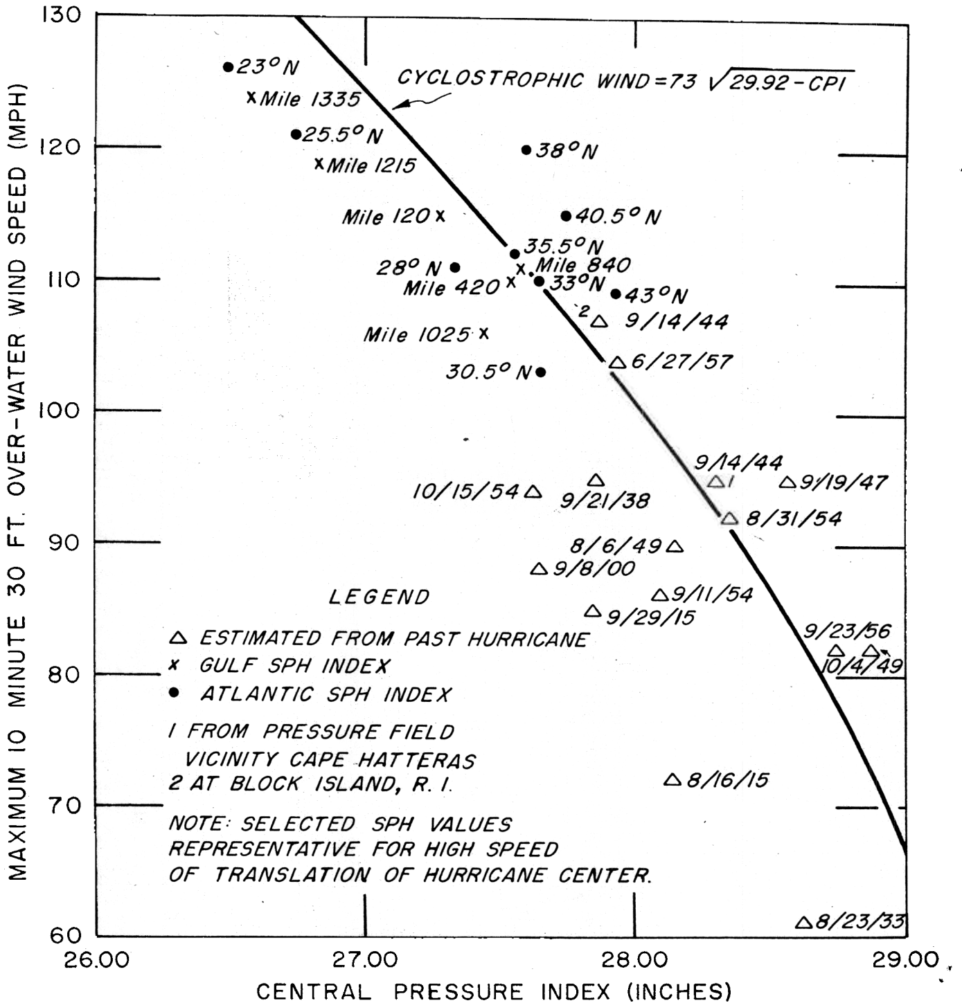
Figure 48. - Relation of central pressure index to maximum 30-ft. wind, Atlantic and Gulf Coasts.
