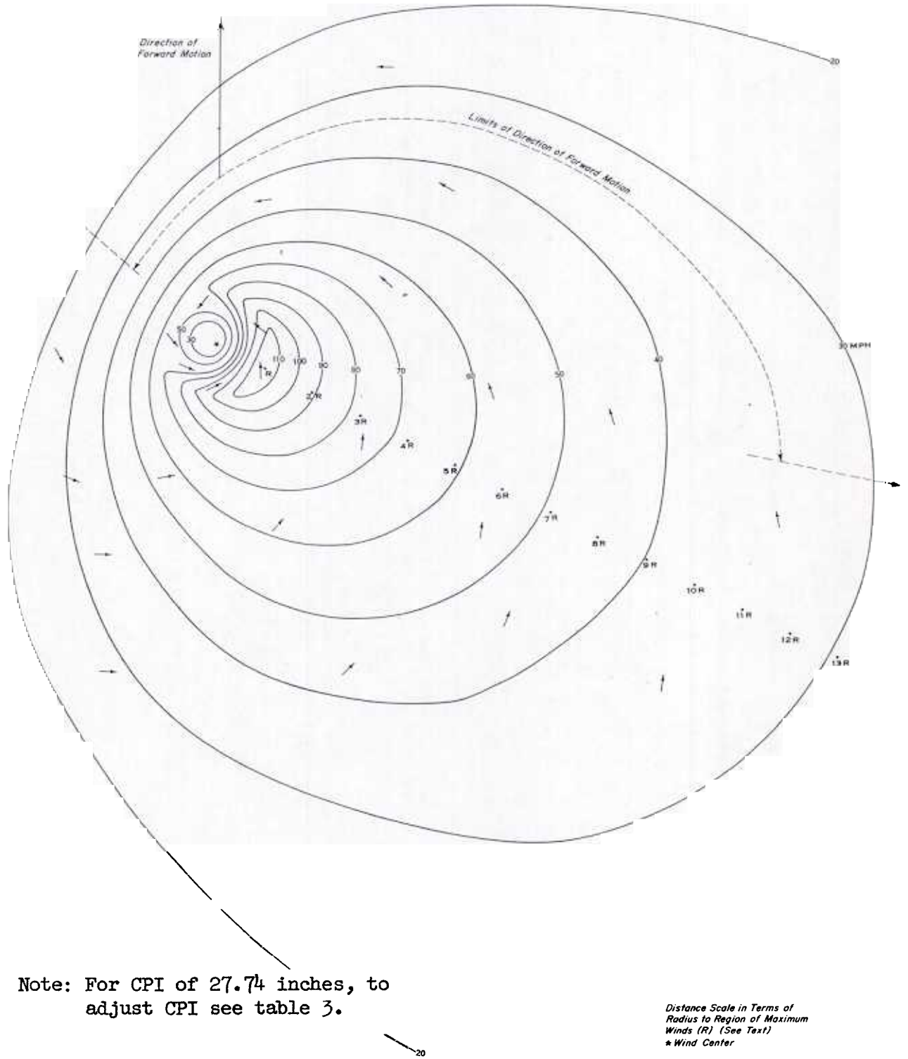
Figure 36. - Standard Project Hurricane 30-ft. over-water isovel pattern.
