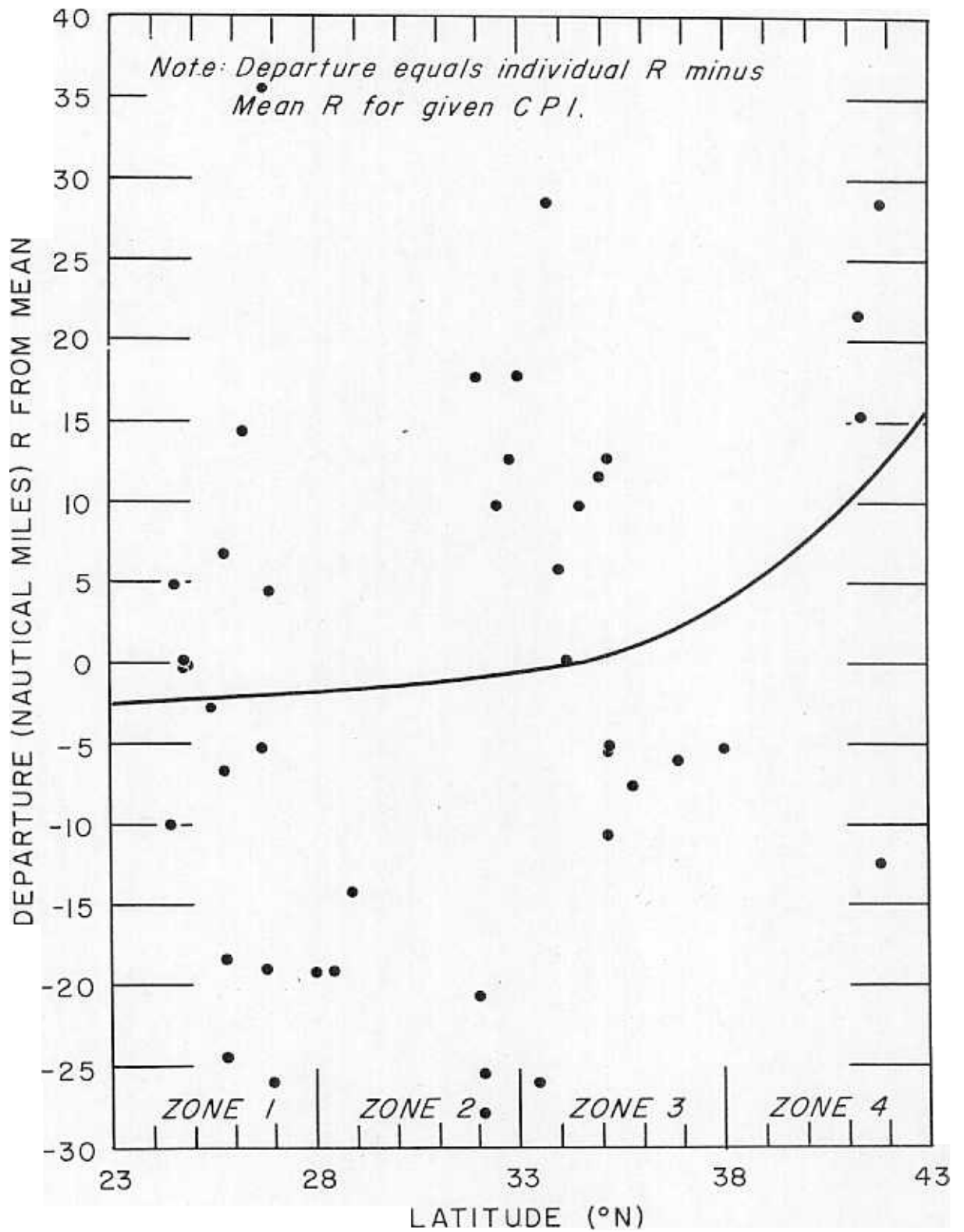
Figure 8. - Variation with latitude of departures of points in figure 7 from mean curve.
