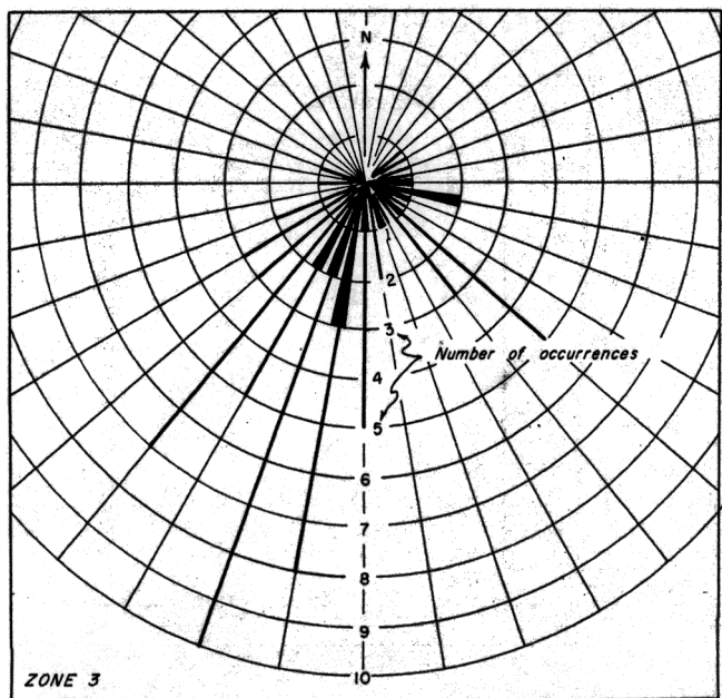
Figure 10. - Azimuth distribution of paths followed by hurricanes, 1887-1956.
