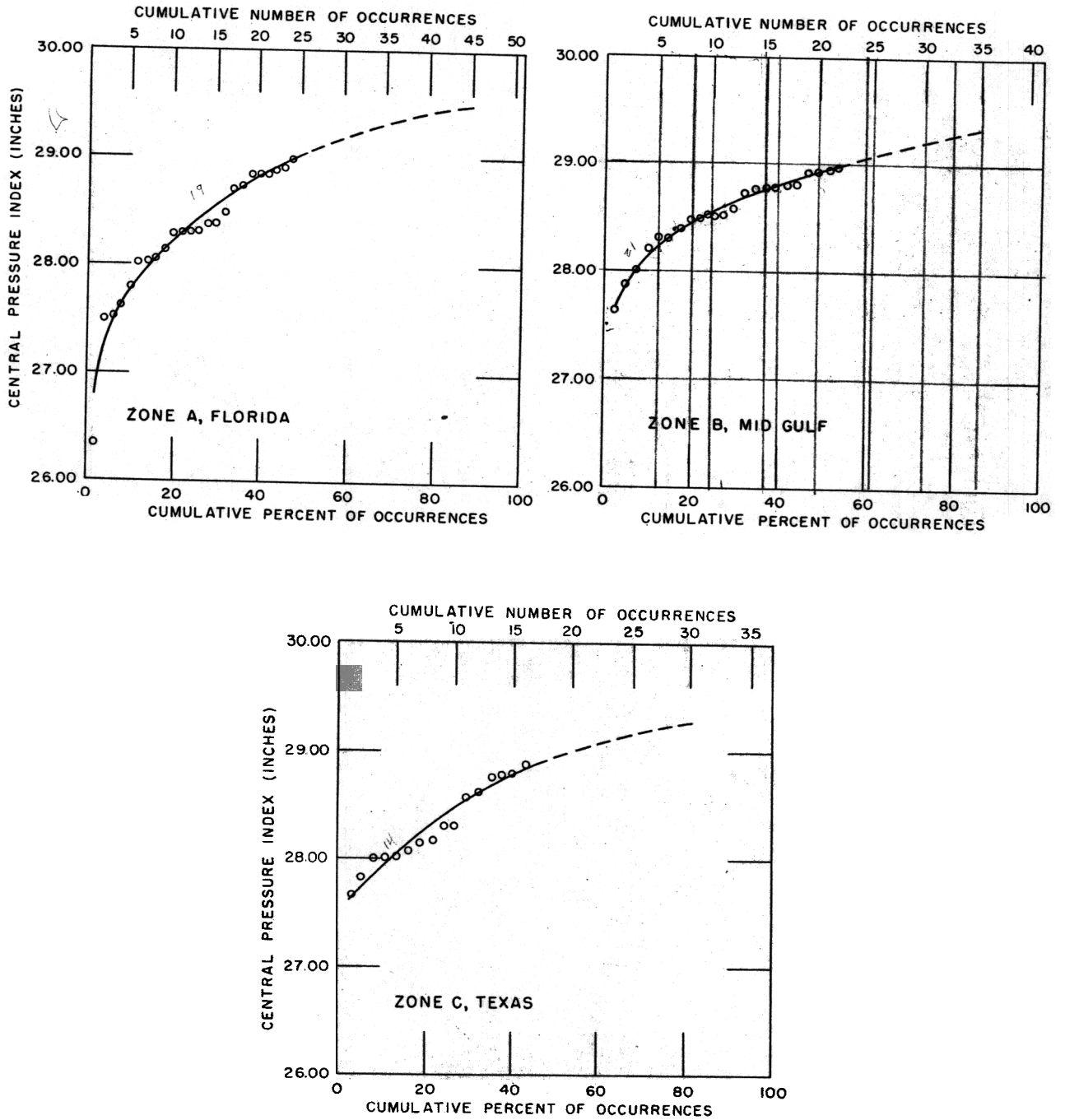
Figure 12. - Cumulative frequency of hurricane central pressure index, Gulf Coast United States (1900-1956).
