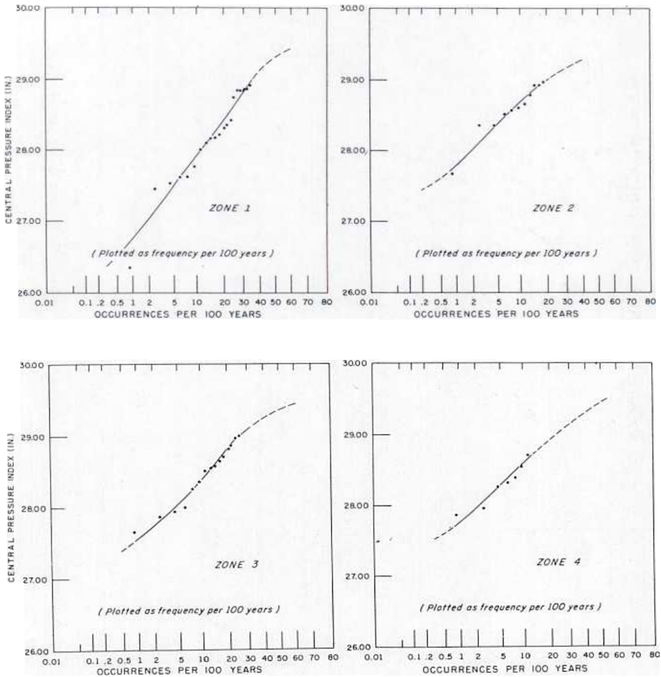
Figure 4. - Cumulative frequencies of hurricane central pressure index, 1900-1956, (plotted as frequency per 100 years).
