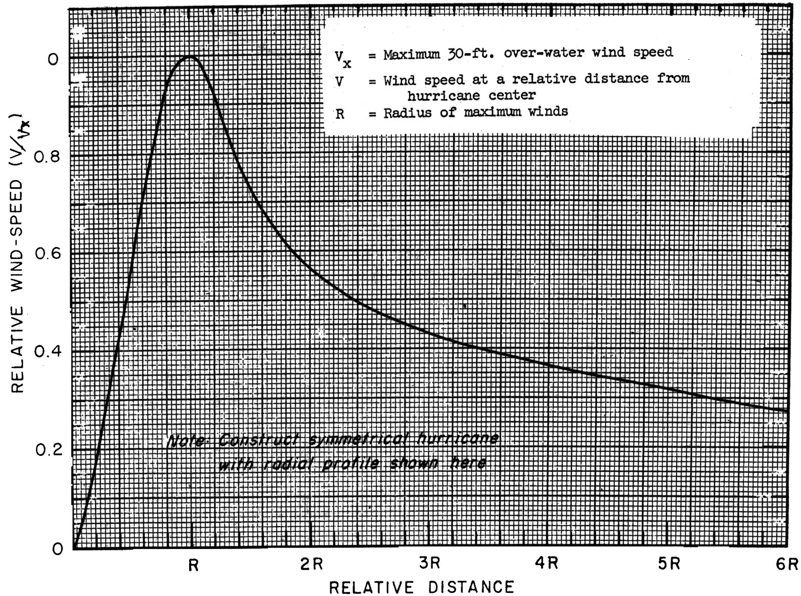
Figure 47. Standard Project Hurricane 30-ft. wind-speed profile, small radius (RS) hurricanes, all zones. 67
