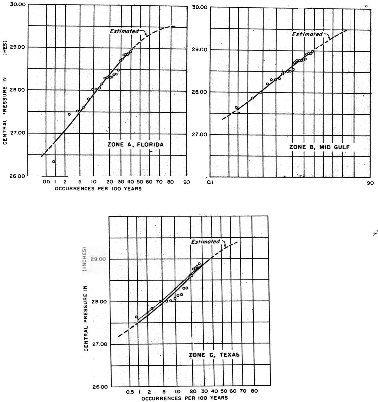
Figure 14. - Cumulative frequency of hurricane central pressure index (1900-1956)
