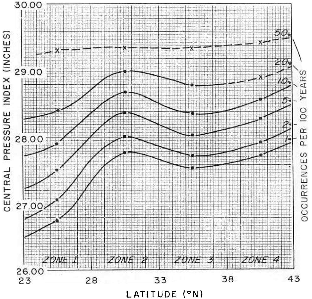
Figure 5. - Latitudinal variation of average frequency per 100 years of hurricane central pressure index, east coast United States (1900-1956) over zones of approximately 60,000 square miles.
