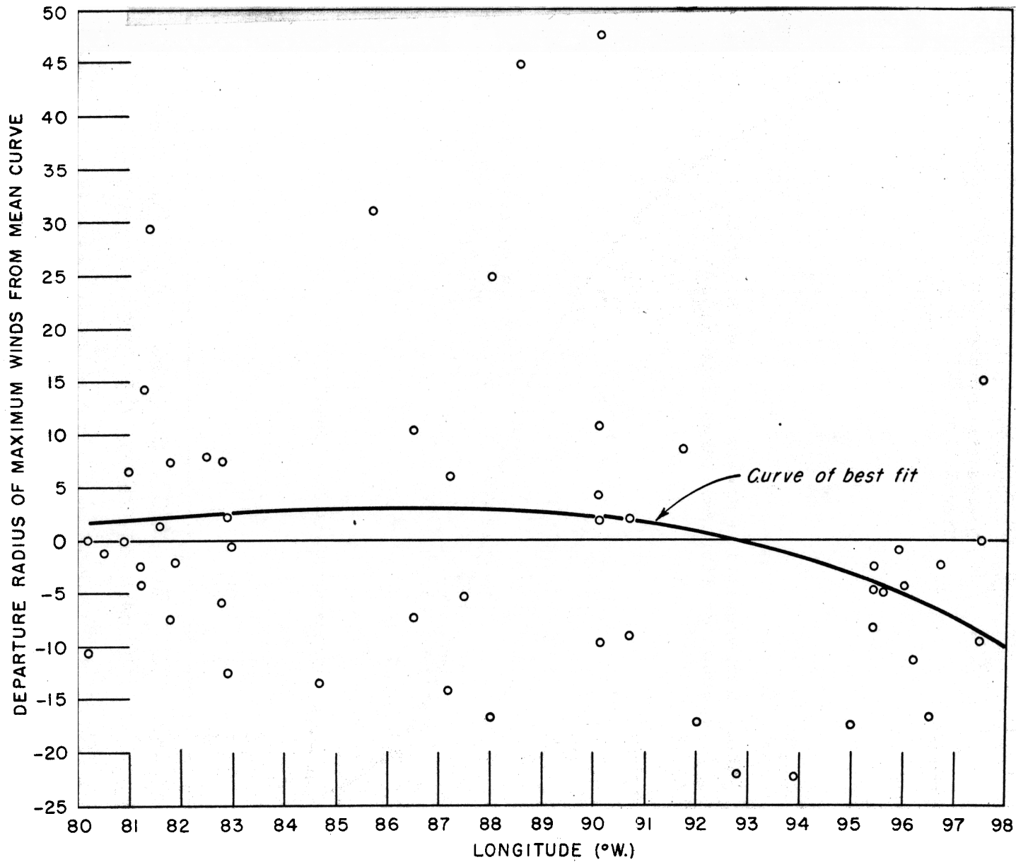
Figure 19. - Variation with longitude of departure of radius of maximum winds from mean curve of figure 17. 69
