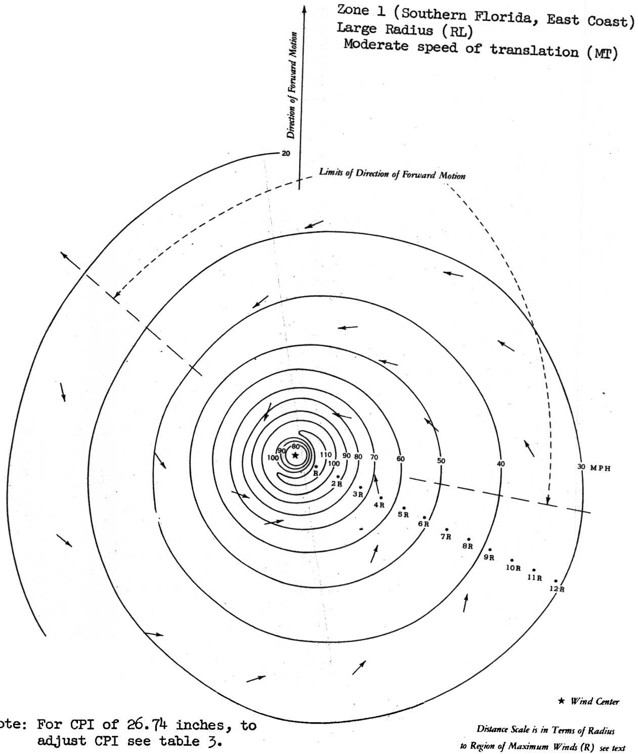
Figure 25. - Standard Project Hurricane 30-ft. over-water isovel pattern.
