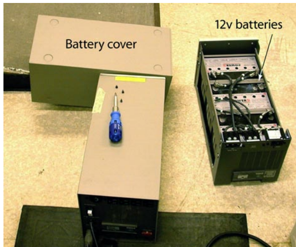
Figure 2-1. Topaz Powermaker Micro UPS
