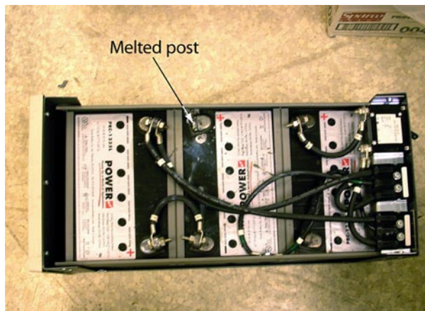
Figure 2-2. Controller unit with batteries
