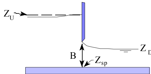
Figure 8-7 Example Sluice Gate with Broad Crested Spillway
