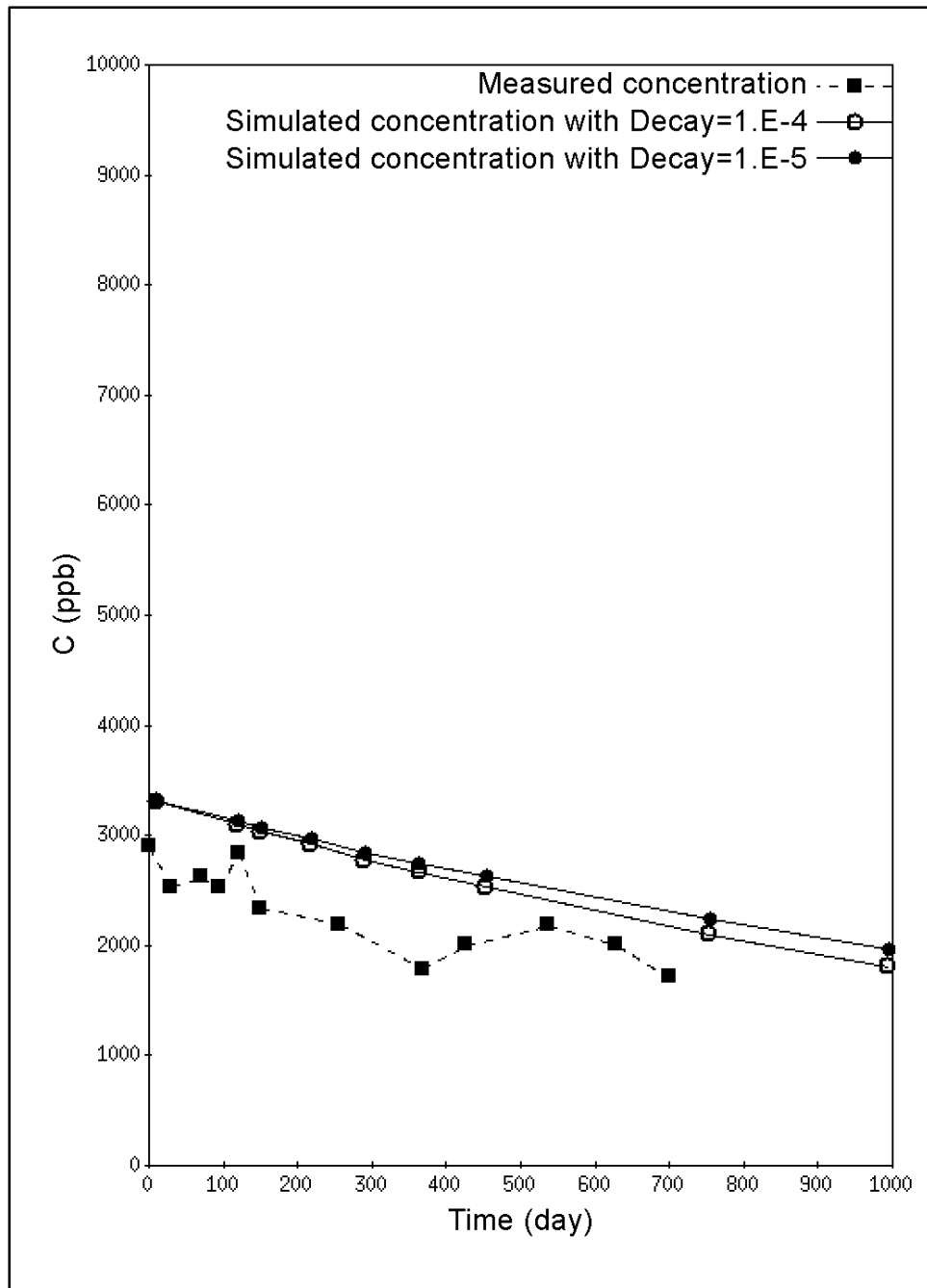
Figure 14. Time series of TNT concentration for measured and calibrated model with different first-order decay rates (1.E-4 and 1.E-5 1/day) and fixed adsorption coefficient of 2.3E-1 \text{ L kg}^{-1} as shown above (Original data were from MW083U)
