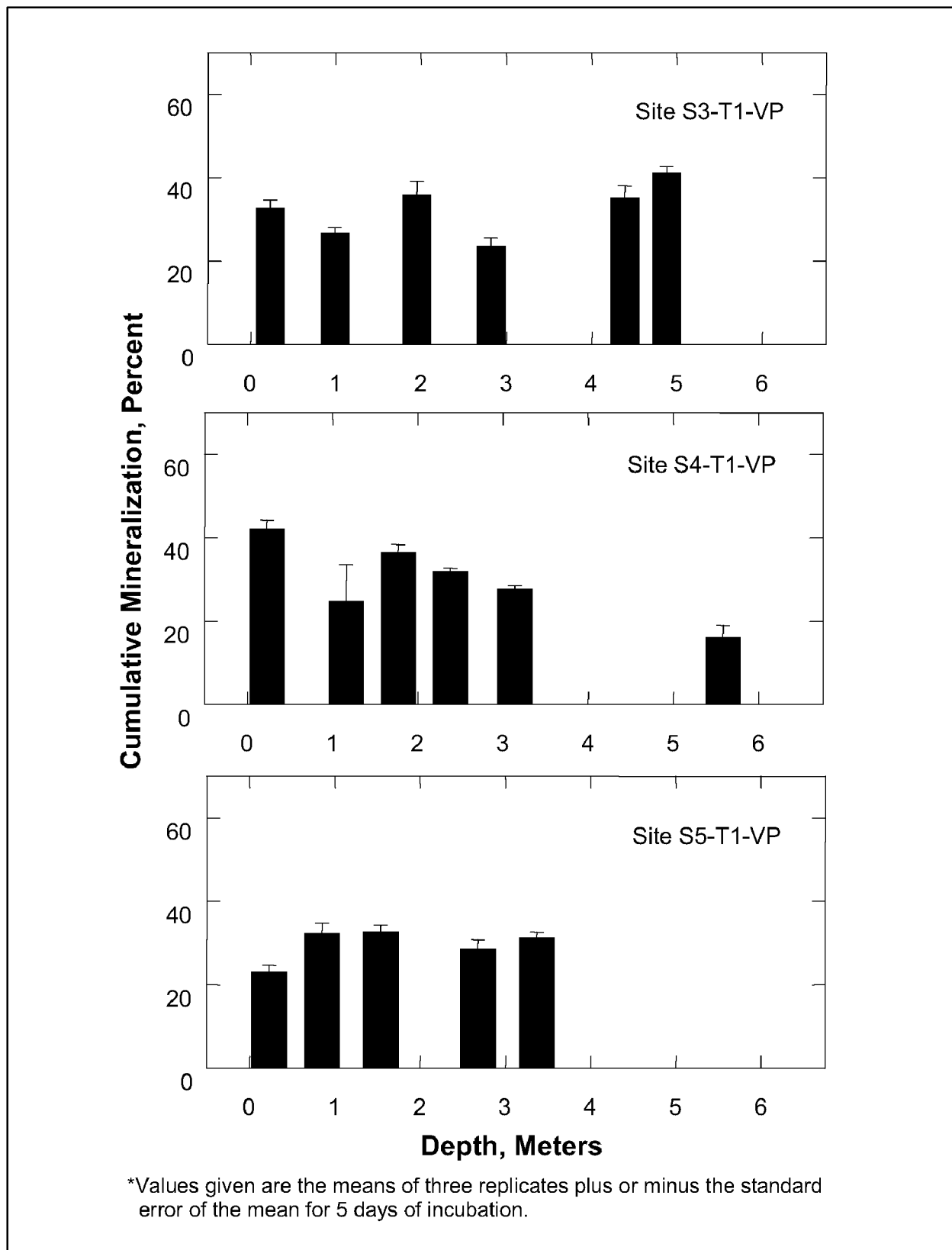
Figure 9. Acetate mineralization in Joliet vertical profile samples (Radiochemical purity was >99 percent)
