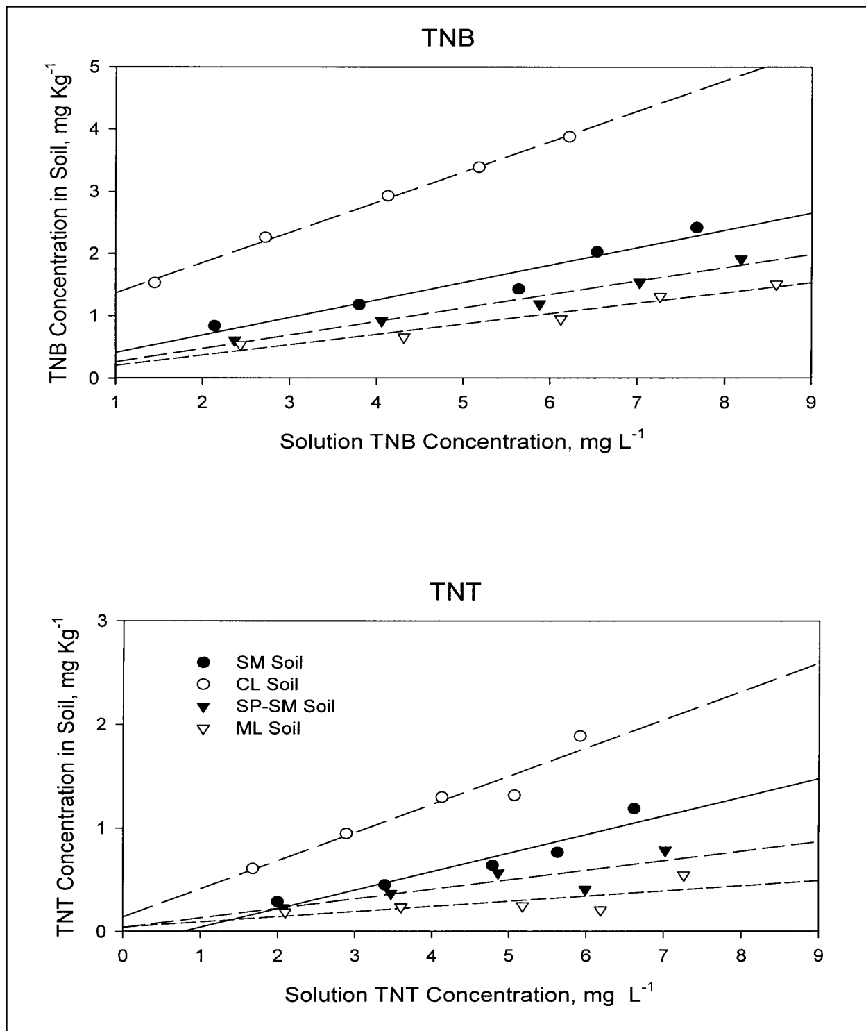
Appendix Figure 2. TNB and TNT adsorption on LAAP aquifer soils and fitted linear adsorption model
