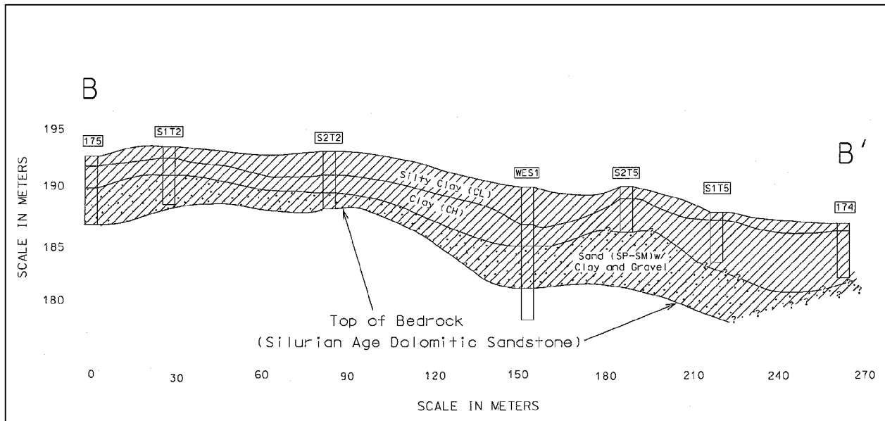
Figure 18. Geological Cross Section B-B' at JAAP
