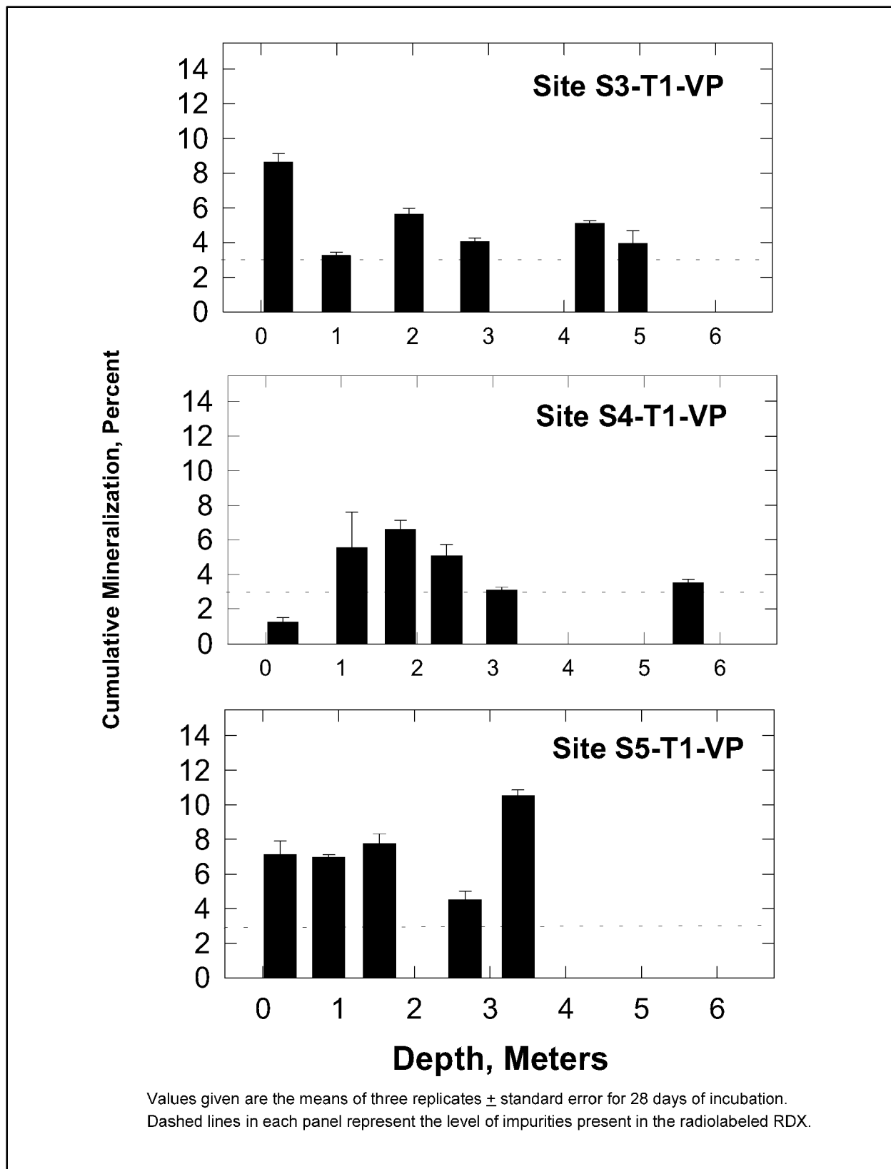
Figure 10. RDX mineralization in Joliet vertical profile samples
