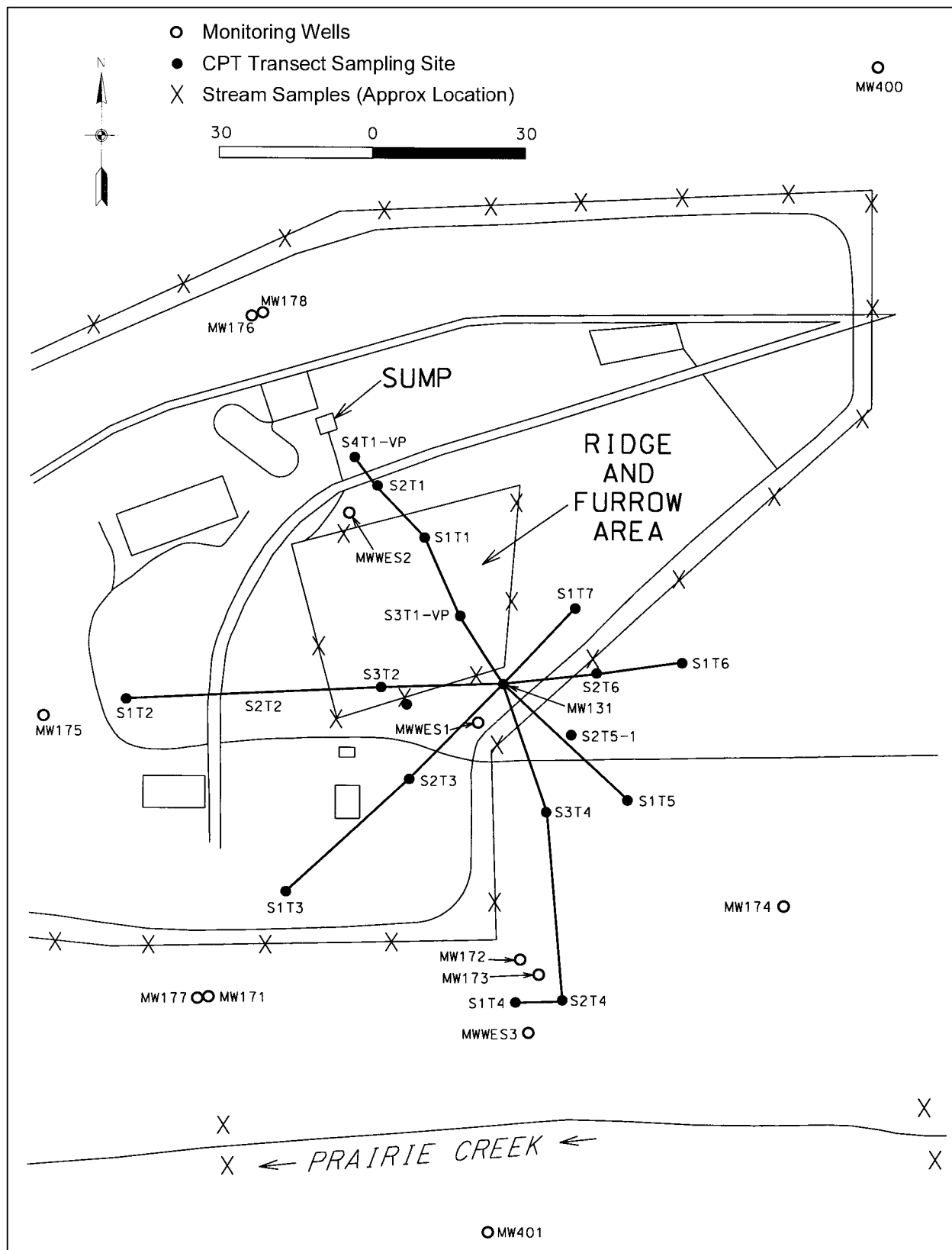
Figure 4. Locations of monitoring well and cone penetrometry sampling points at Site L1, JAAP
