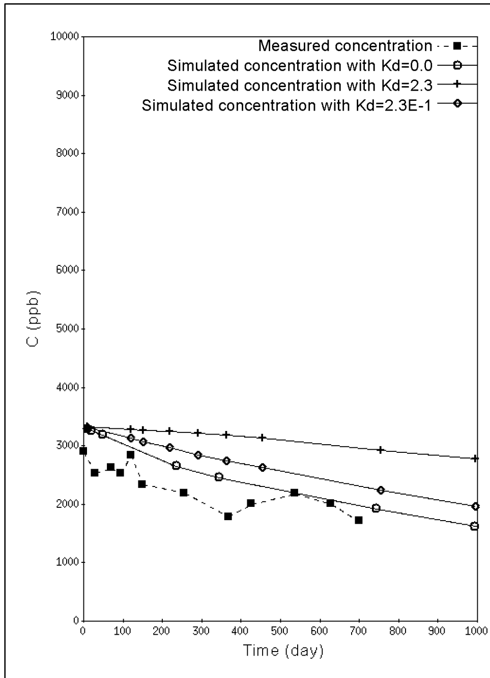
Figure 13. Time Series of TNT concentration for measured and calibrated model with different adsorption coefficients ( L\ kg^{-1} ) as shown above (Original data were from MW083U)
