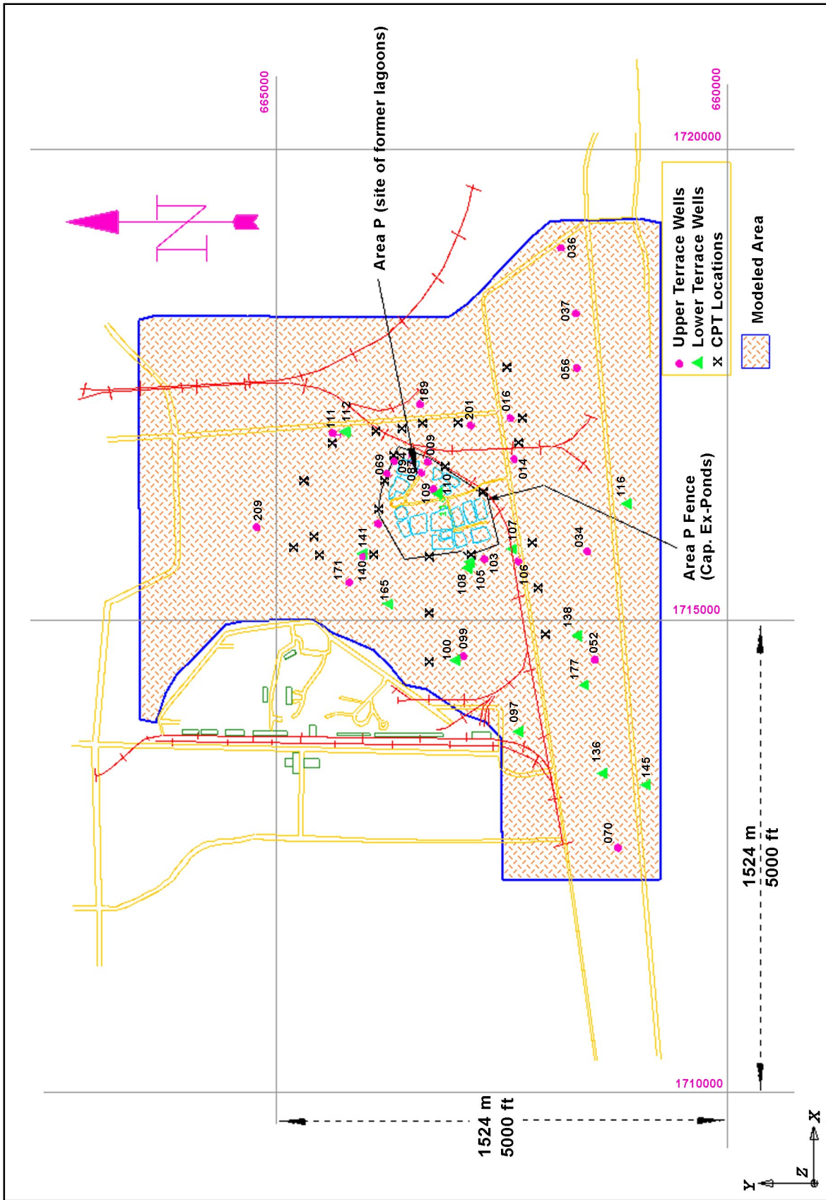
Figure 1. Modeled area at LAAP included Area P (site of former lagoons) and surrounding groundwater monitoring wells
