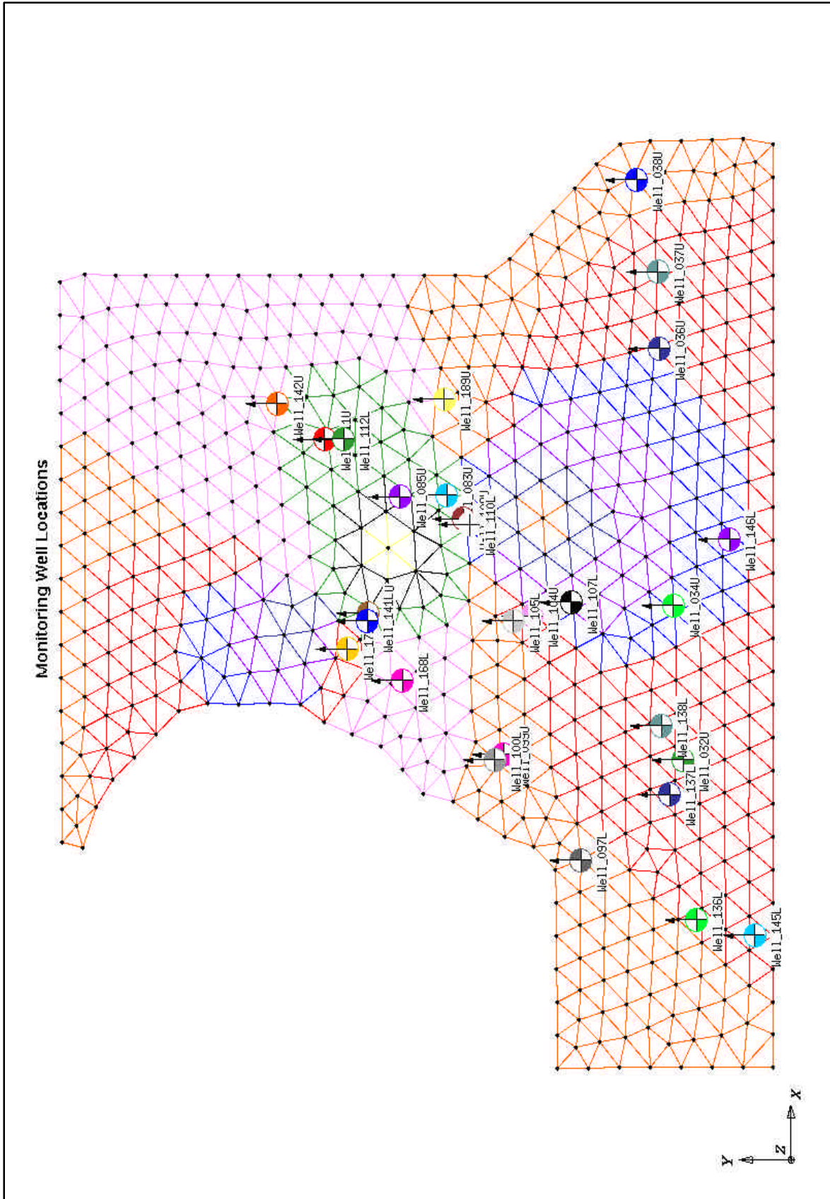
Figure 6. Locations of monitoring wells (gauges in GMS 2.0) screened in different aquifer layers
