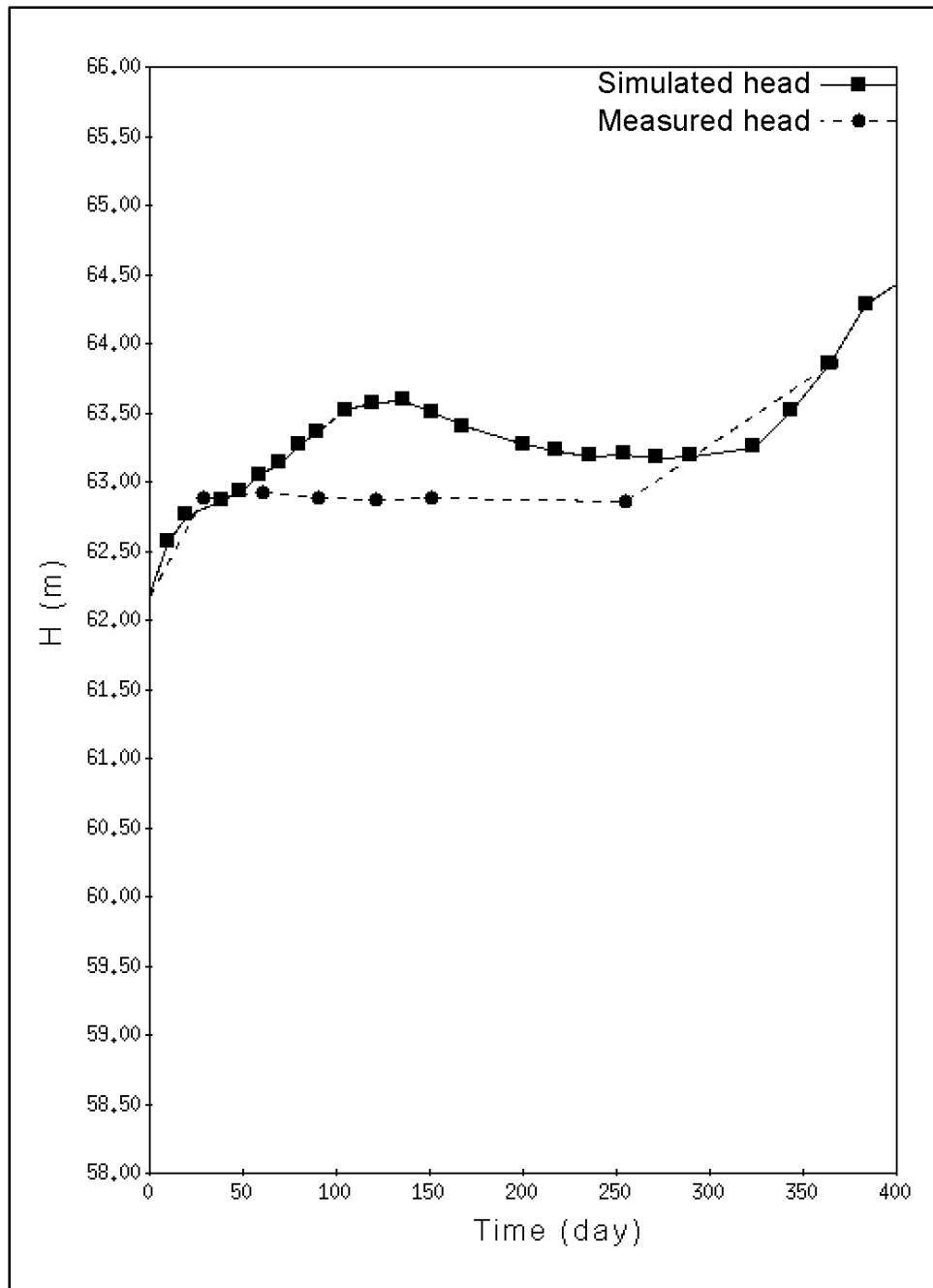
Figure 9. Comparison between measured (---●---) and simulated (---■---) head (above MSL) in MW142U screened in the upper aquifer
