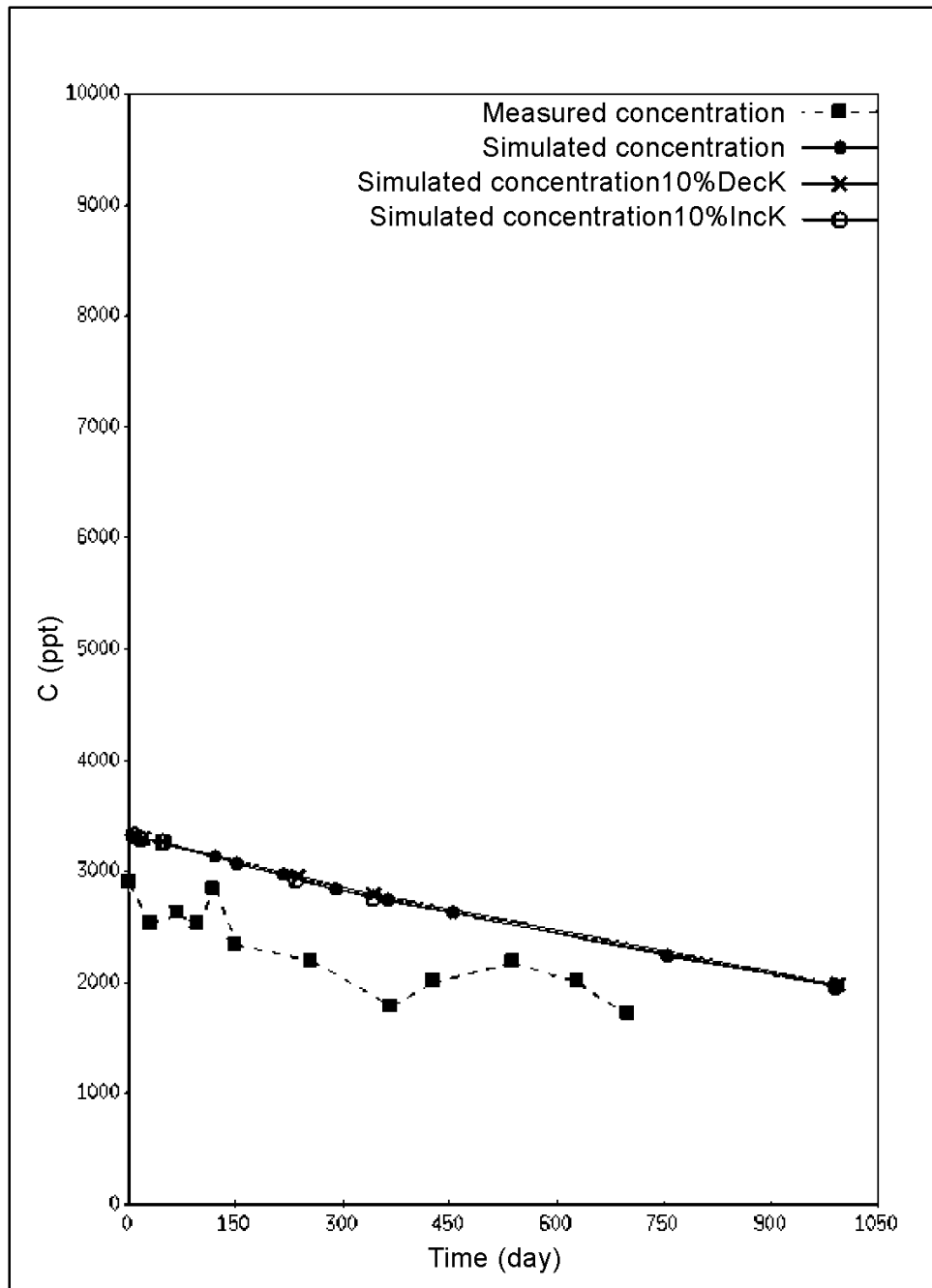
Figure 12. Time series of TNT concentration for measured calibrated model, with 10-percent increase of conductivity, and with 10-percent decrease of conductivity, respectively (Original data were from MW083U)
