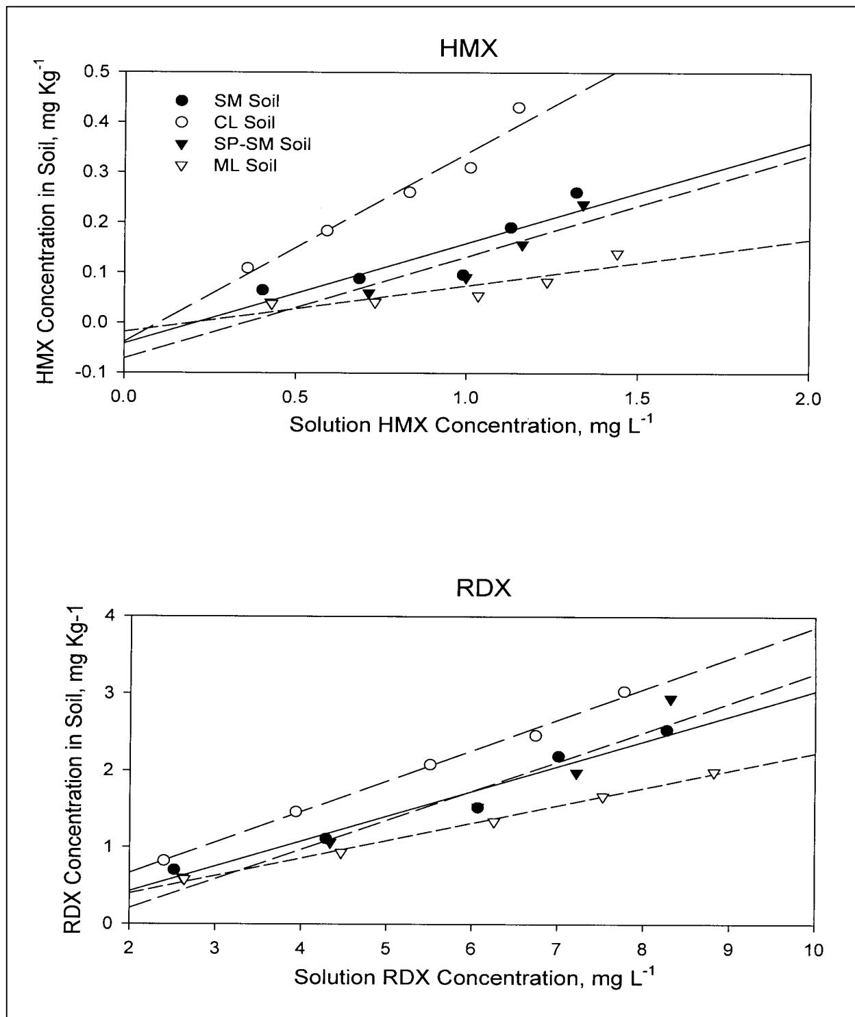
Appendix Figure 1. HMX and RDX adsorption on LAAP aquifer soils and fitted linear adsorption model
