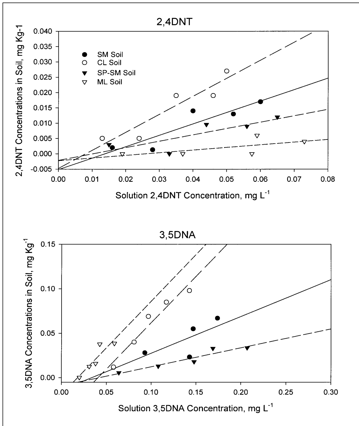
Appendix Figure 3. 2,4DNT and 3,5DNA adsorption on LAAP aquifer soils and fitted linear adsorption model
