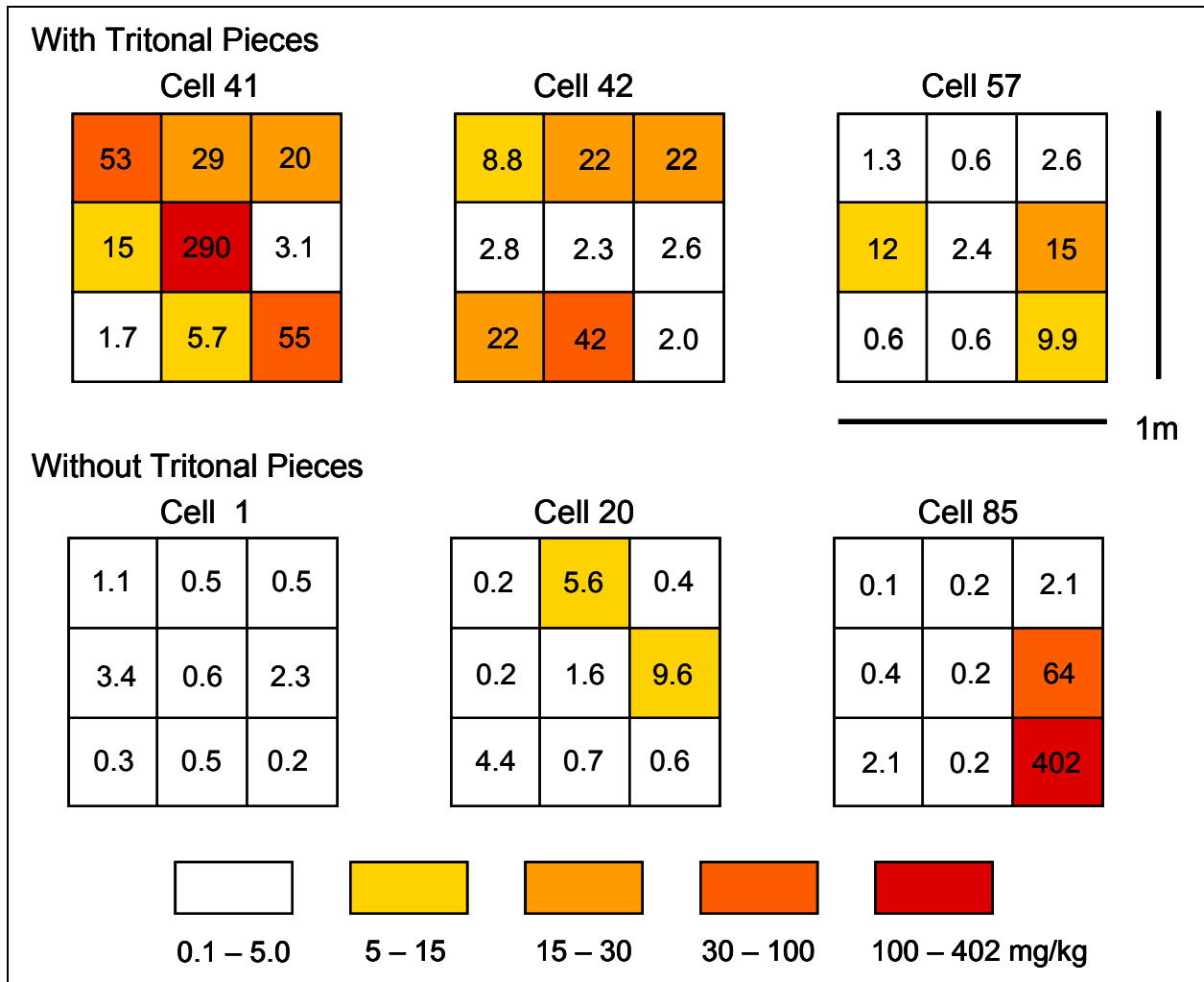
Figure 5-9. TNT concentrations (mg/kg) in nine discrete samples collected at six 1-m x 1-m cells within 10-m x 10-m Grid A (Figure 5-7) near a low-order 2,000-lb bomb. Upper three cells were collected where tritonal pieces were visible at the surface; lower three cells had no visible tritonal.
