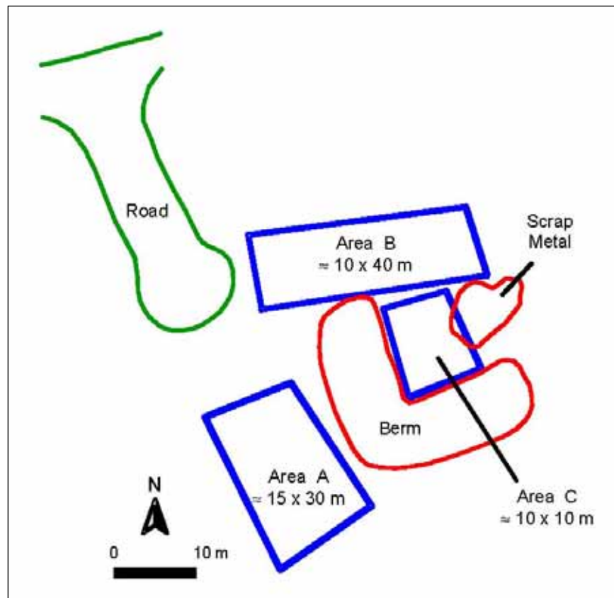
Figure 3-6. Location of sampling decision units at demolition range. Triplicate 50-increment samples were collected in Areas A to C.
