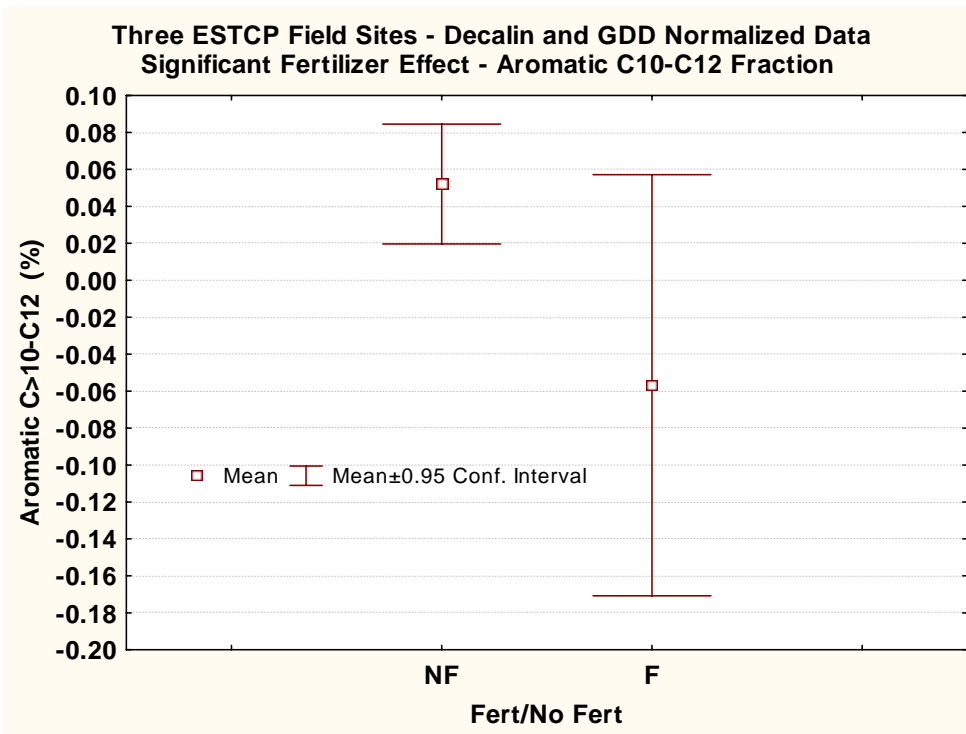
Figure 35. Three ESTCP field sites - decalin and GDD normalized data – significant fertilizer effects (inhibition) on depletion of aromatic C>10-12 fraction.
