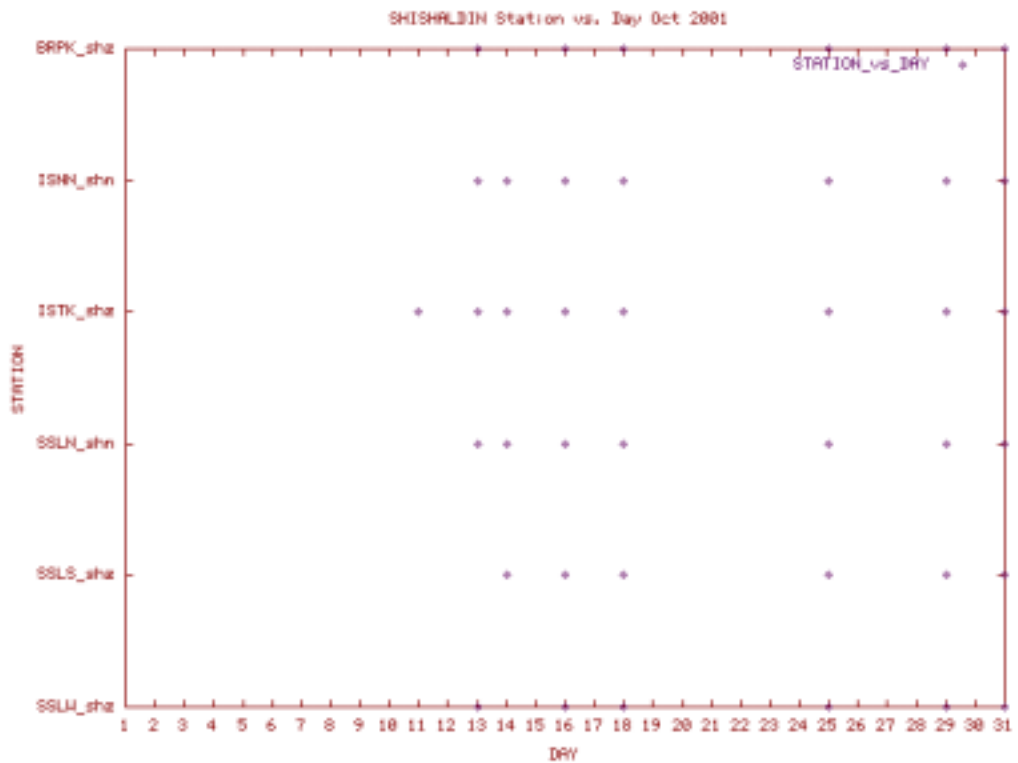
Station Use Plot for the Shishaldin subnet for October 2001
