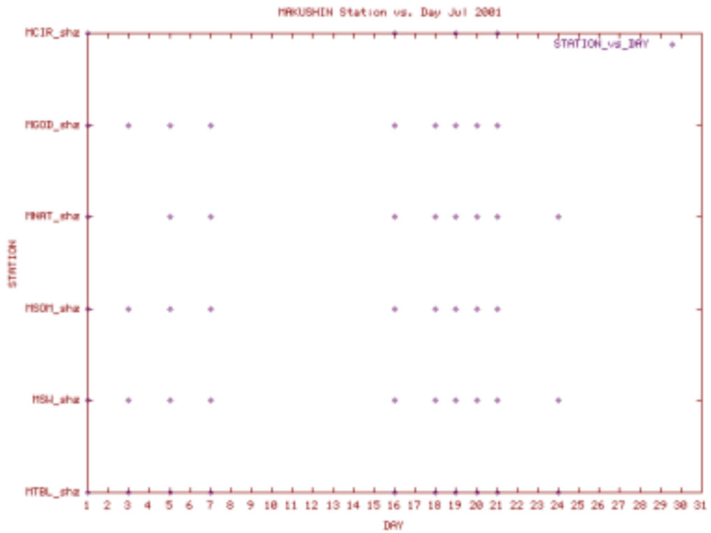
Station Use Plot for the Makushin subnet for July 2001
