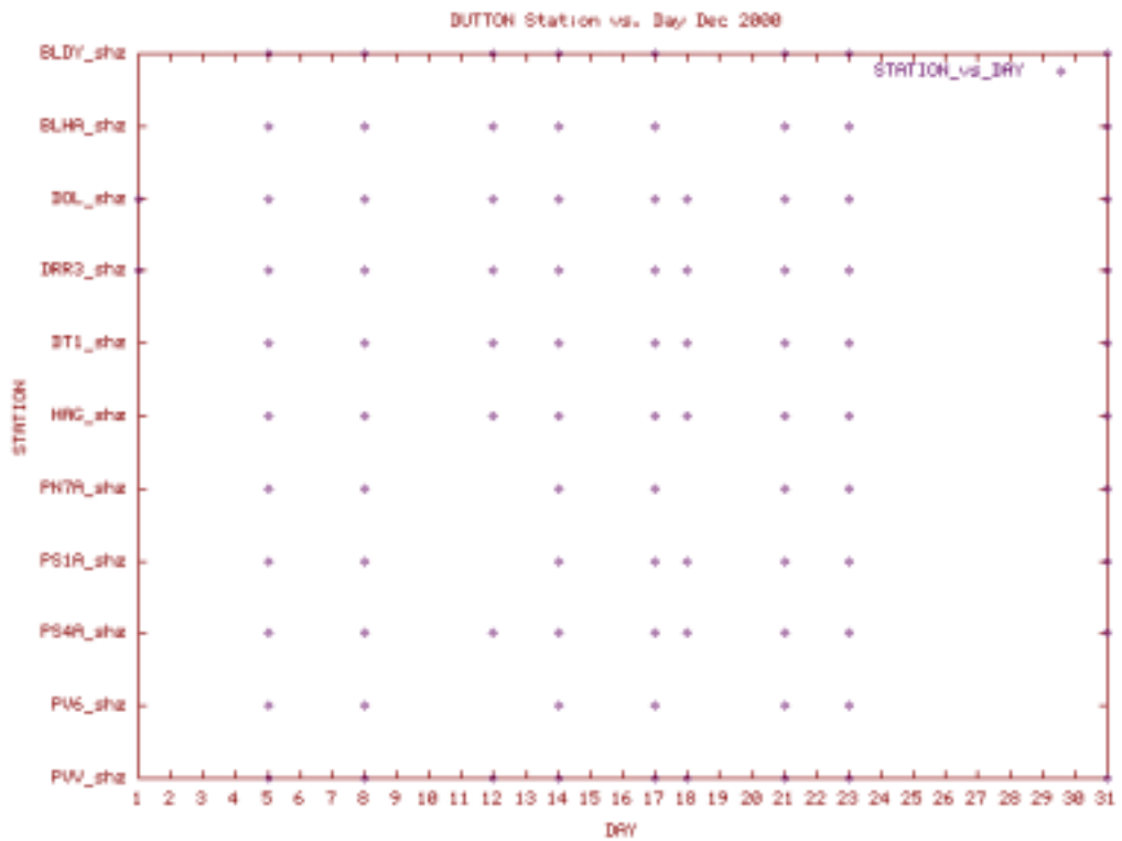
Station Use Plot for the Dutton subnet for December 2000
