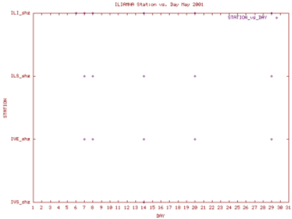
Station Use Plot for the Iliamna subnet for May 2001
