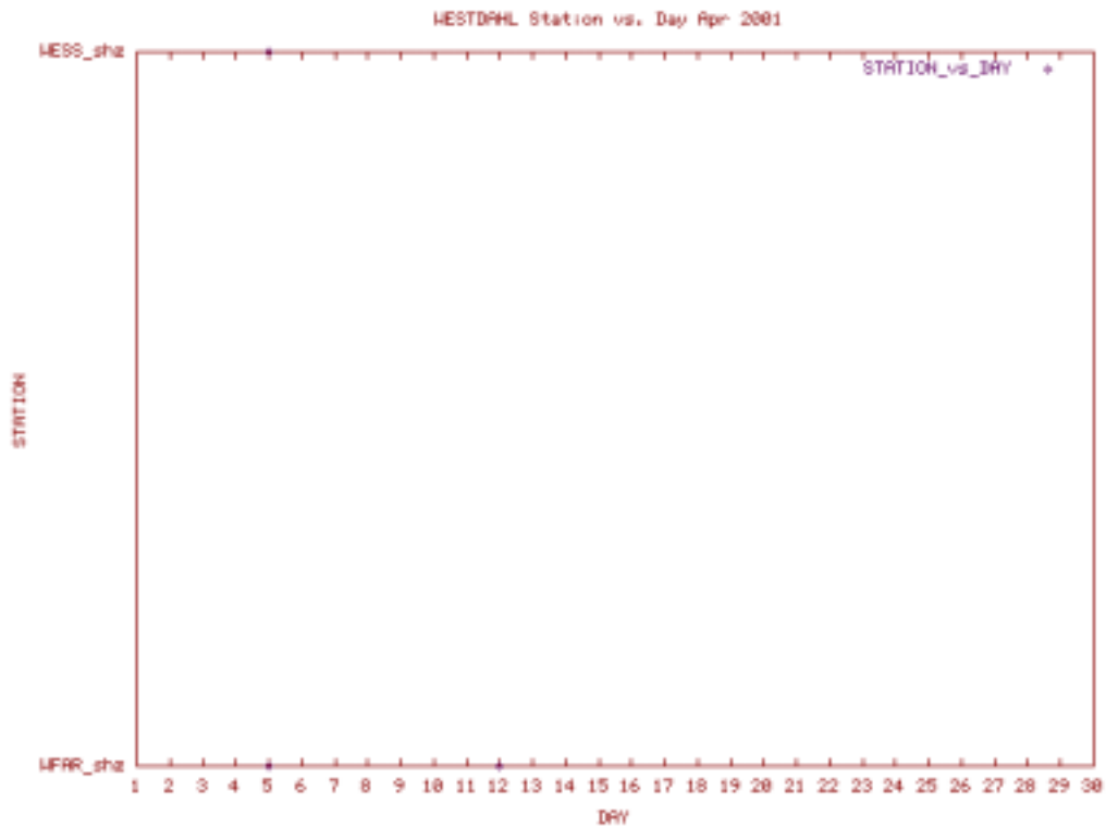
Station Use Plot for the Westdahl subnet for April 2001
