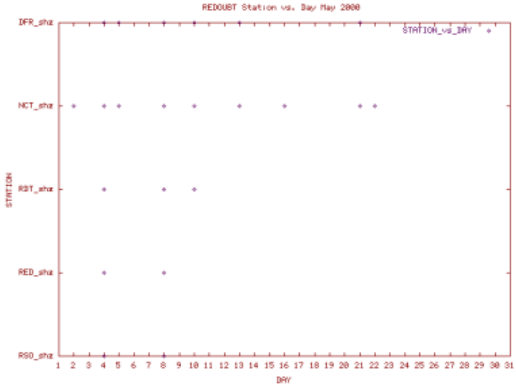
Station Use Plot for the Redoubt subnet for May 2000
