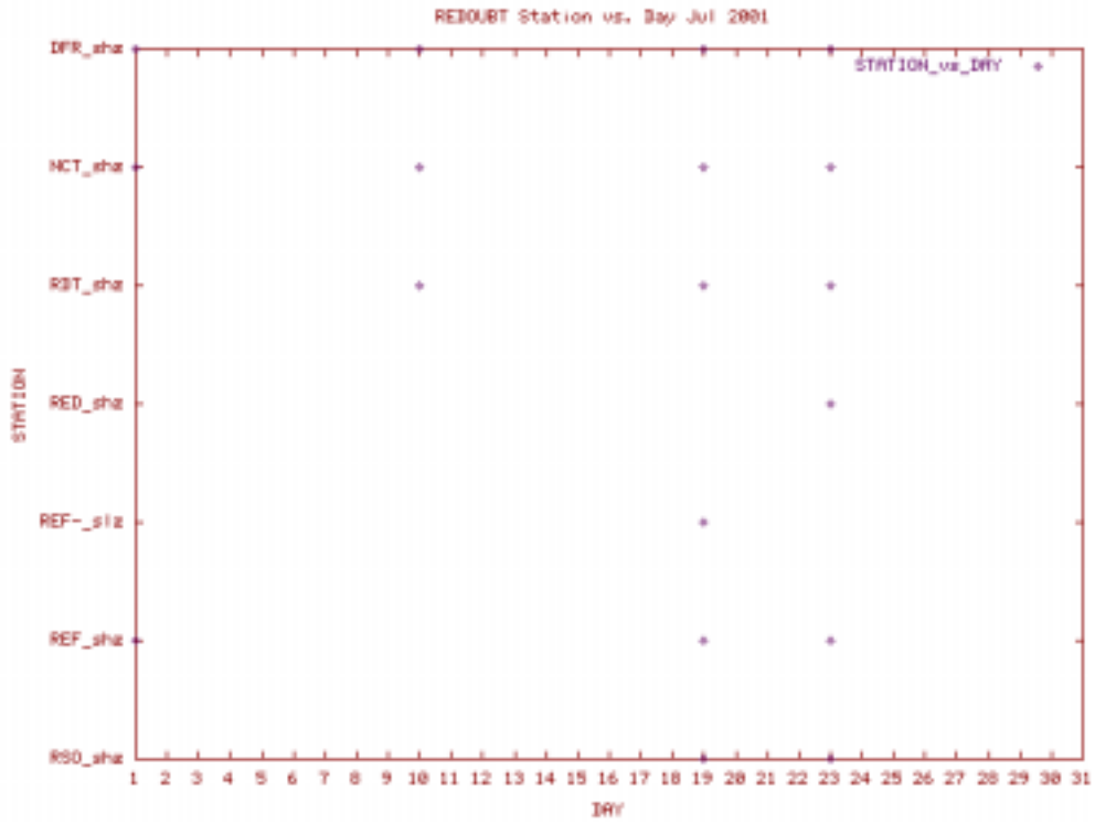
Station Use Plot for the Redoubt subnet for July 2001
