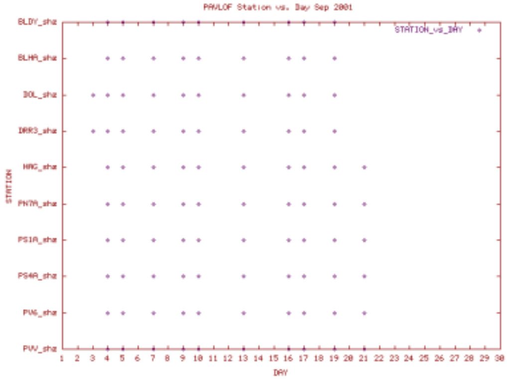
Station Use Plot for the Pavlof subnet for September 2001
