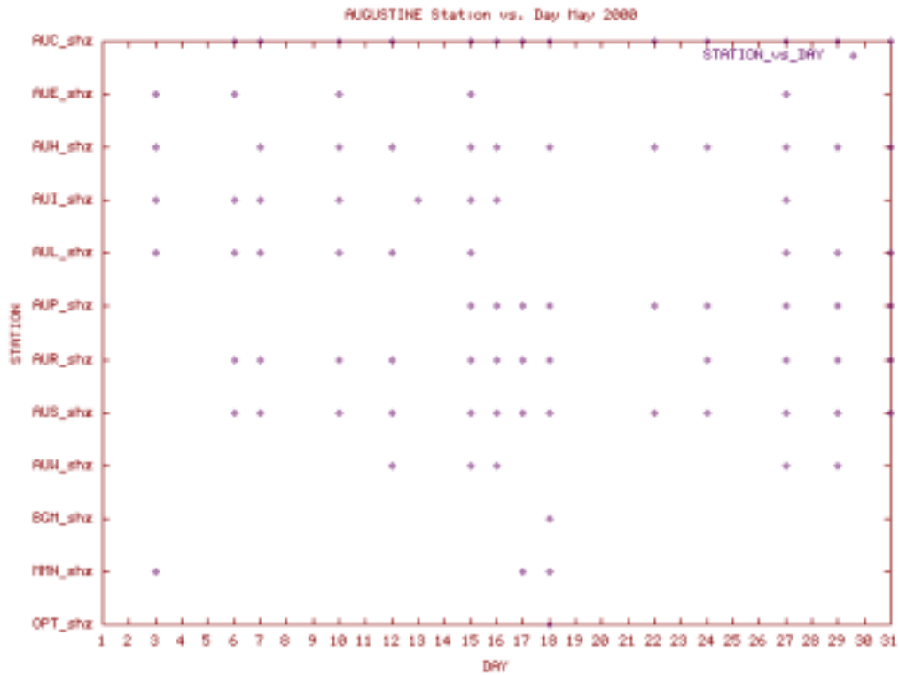
Station Use Plot for the Augustine subnet for May 2000
