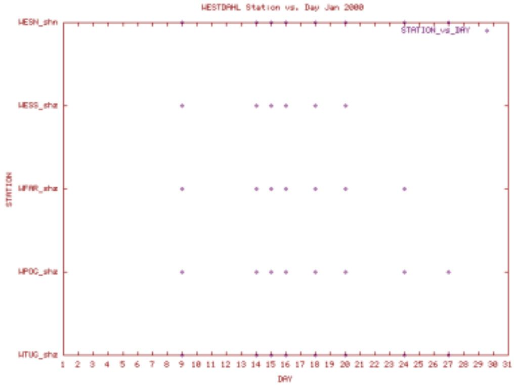
Station Use Plot for the Westdahl subnet for January 2000
