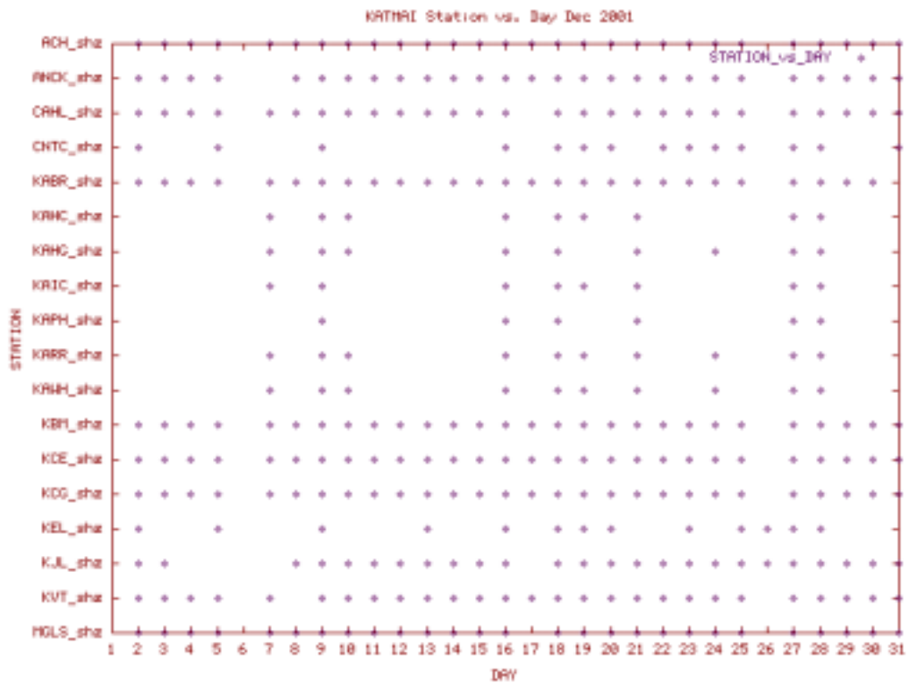
Station Use Plot for the Katmai volcanic group subnet for December 2001
