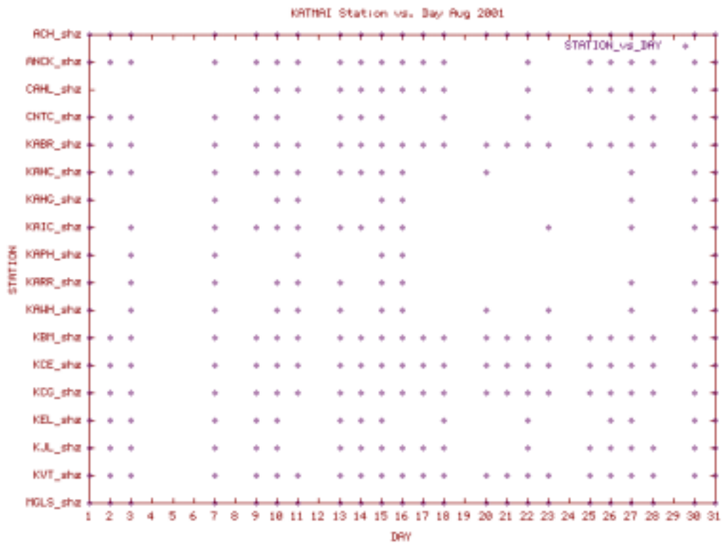
Station Use Plot for the Katmai volcanic group subnet for August 2001
