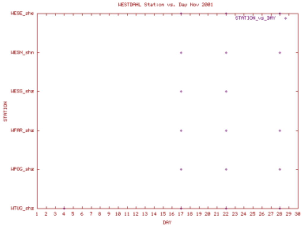
Station Use Plot for the Westdahl subnet for November 2001
