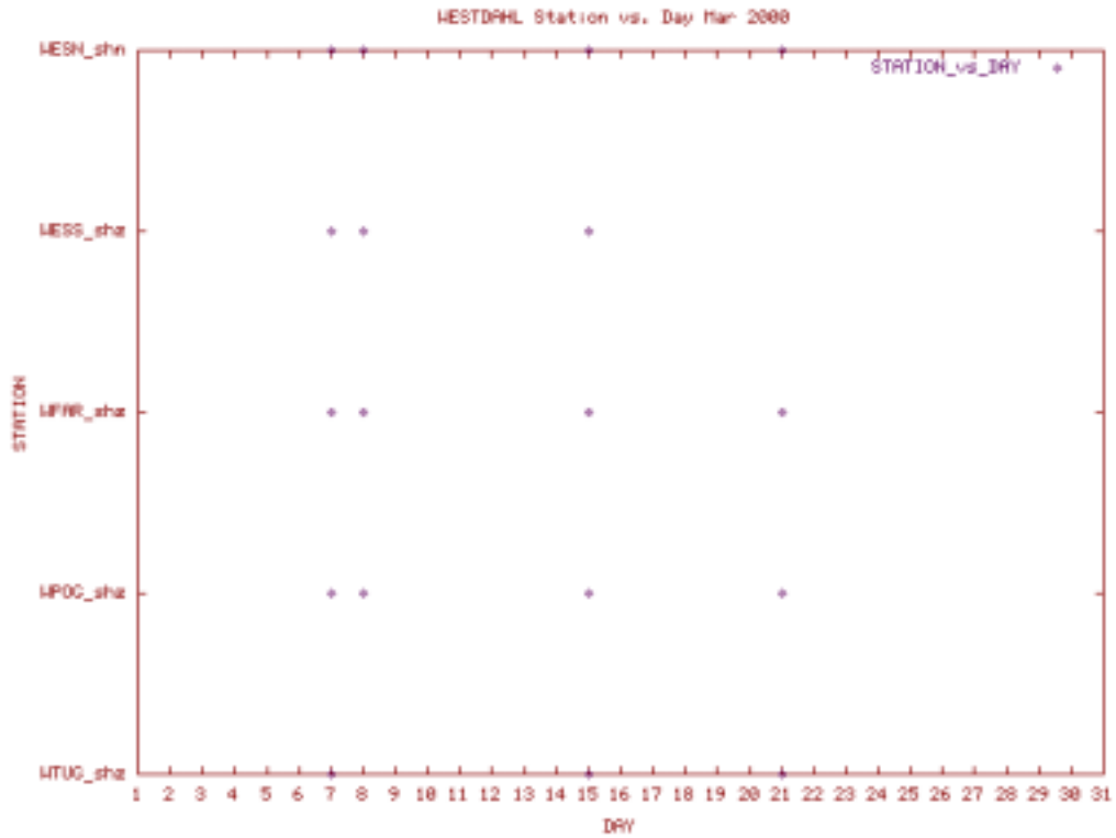
Station Use Plot for the Westdahl subnet for March 2000
