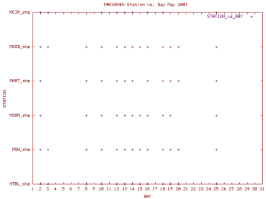
Station Use Plot for the Makushin subnet for May 2001
