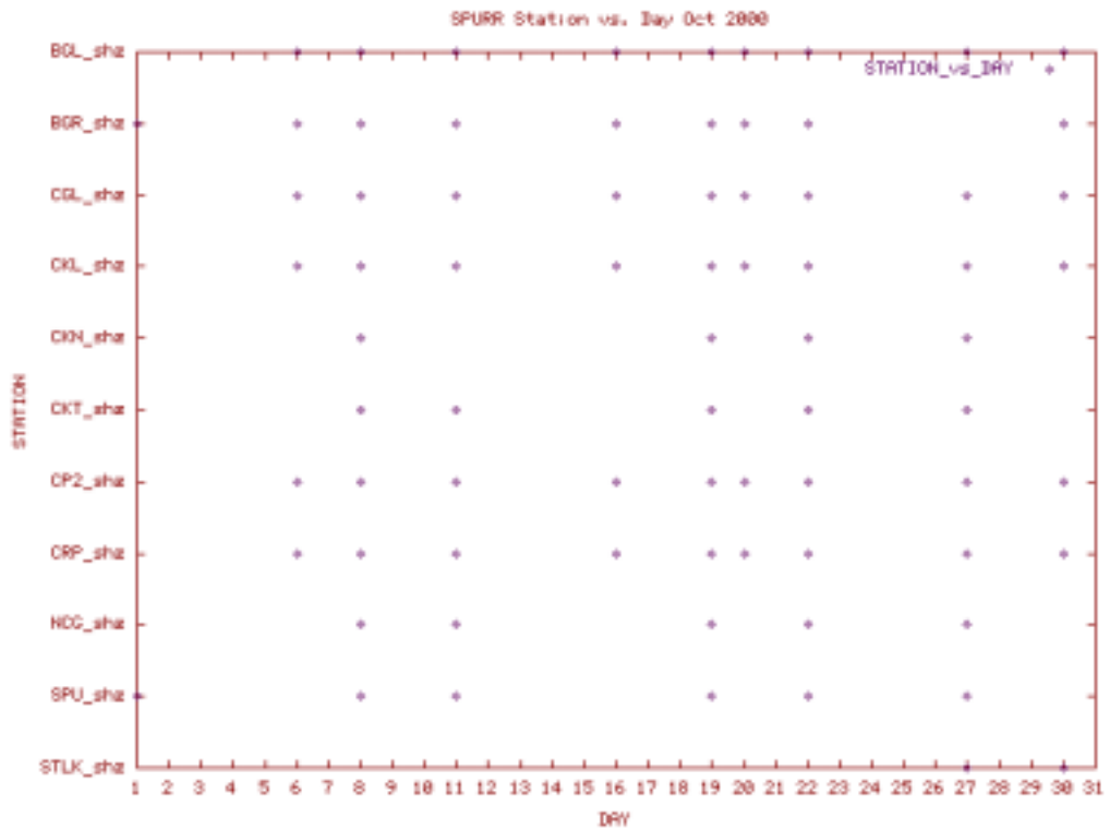
Station Use Plot for the Spurr subnet for October 2000
