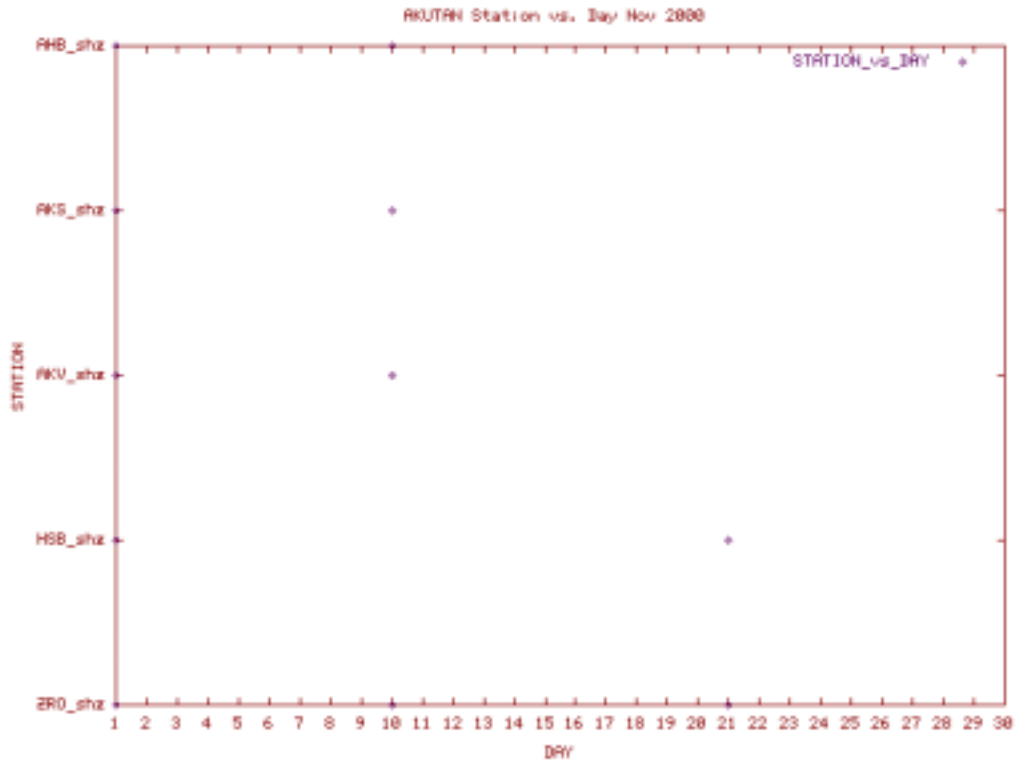
Station Use Plot for the Akutan subnet for November 2000
