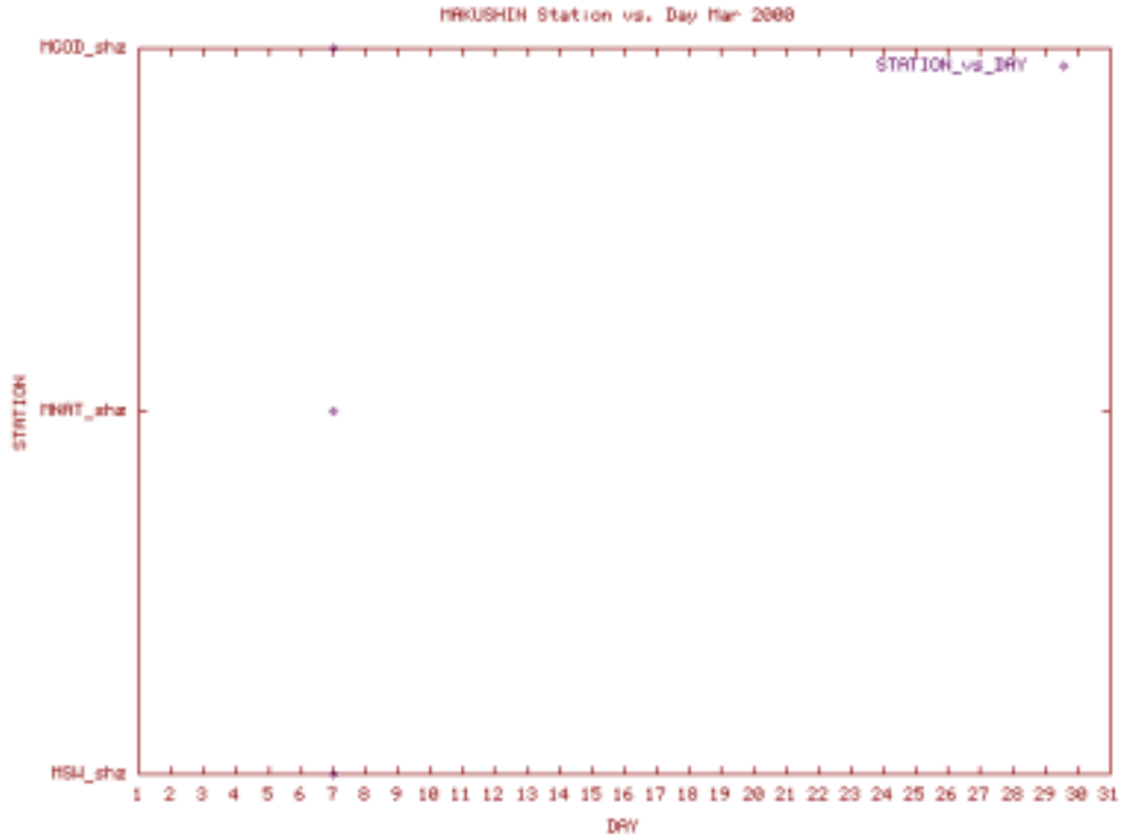
Station Use Plot for the Makushin subnet for March 2000
