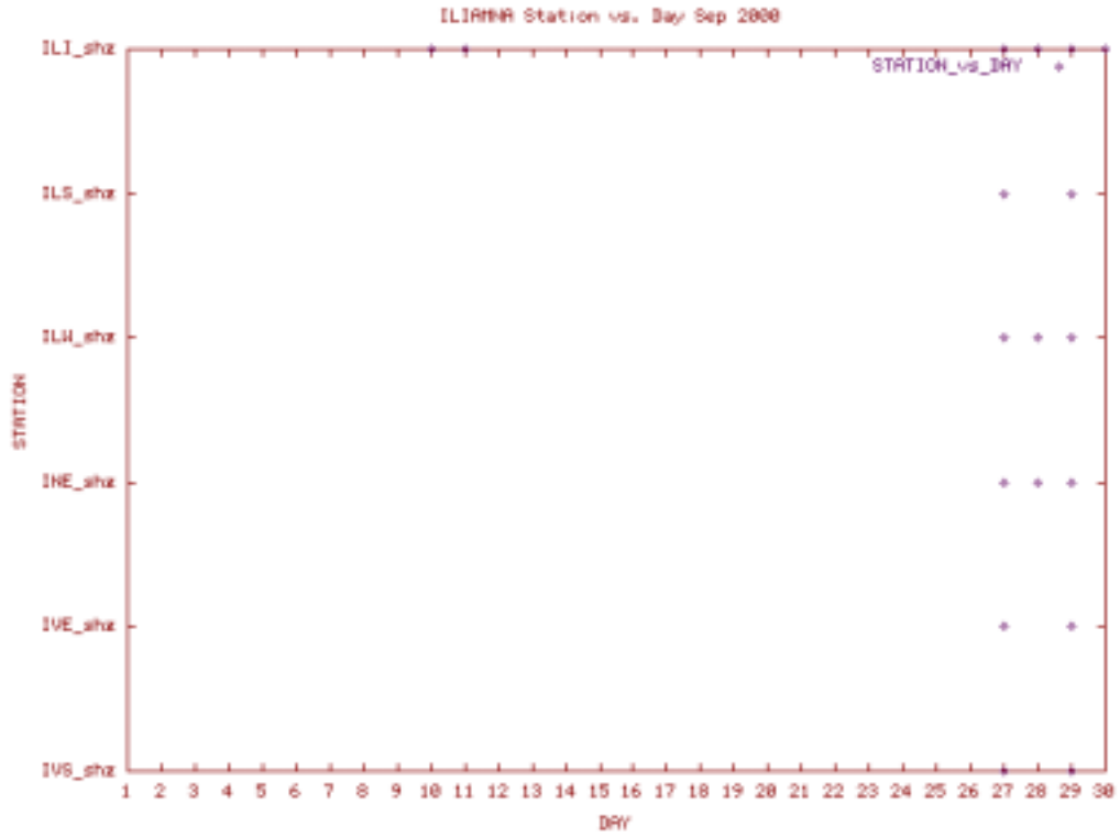
Station Use Plot for the Iliamna subnet for September 2000
