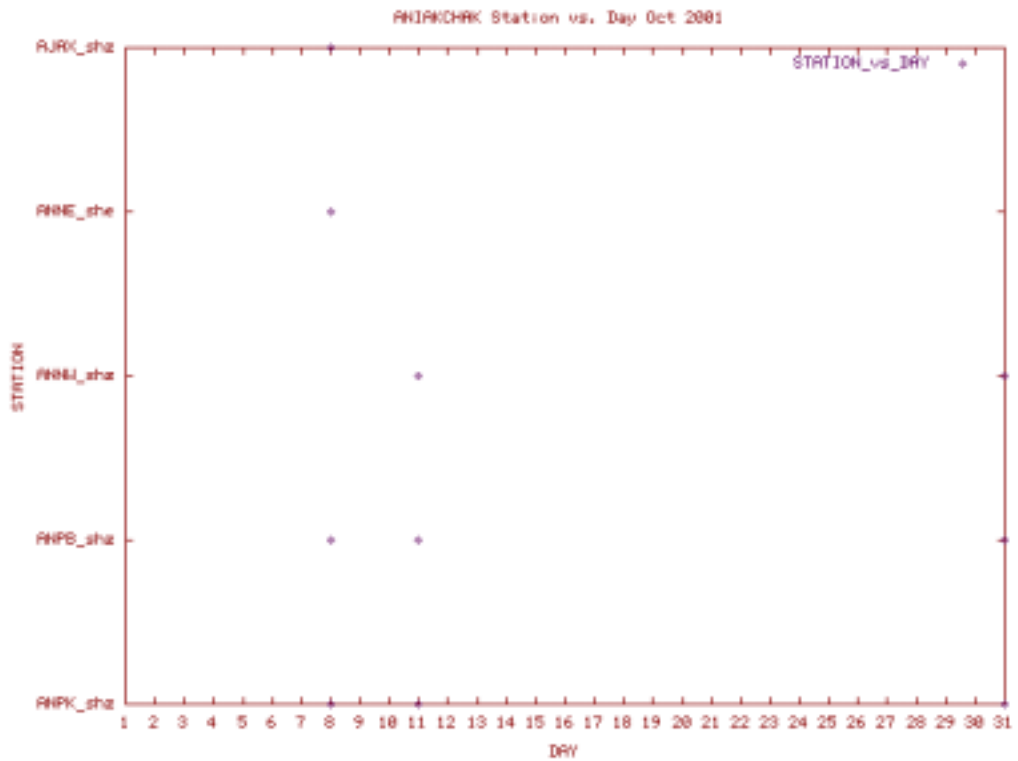
Station Use Plot for the Aniakchak subnet for October 2001
