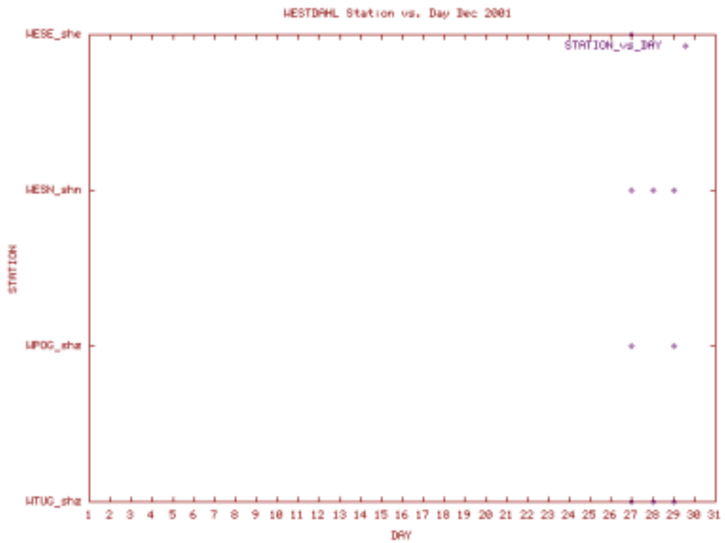
Station Use Plot for the Westdahl subnet for December 2001
