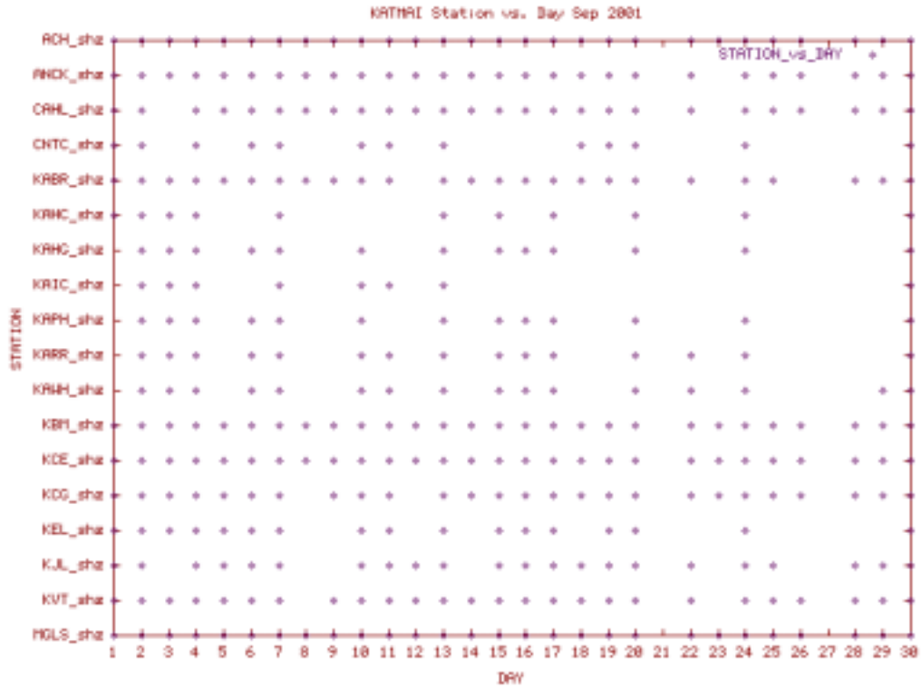
Station Use Plot for the Katmai volcanic group subnet for September 2001
