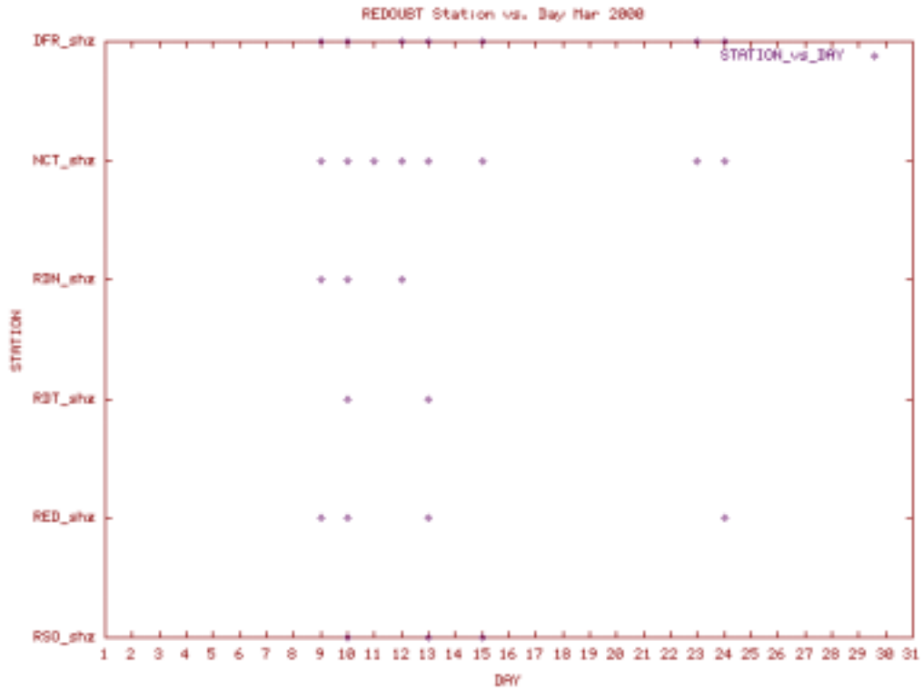
Station Use Plot for the Redoubt subnet for March 2000
