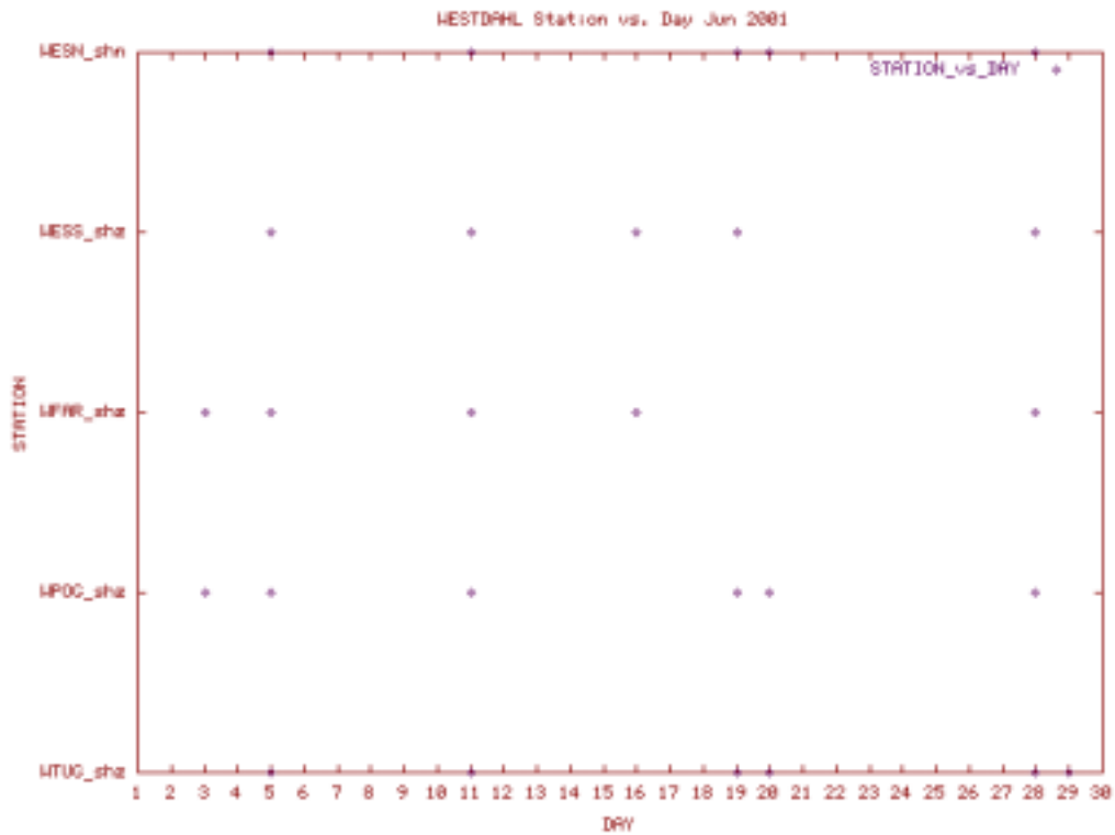
Station Use Plot for the Westdahl subnet for June 2001
