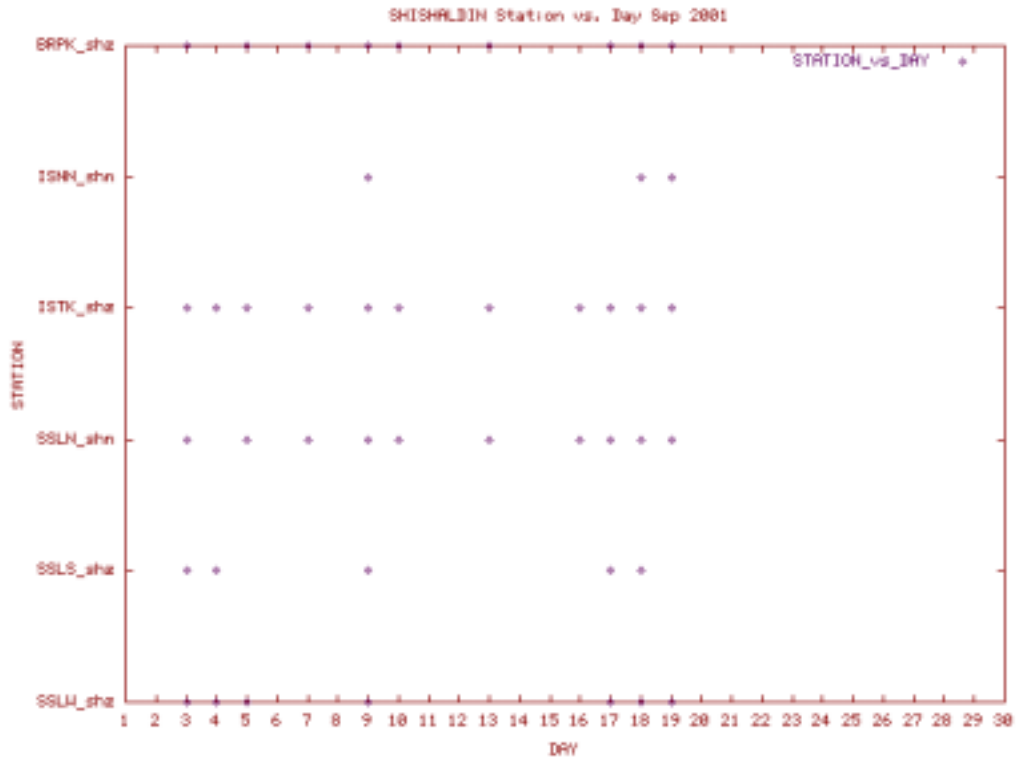
Station Use Plot for the Shishaldin subnet for September 2001
