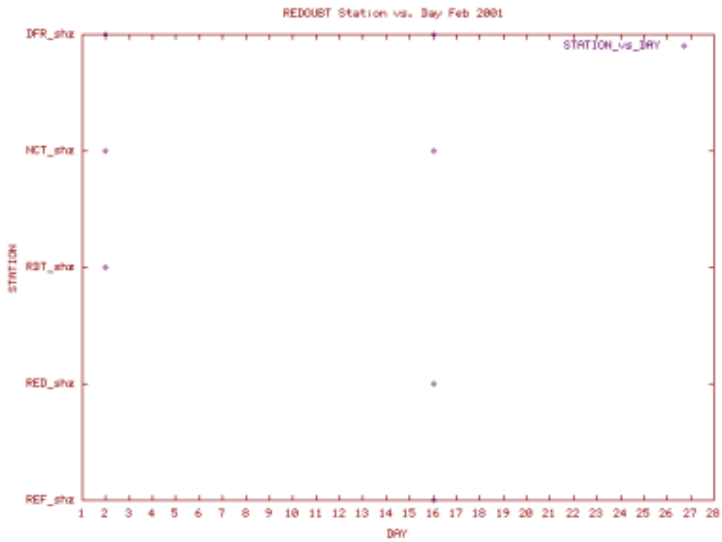
Station Use Plot for the Redoubt subnet for February 2001
