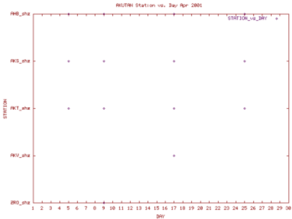
Station Use Plot for the Akutan subnet for April 2001
