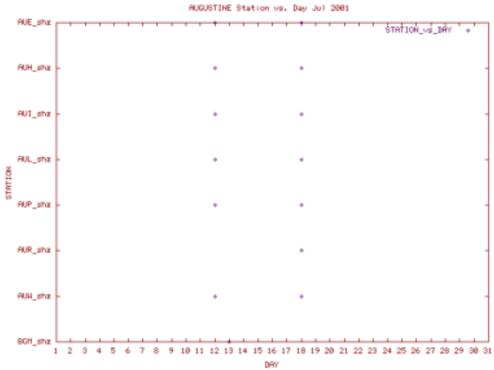
Station Use Plot for the Augustine subnet for July 2001
