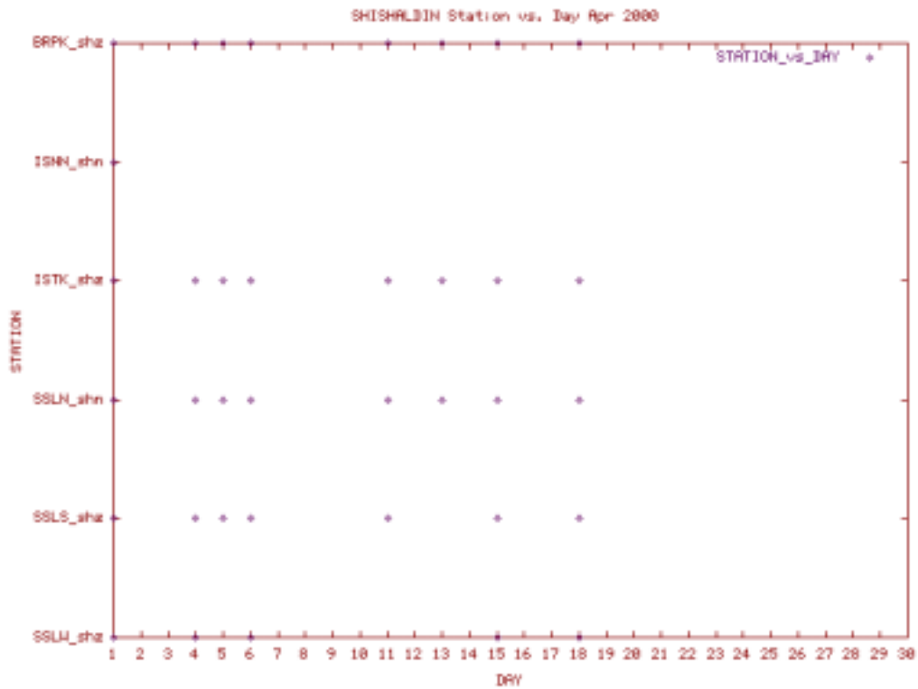
Station Use Plot for the Shishaldin subnet for April 2000
