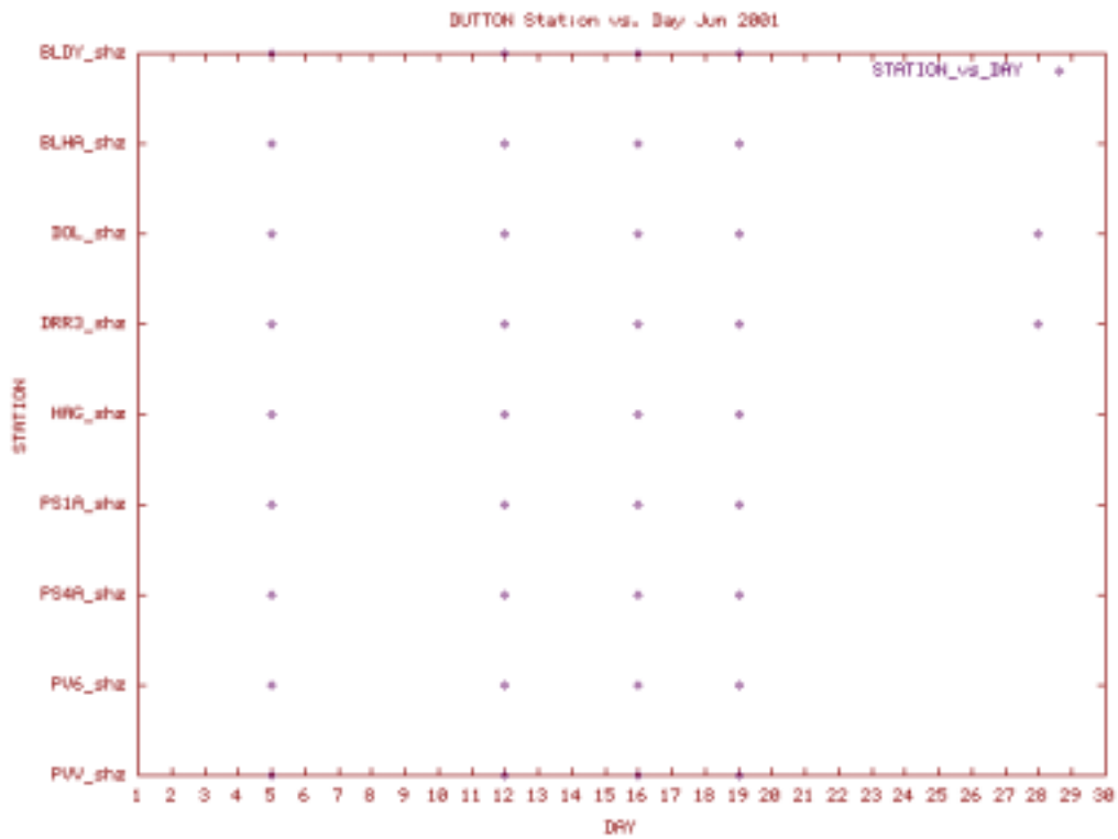
Station Use Plot for the Dutton subnet for June 2001
