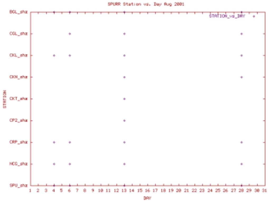
Station Use Plot for the Spurr subnet for August 2001
