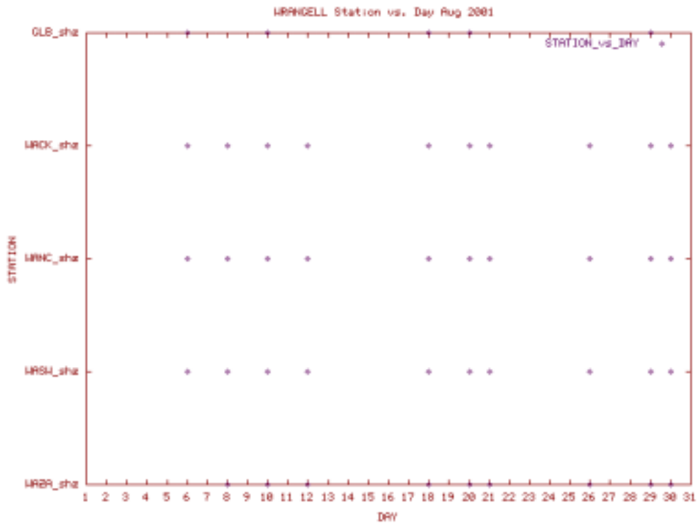
Station Use Plot for the Wrangell subnet for August 2001
