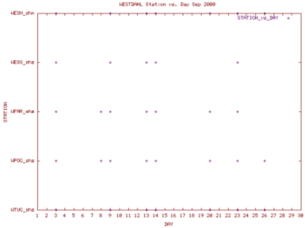
Station Use Plot for the Westdahl subnet for September 2000
