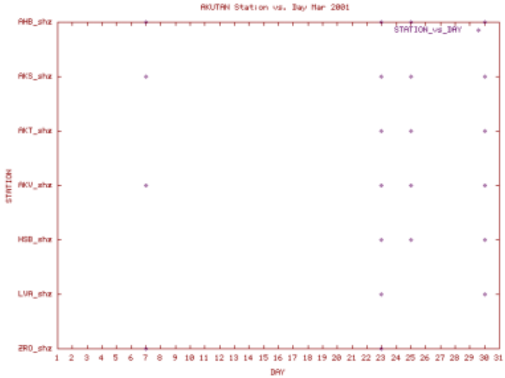
Station Use Plot for the Akutan subnet for March 2001
