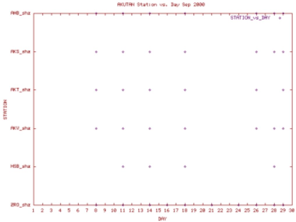
Station Use Plot for the Akutan subnet for September 2000
