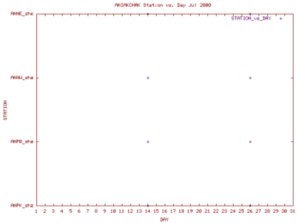
Station Use Plot for the Aniakchak subnet for July 2000
