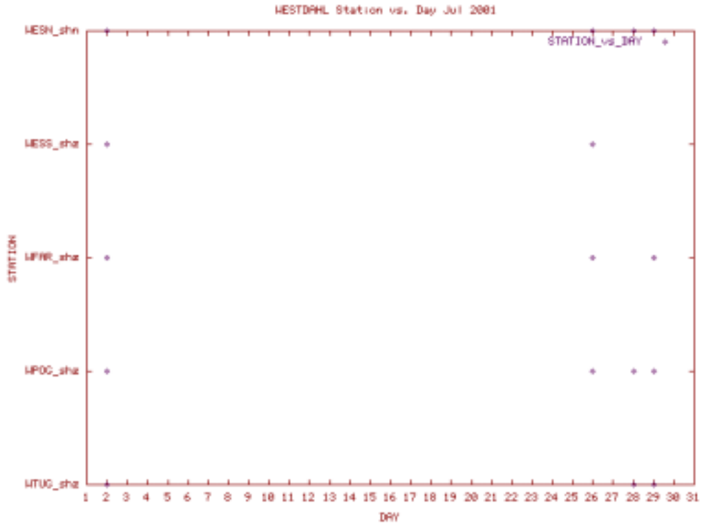
Station Use Plot for the Westdahl subnet for July 2001
