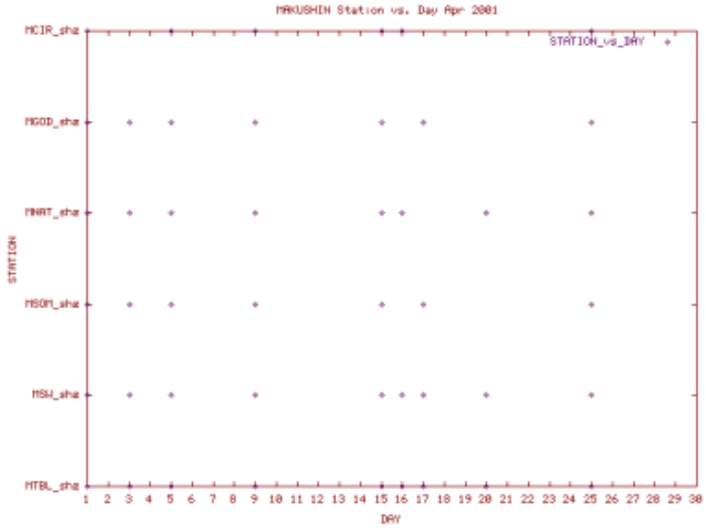
Station Use Plot for the Makushin subnet for April 2001
