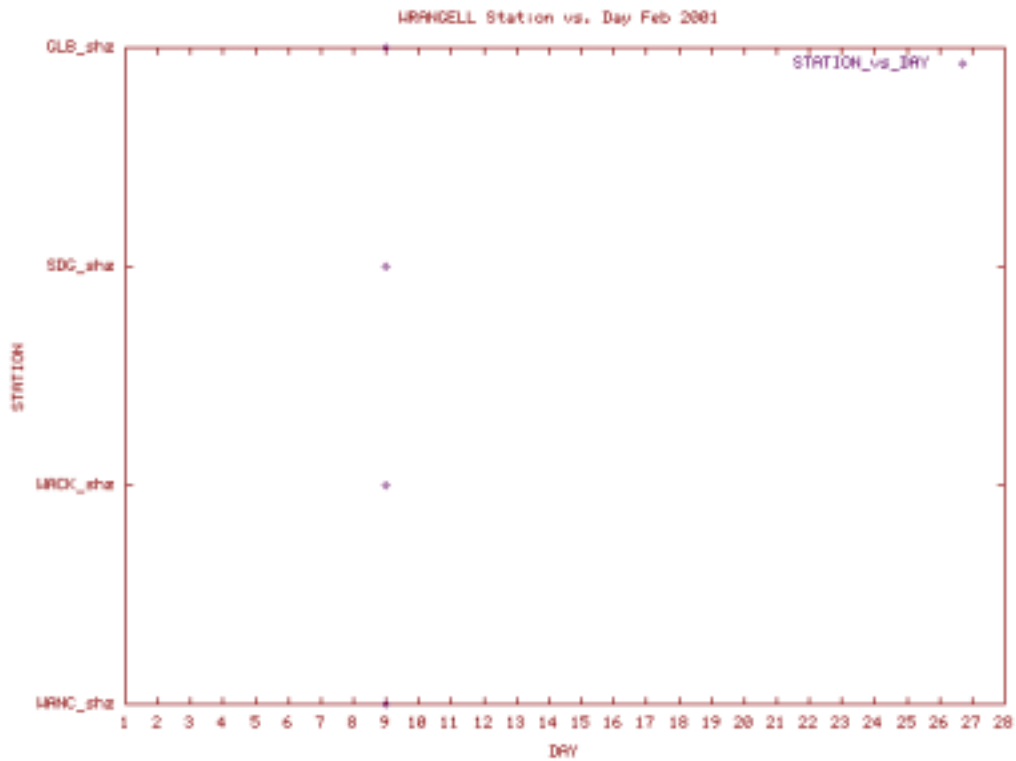
Station Use Plot for the Wrangell subnet for February 2001
