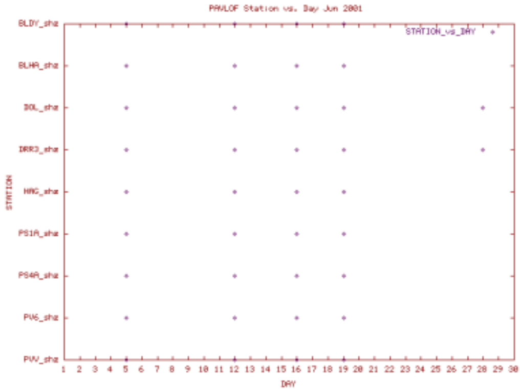
Station Use Plot for the Pavlof subnet for June 2001
