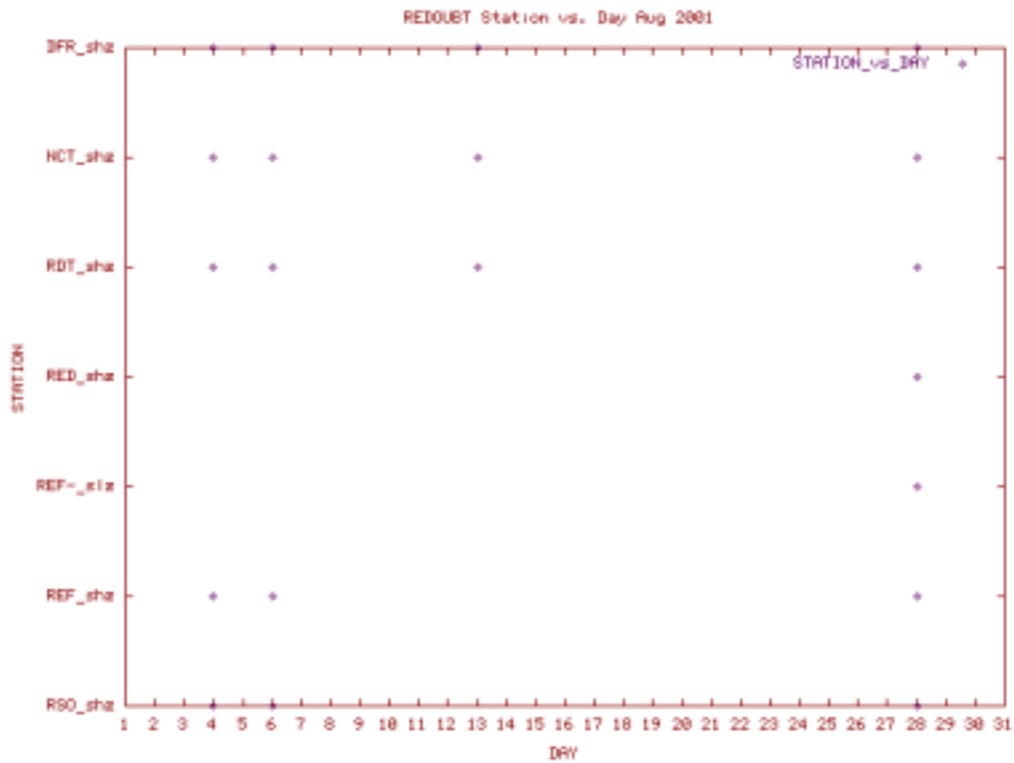
Station Use Plot for the Redoubt subnet for August 2001
