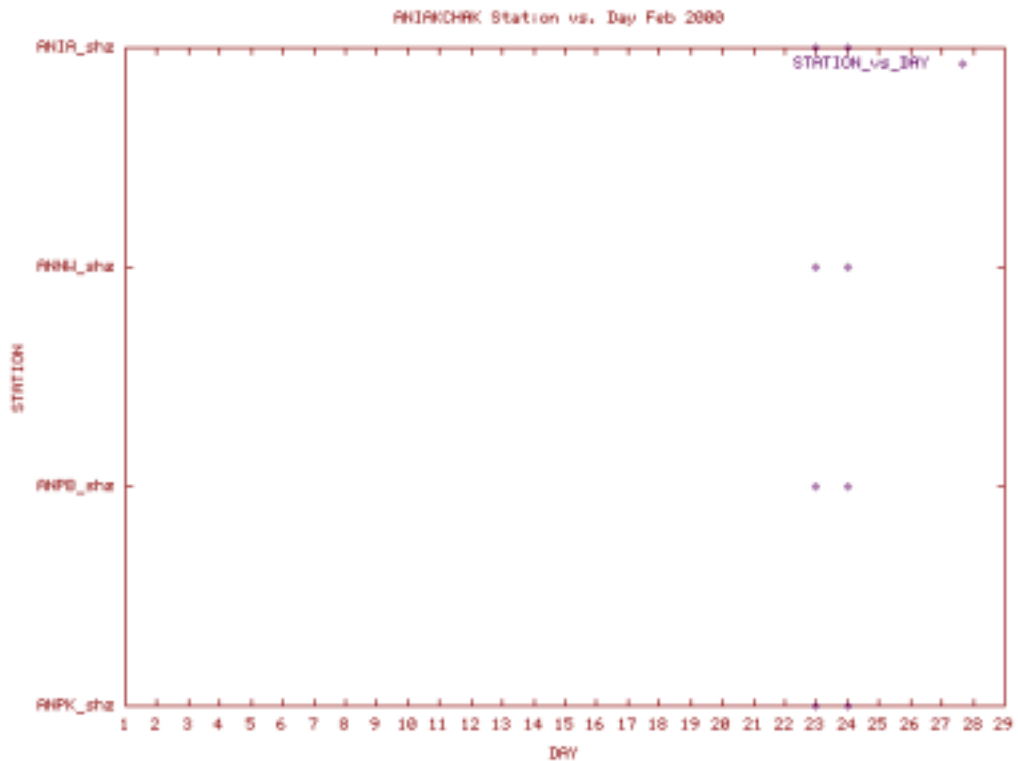
Station Use Plot for the Aniakchak subnet for February 2000
