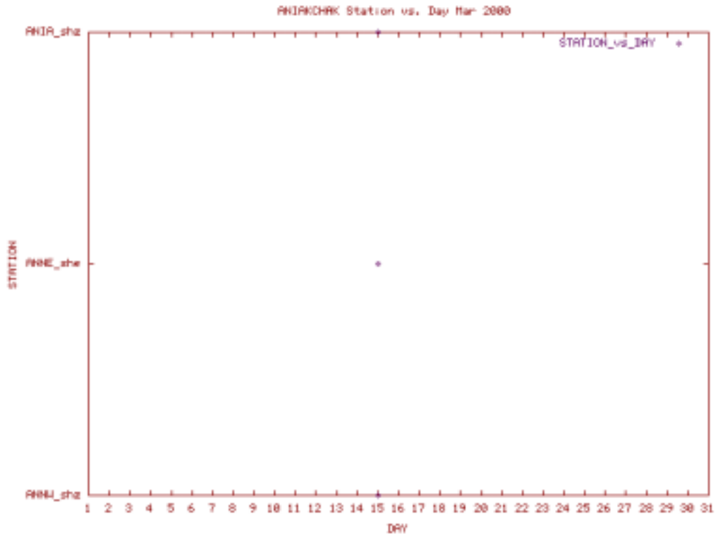
Station Use Plot for the Aniakchak subnet for March 2000
