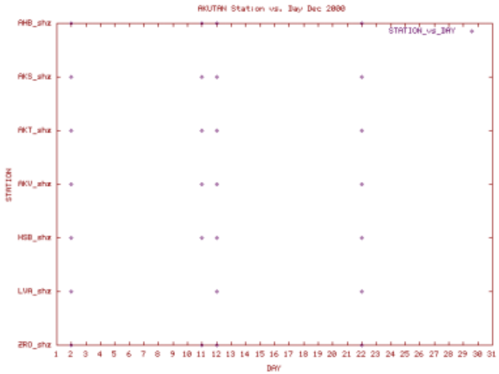
Station Use Plot for the Akutan subnet for December 2000
