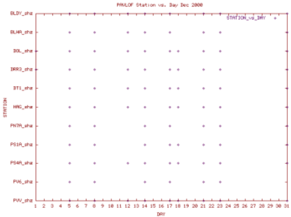
Station Use Plot for the Pavlof subnet for December 2000
