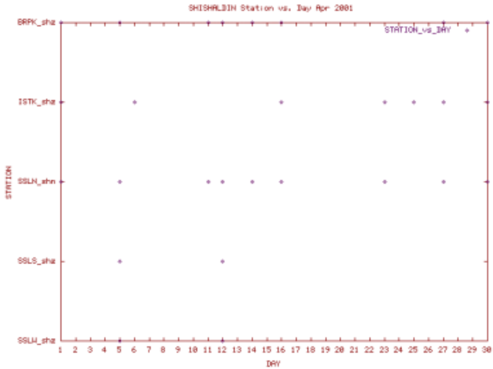
Station Use Plot for the Shishaldin subnet for April 2001
