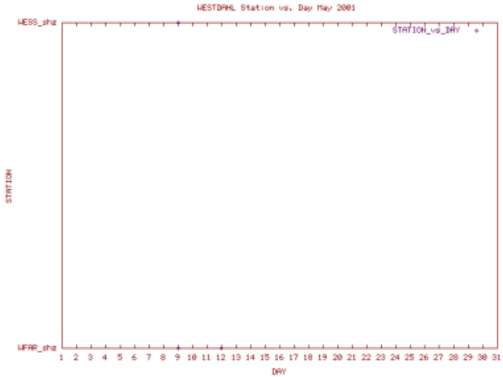
Station Use Plot for the Westdahl subnet for May 2001
