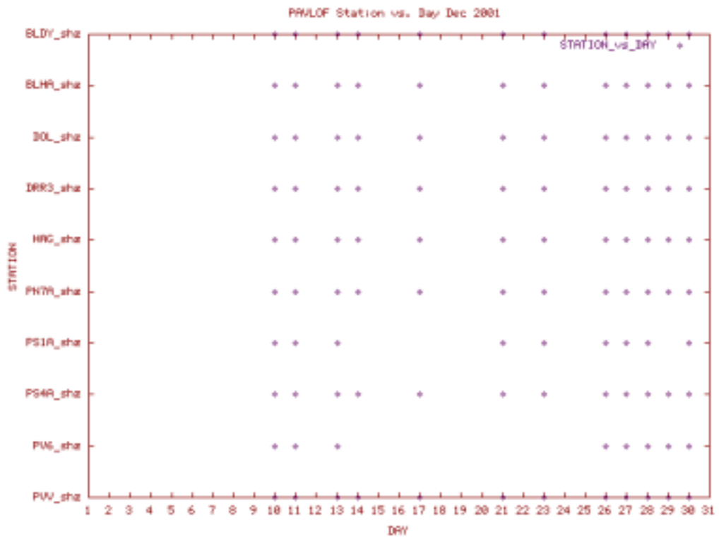
Station Use Plot for the Pavlof subnet for December 2001
