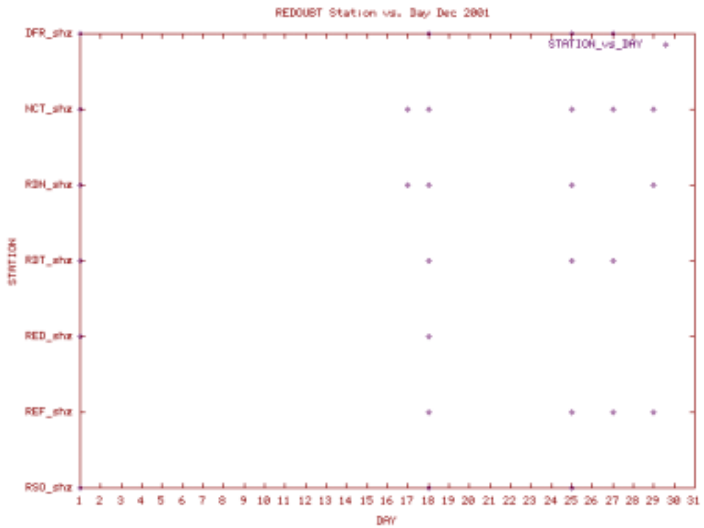
Station Use Plot for the Redoubt subnet for December 2001
