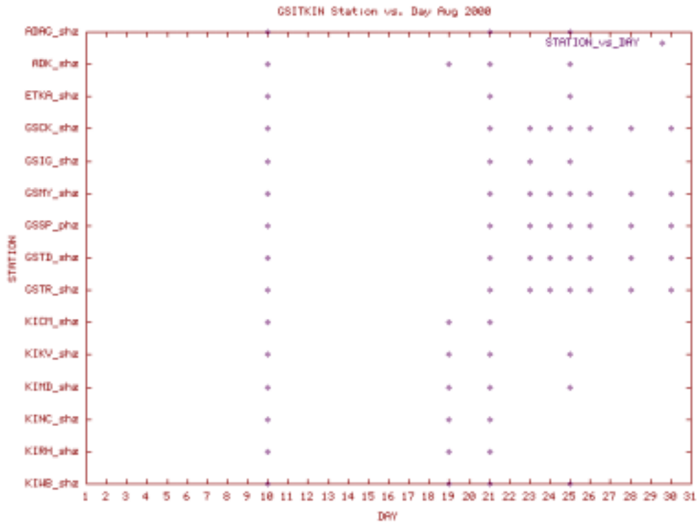
Station Use Plot for the Great Sitkin subnet for August 2000
