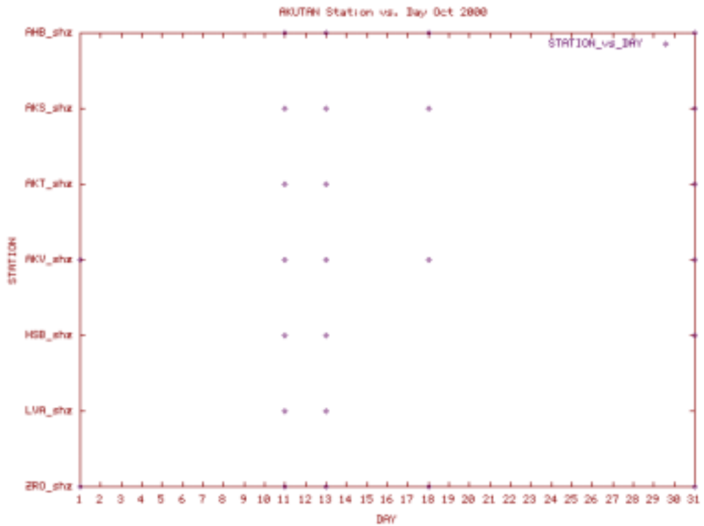
Station Use Plot for the Akutan subnet for October 2000
