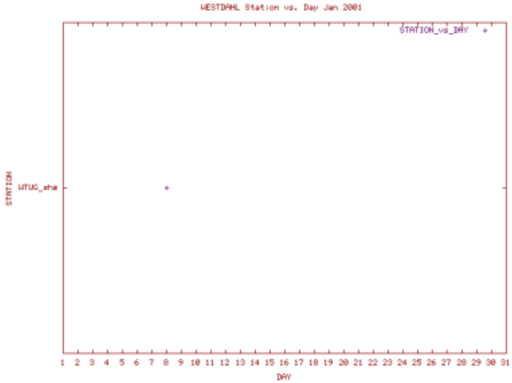
Station Use Plot for the Westdahl subnet for January 2001
