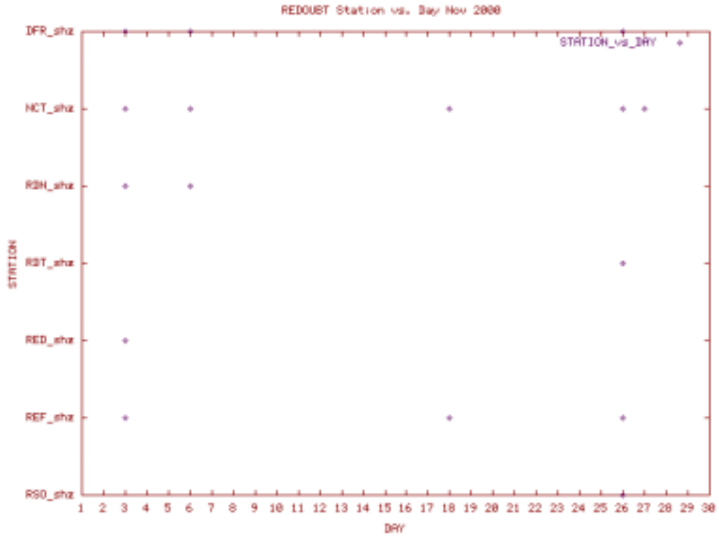
Station Use Plot for the Redoubt subnet for November 2000
