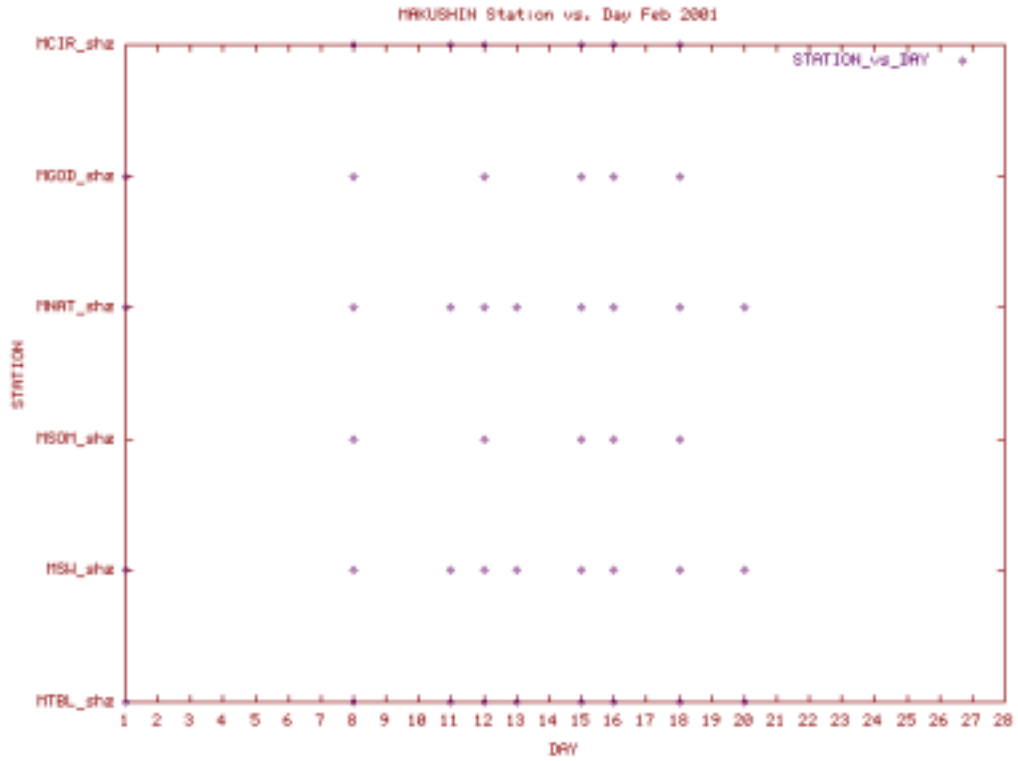
Station Use Plot for the Makushin subnet for February 2001
