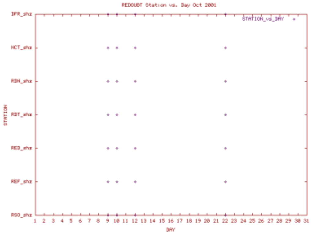
Station Use Plot for the Redoubt subnet for October 2001
