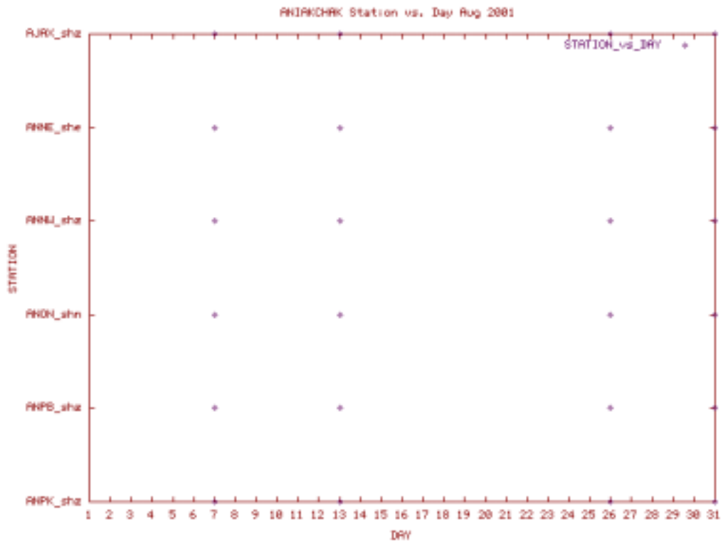
Station Use Plot for the Aniakchak subnet for August 2001
