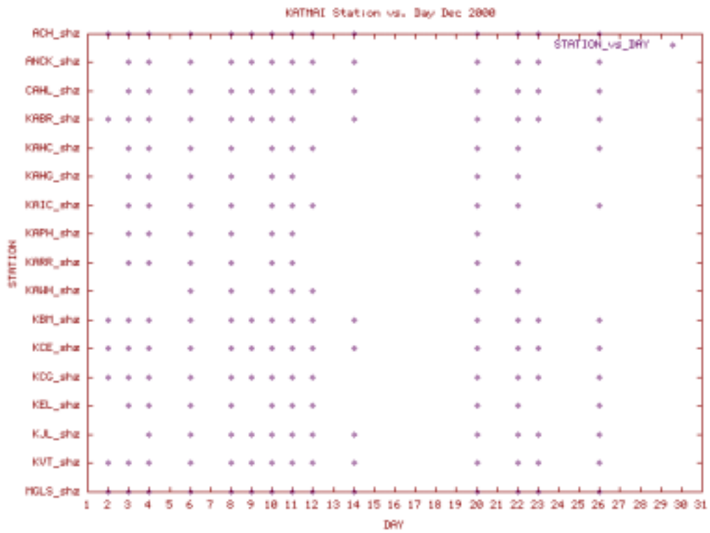
Station Use Plot for the Katmai volcanic group subnet for December 2000
