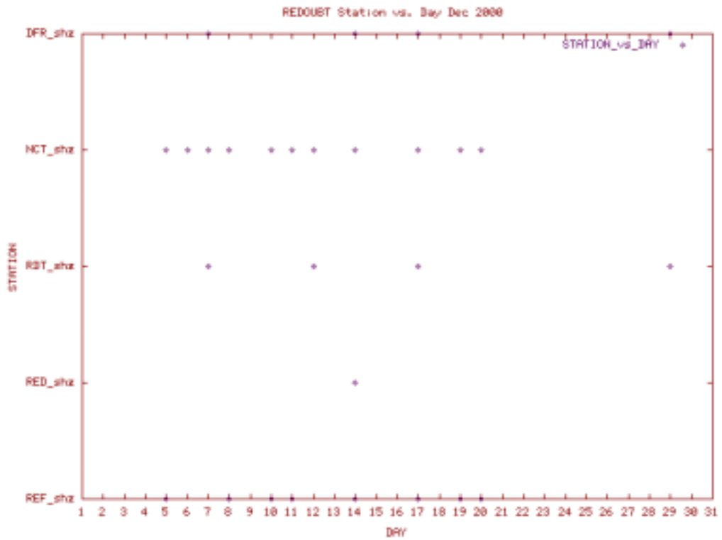
Station Use Plot for the Redoubt subnet for December 2000
