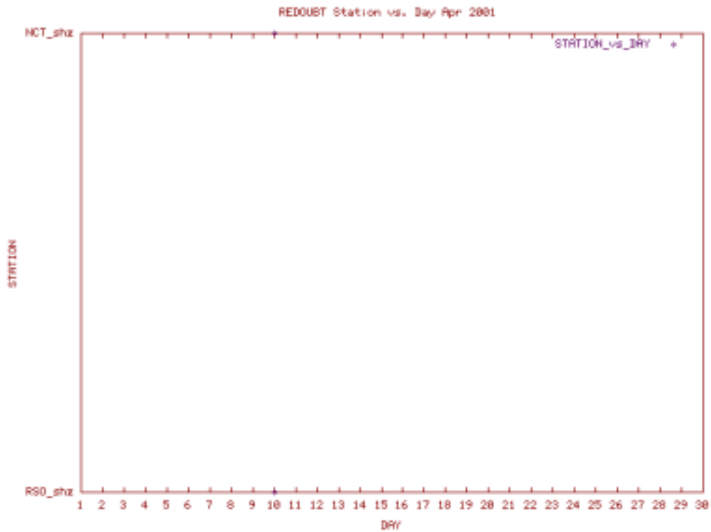
Station Use Plot for the Redoubt subnet for April 2001
