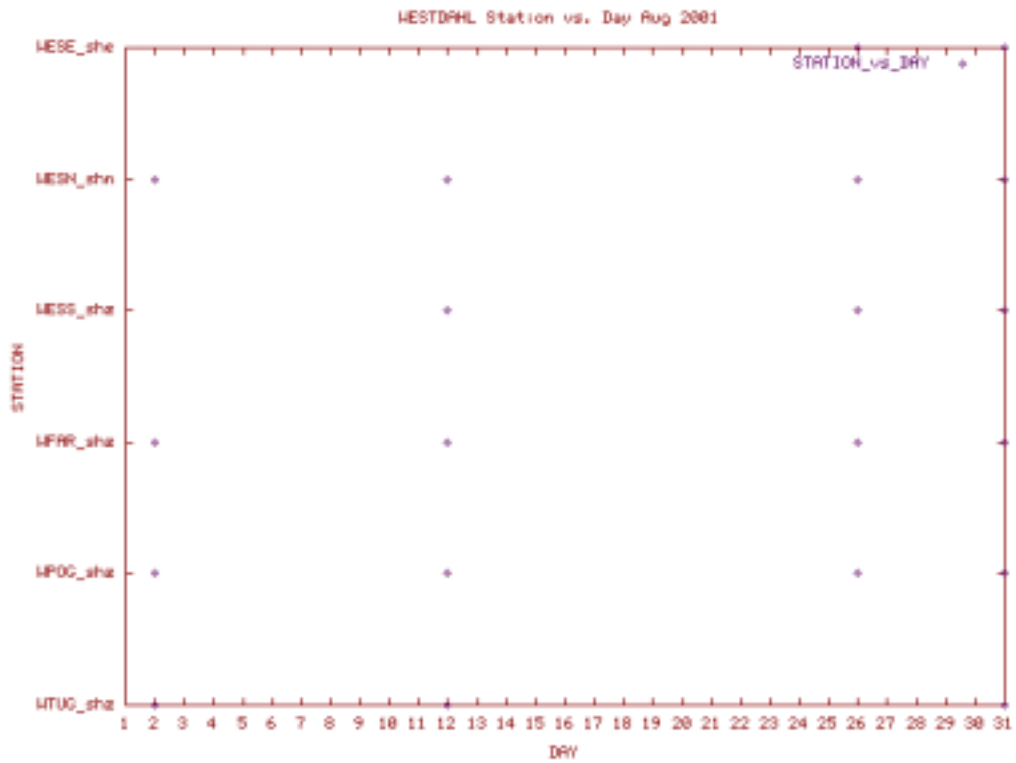
Station Use Plot for the Westdahl subnet for August 2001
