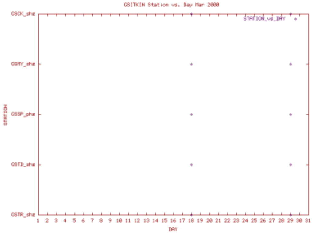
Station Use Plot for the Great Sitkin subnet for March 2000
