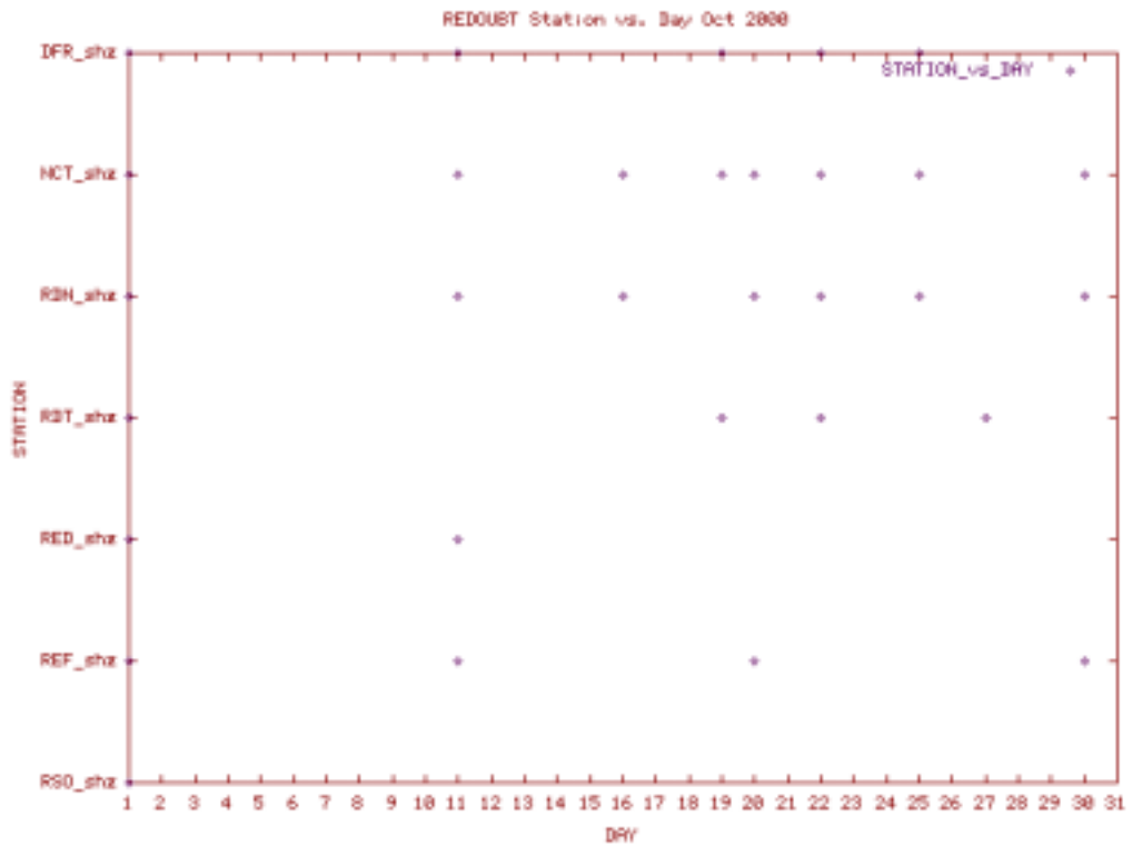
Station Use Plot for the Redoubt subnet for October 2000
