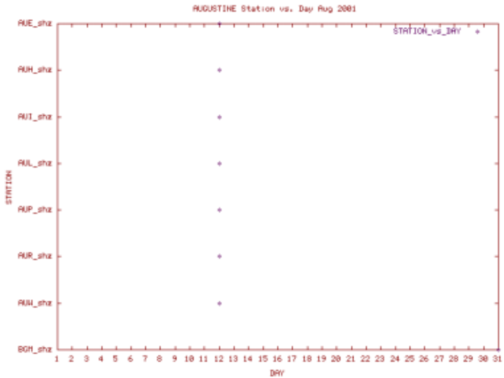
Station Use Plot for the Augustine subnet for August 2001
