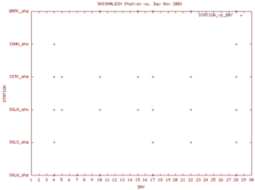
Station Use Plot for the Shishaldin subnet for November 2001
