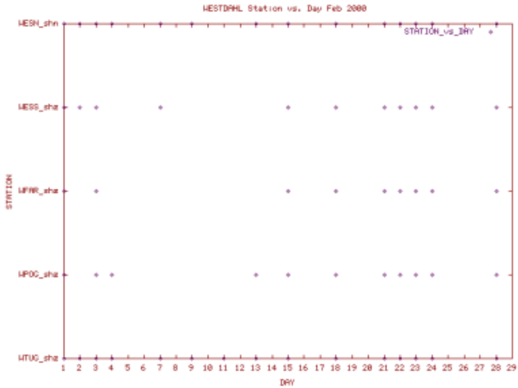
Station Use Plot for the Westdahl subnet for February 2000
