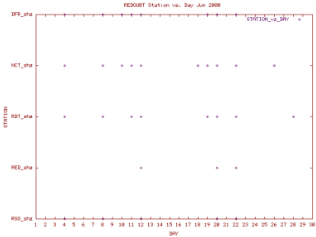
Station Use Plot for the Redoubt subnet for June 2000
