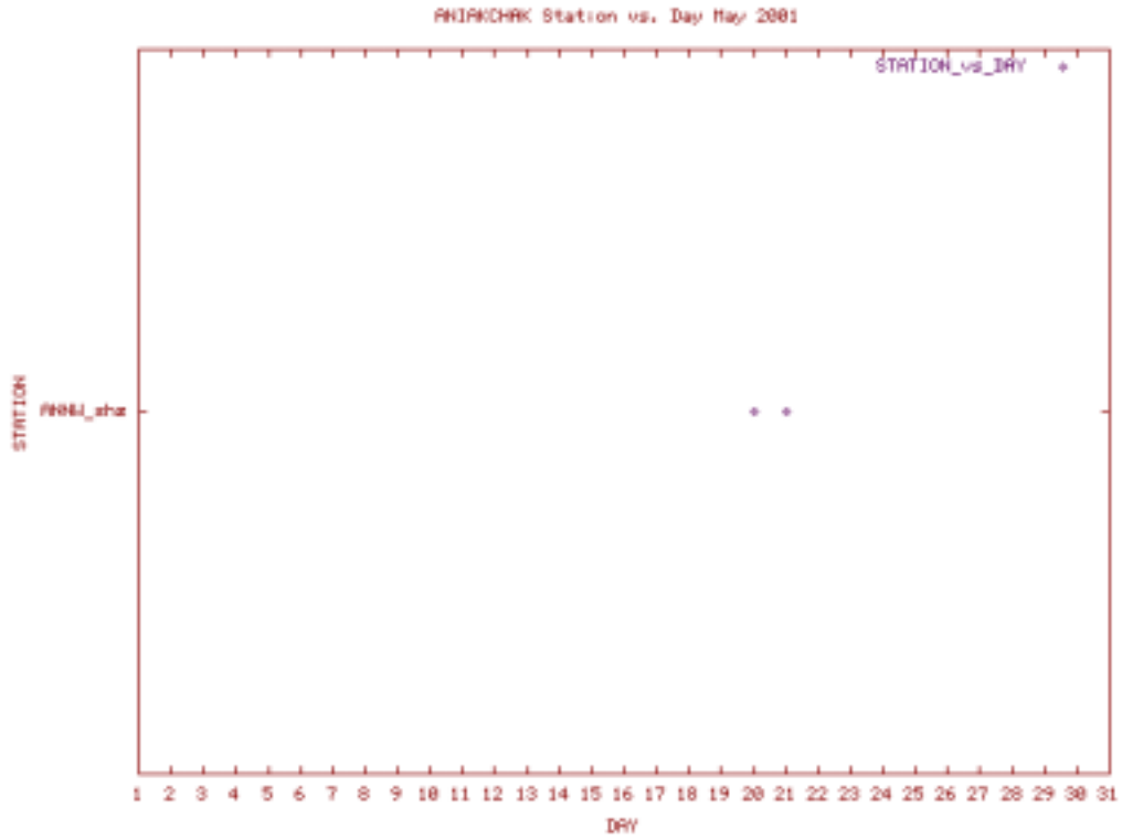
Station Use Plot for the Aniakchak subnet for May 2001
