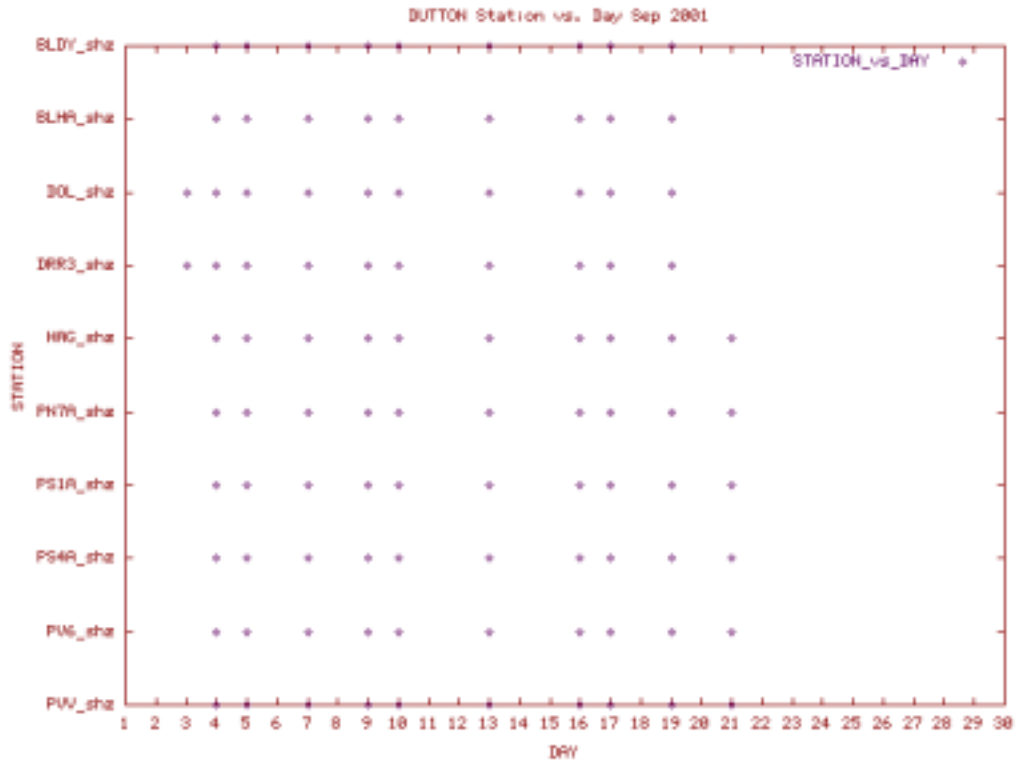
Station Use Plot for the Dutton subnet for September 2001
