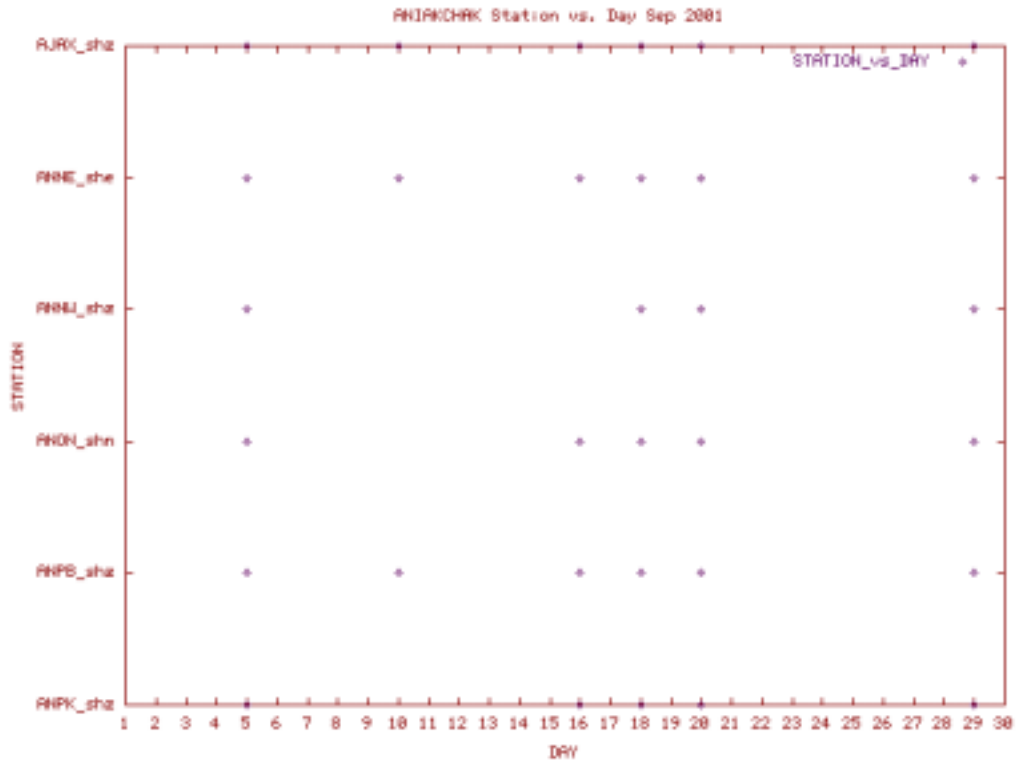
Station Use Plot for the Aniakchak subnet for September 2001
