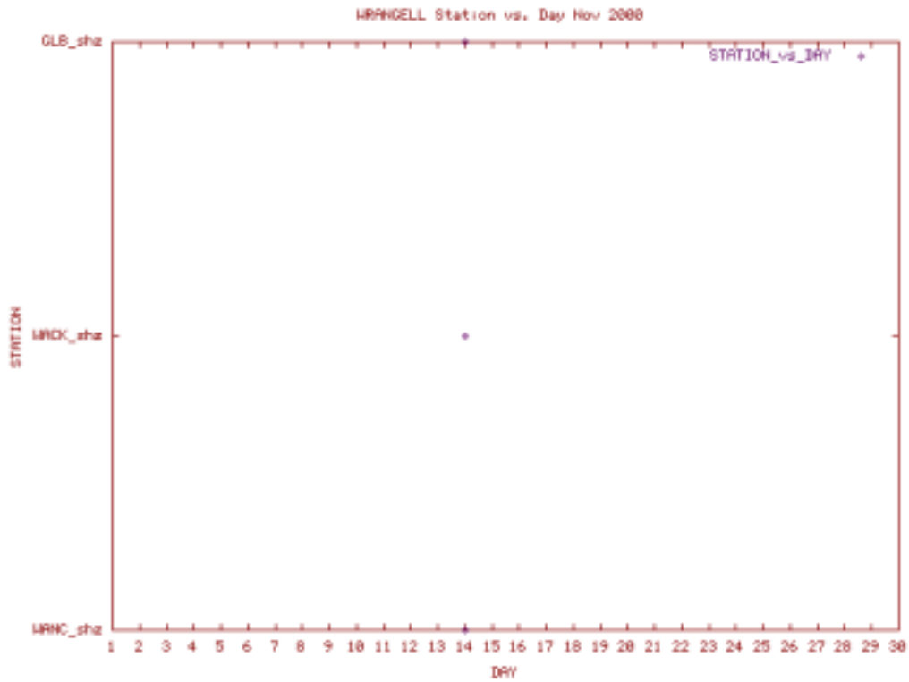
Station Use Plot for the Wrangell subnet for November 2000
