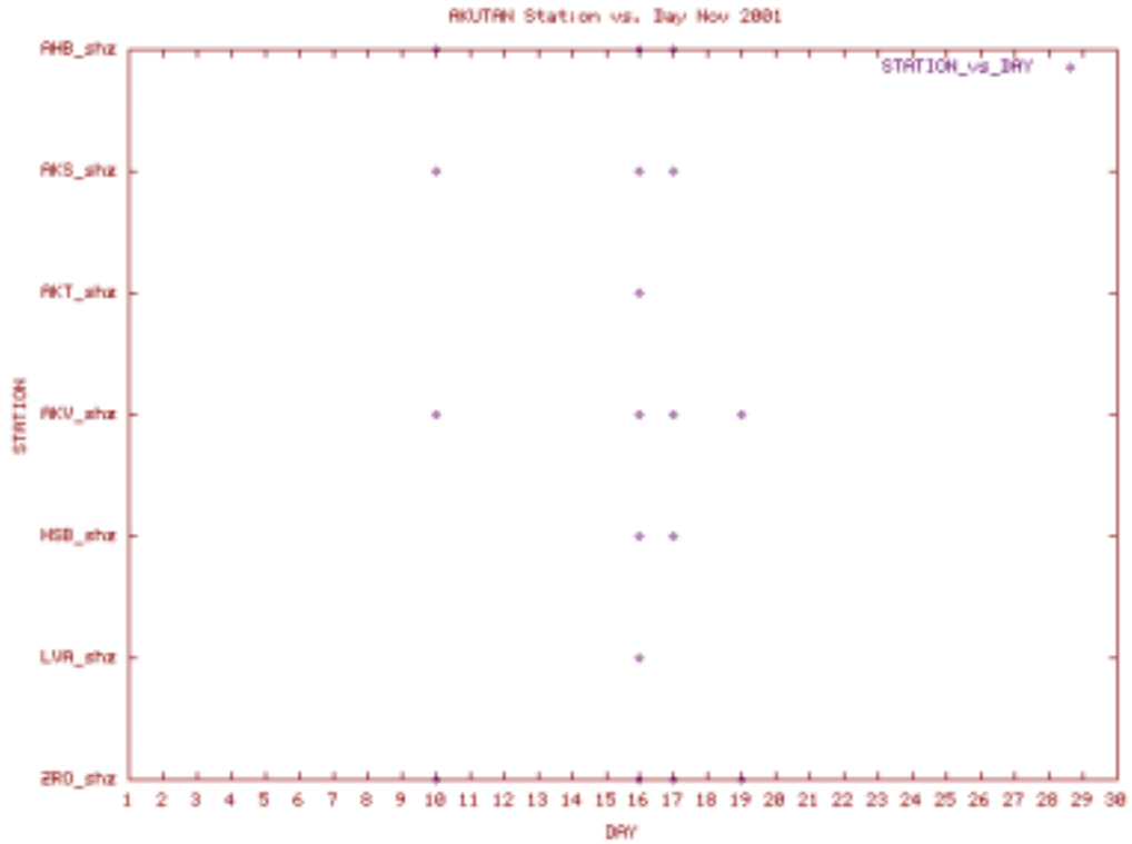
Station Use Plot for the Akutan subnet for November 2001
