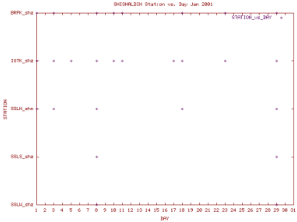
Station Use Plot for the Shishaldin subnet for January 2001
