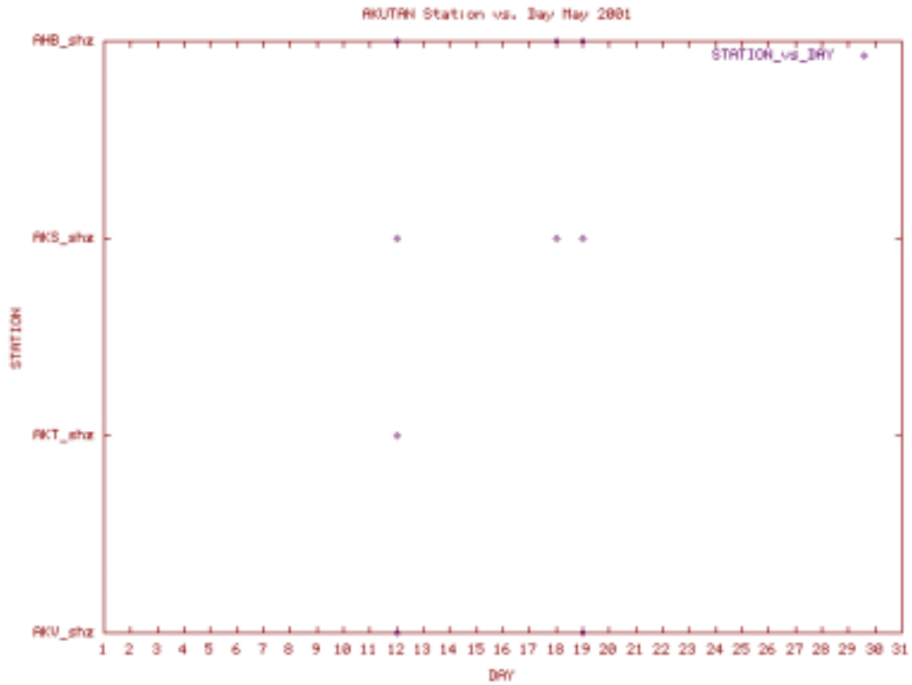
Station Use Plot for the Akutan subnet for May 2001
