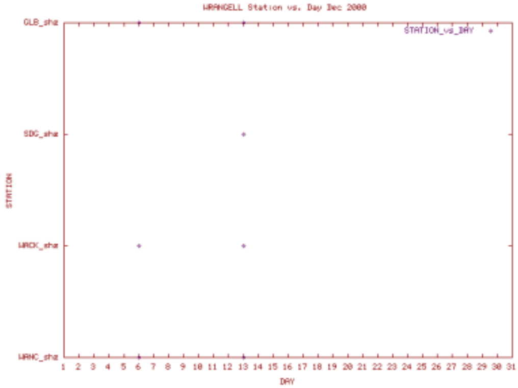
Station Use Plot for the Wrangell subnet for December 2000
