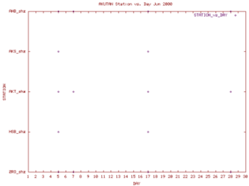
Station Use Plot for the Akutan subnet for June 2000
