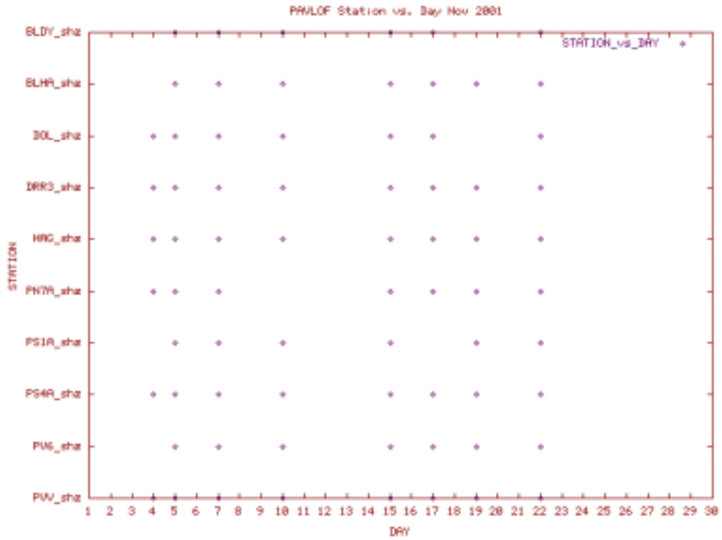
Station Use Plot for the Pavlof subnet for November 2001
