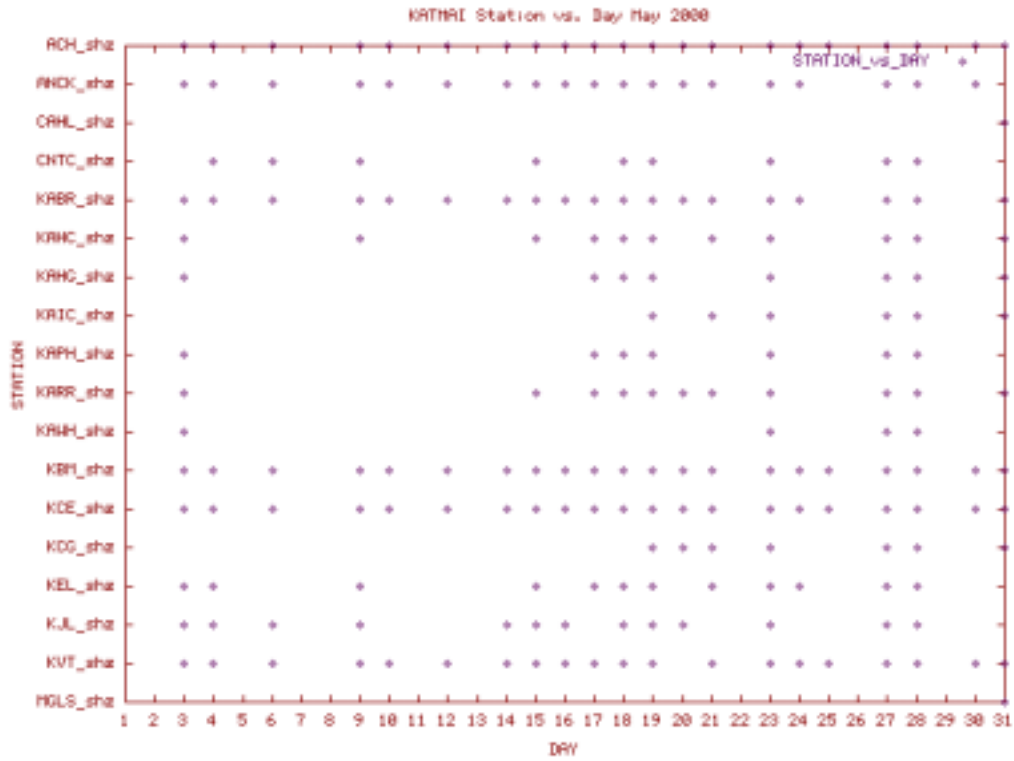
Station Use Plot for the Katmai volcanic group subnet for May 2000
