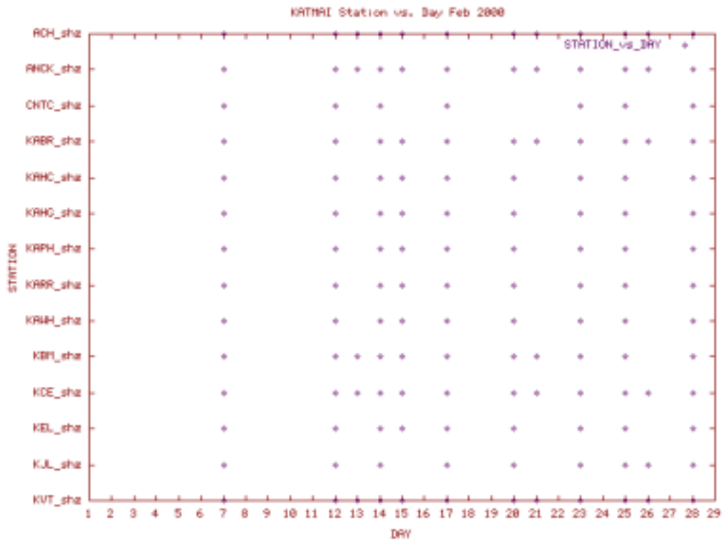
Station Use Plot for the Katmai volcanic group subnet for February 2000
