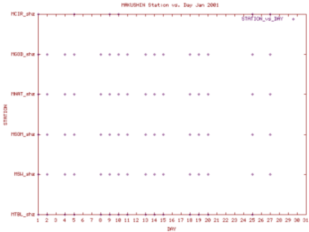
Station Use Plot for the Makushin subnet for January 2001
