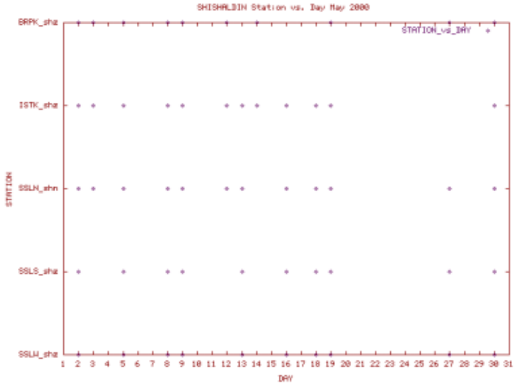
Station Use Plot for the Shishaldin subnet for May 2000
