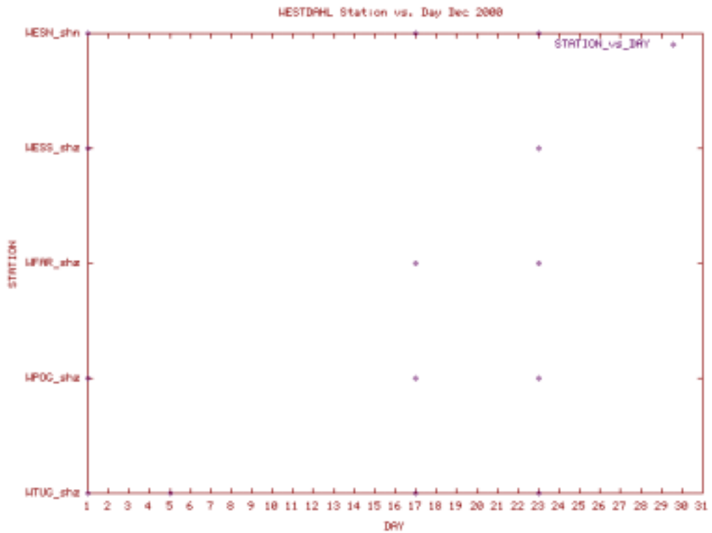
Station Use Plot for the Westdahl subnet for December 2000
