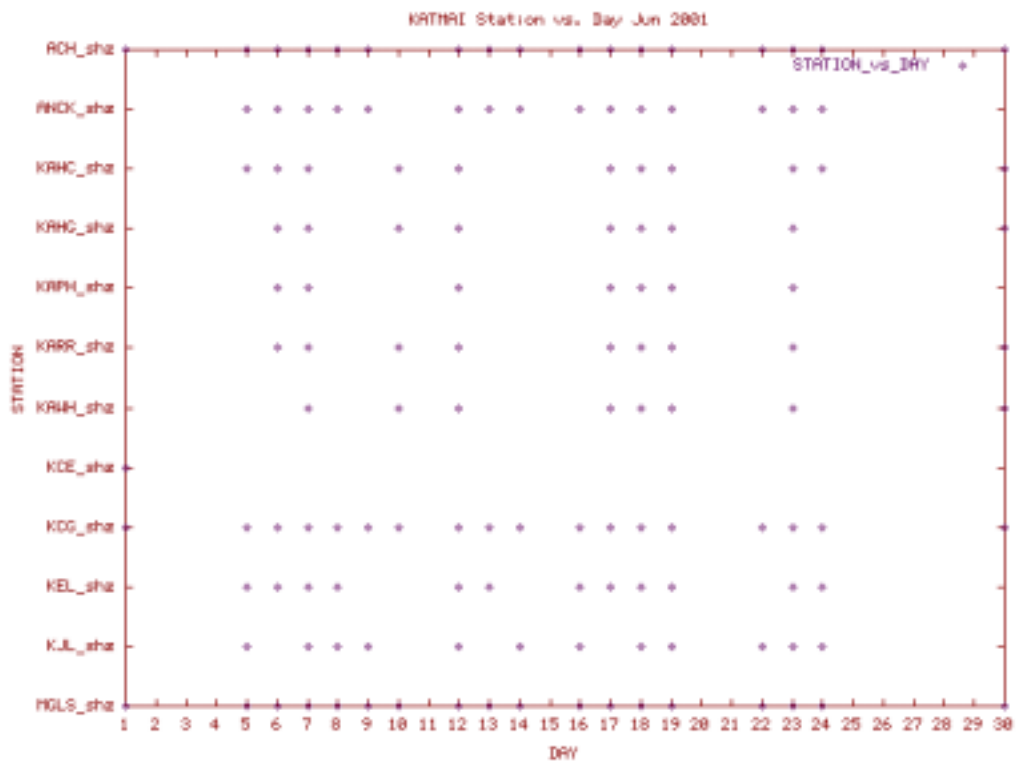
Station Use Plot for the Katmai volcanic group subnet for June 2001
