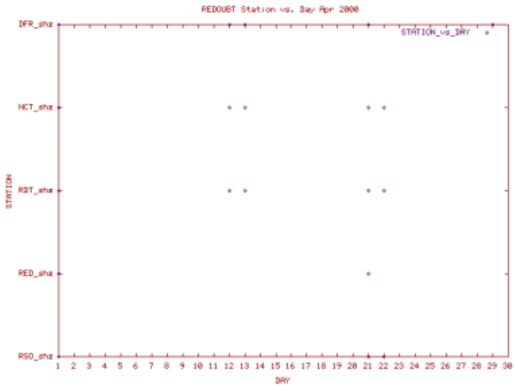
Station Use Plot for the Redoubt subnet for April 2000
