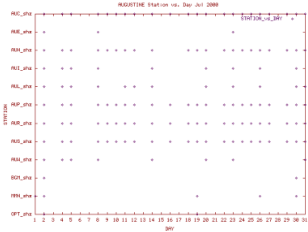
Station Use Plot for the Augustine subnet for July 2000
