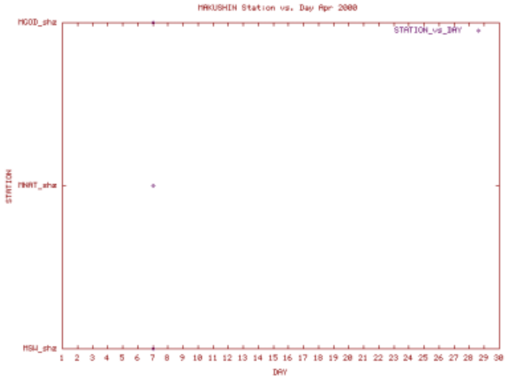
Station Use Plot for the Makushin subnet for April 2000
