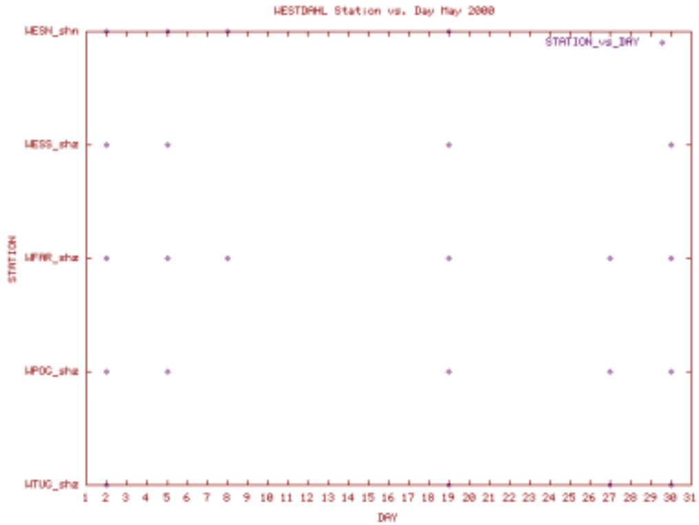
Station Use Plot for the Westdahl subnet for May 2000
