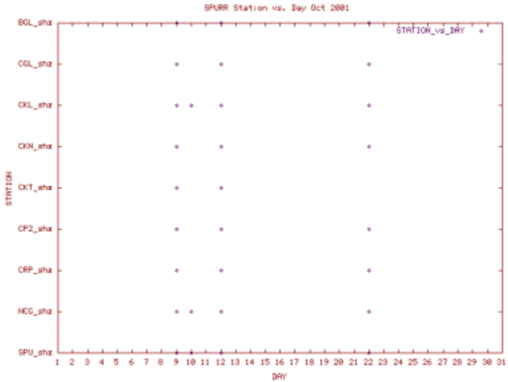
Station Use Plot for the Spurr subnet for October 2001
