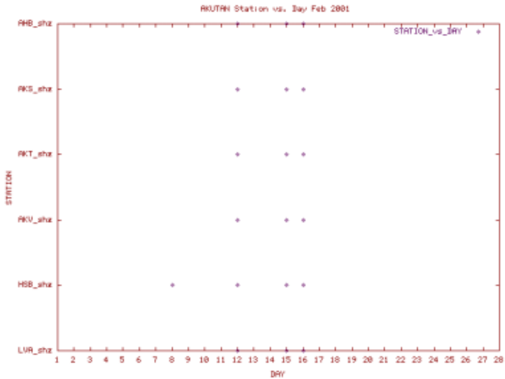
Station Use Plot for the Akutan subnet for February 2001
