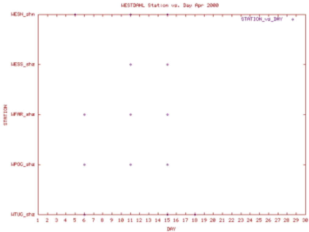
Station Use Plot for the Westdahl subnet for April 2000
