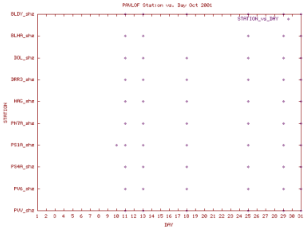
Station Use Plot for the Pavlof subnet for October 2001
