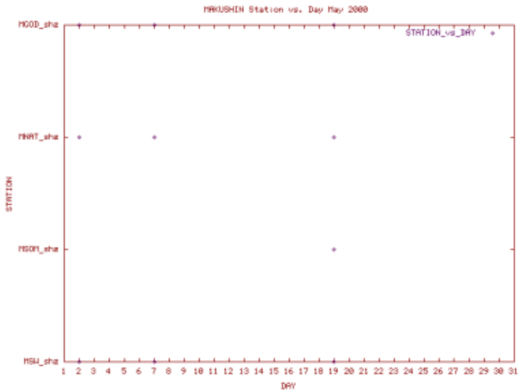
Station Use Plot for the Makushin subnet for May 2000
