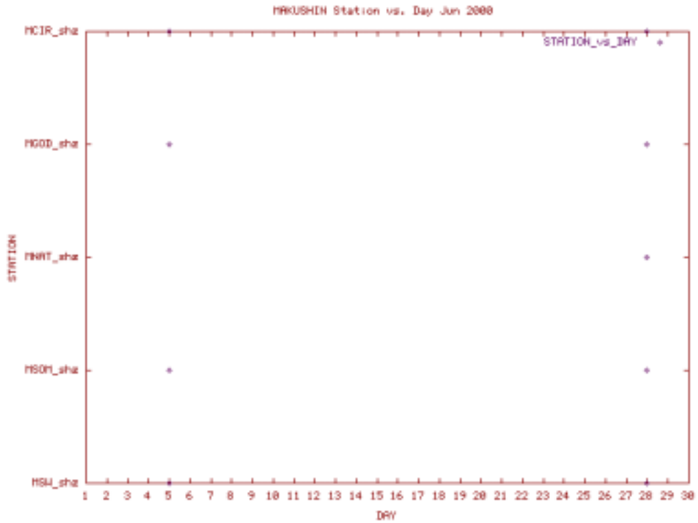
Station Use Plot for the Makushin subnet for Jun 2000
