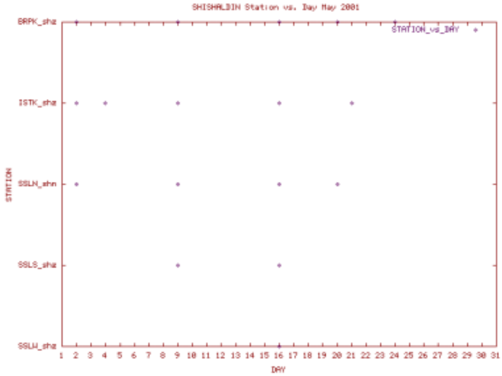
Station Use Plot for the Shishaldin subnet for May 2001
