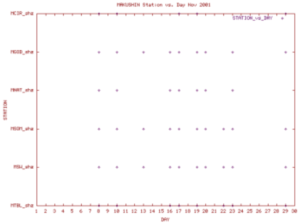
Station Use Plot for the Makushin subnet for November 2001
