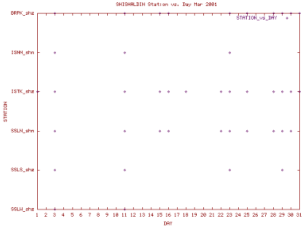
Station Use Plot for the Shishaldin subnet for March 2001
