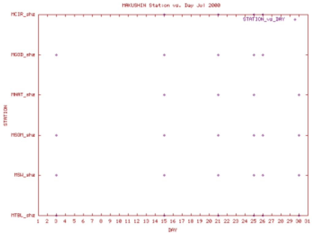
Station Use Plot for the Makushin subnet for July 2000
