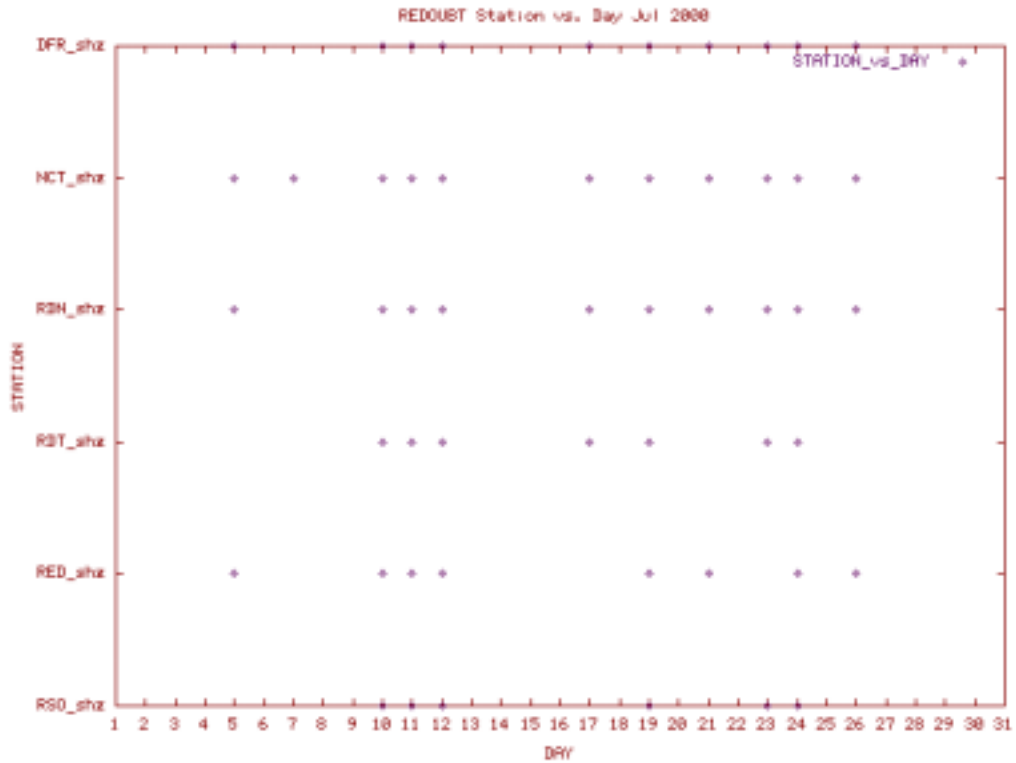
Station Use Plot for the Redoubt subnet for July 2000
