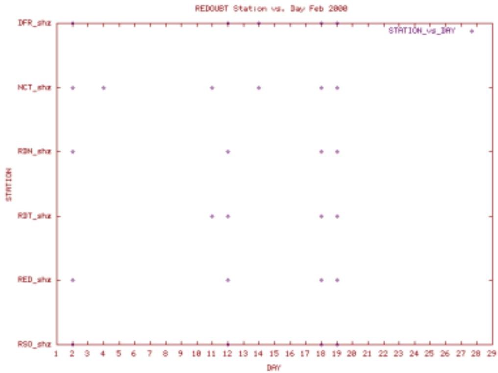
Station Use Plot for the Redoubt subnet for February 2000
