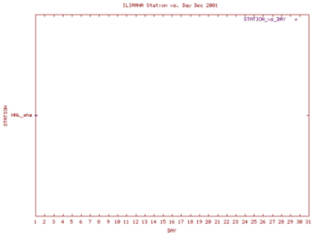
Station Use Plot for the Iliamna subnet for December 2001
