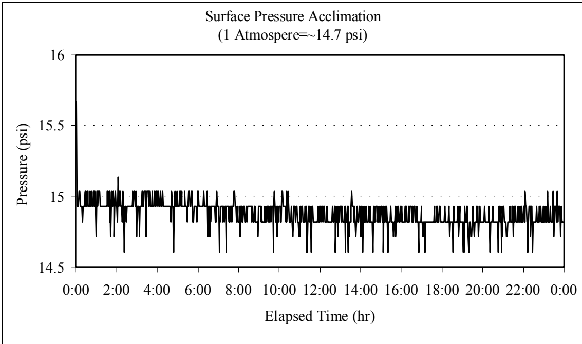
Figure A.1. Example of Surface Acclimation Pressure History
