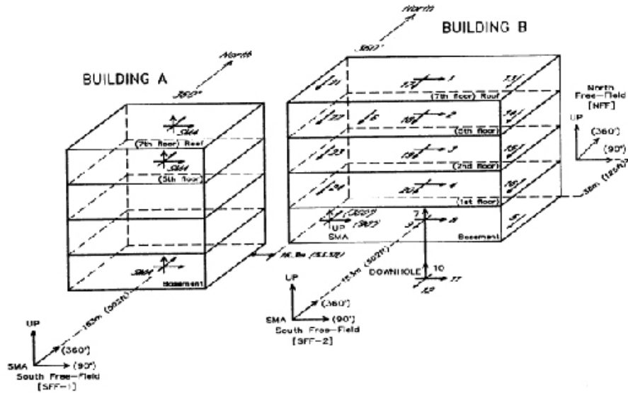
Figure 1. Two instrumented buildings in Norwalk, CA. Building B has a downhole instrument within a caisson.
