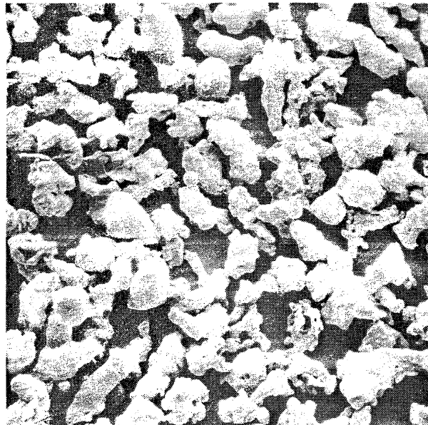
Figure 1. Scanning electron micrographs of the powders used to produce SRM 488. Mag. X160 a. as sized 310 stainless steel powder b. as sized 430 stainless steel powder
