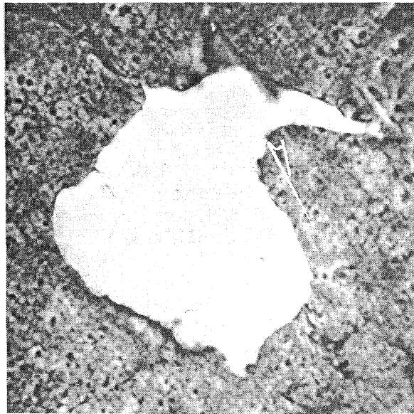
Figure 3. General microstructure of a compact. a. Optical micrograph showing the white austenite particles in the ferrite mixture. Mag. X50. b. Optical micrograph of an enlarged austenite particle. Mag. X800.
