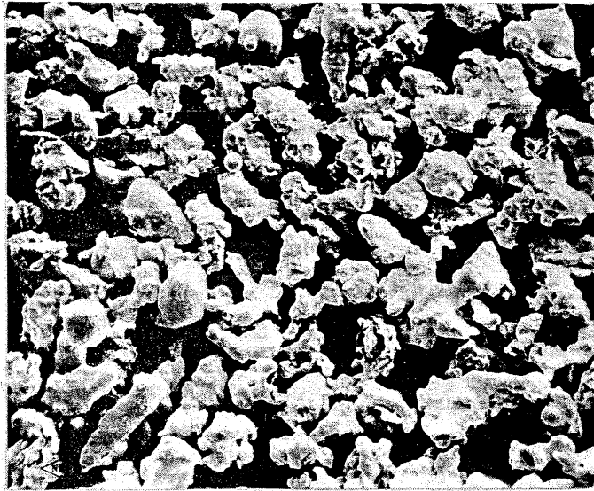
Figure 1. Scanning electron micrographs of the powders used to produce SRM 487. Mag. X160 a. as sized 310 stainless steel powder b. as sized 430 stainless steel powder
