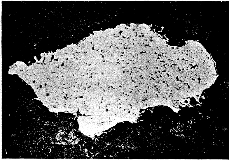
Figure 3. General Microstructure of a compact.
