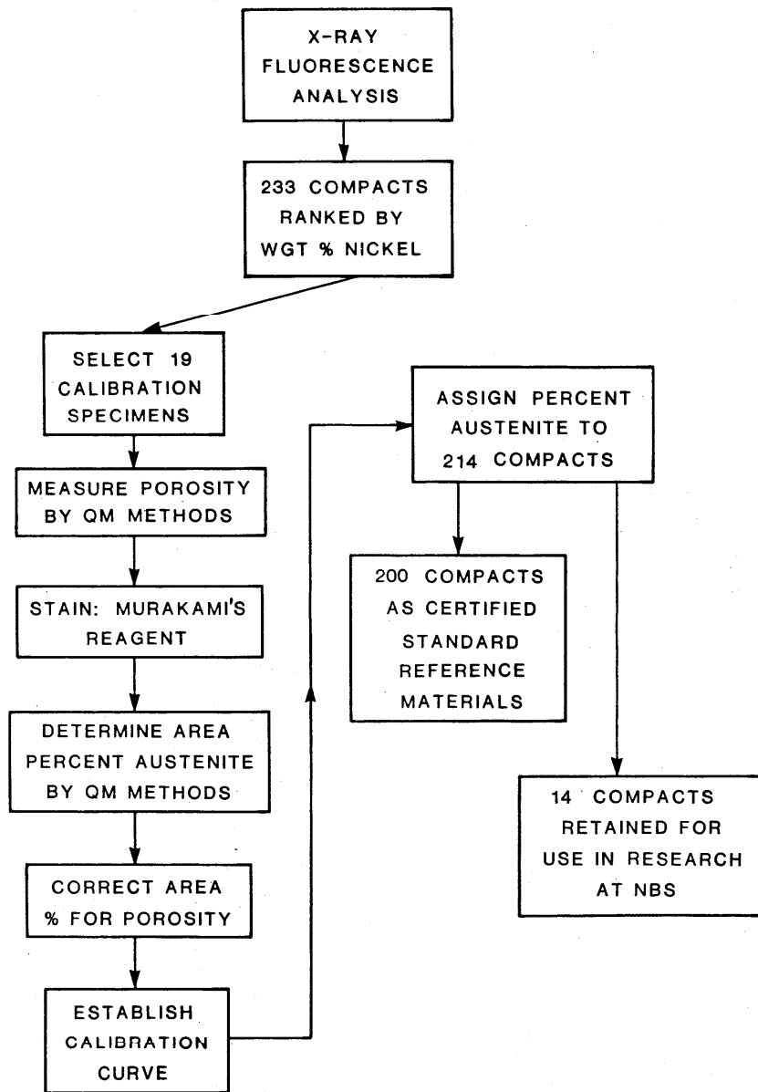
Figure 4. Characterization steps for SRM 487.
