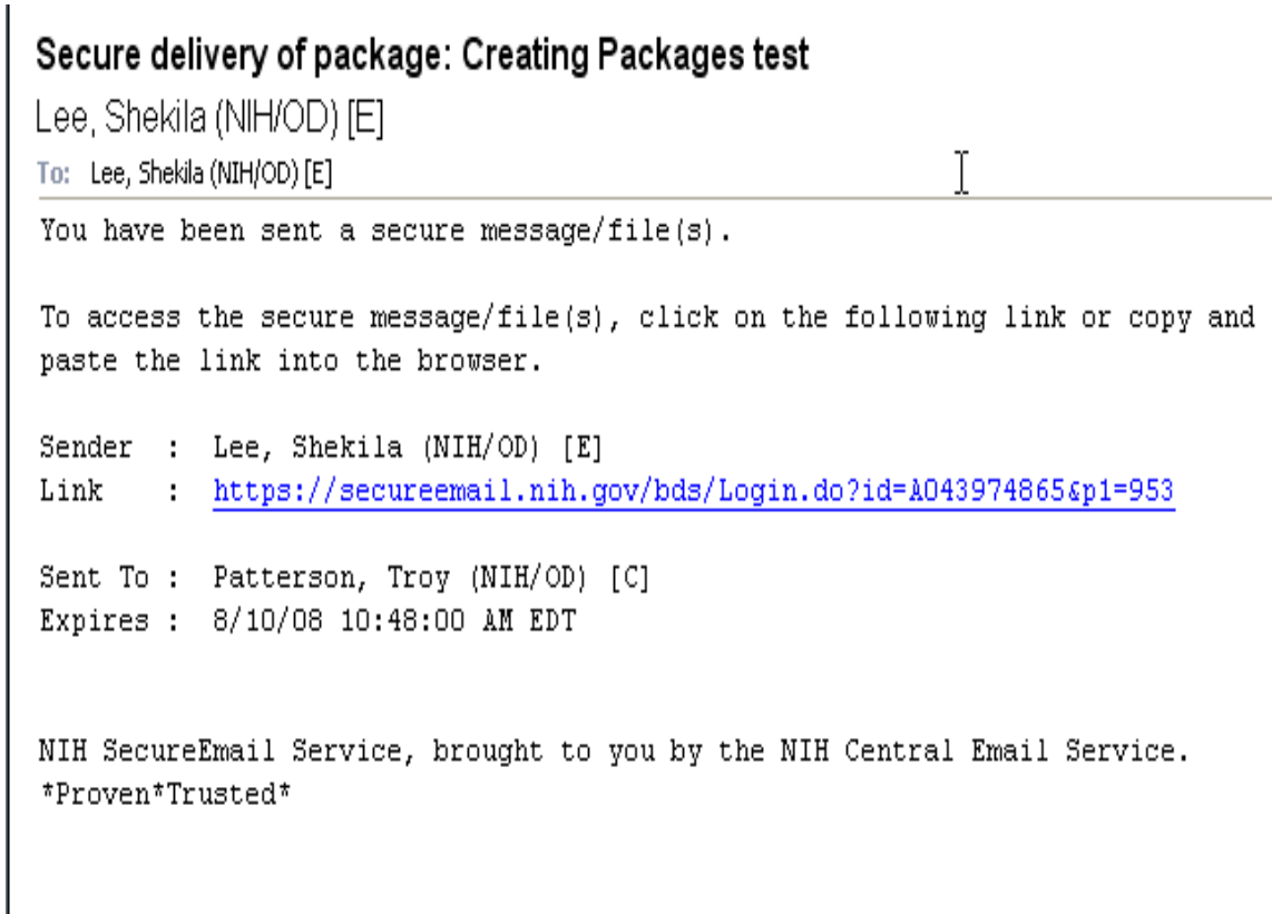
Fig. 18 – Notification Message
