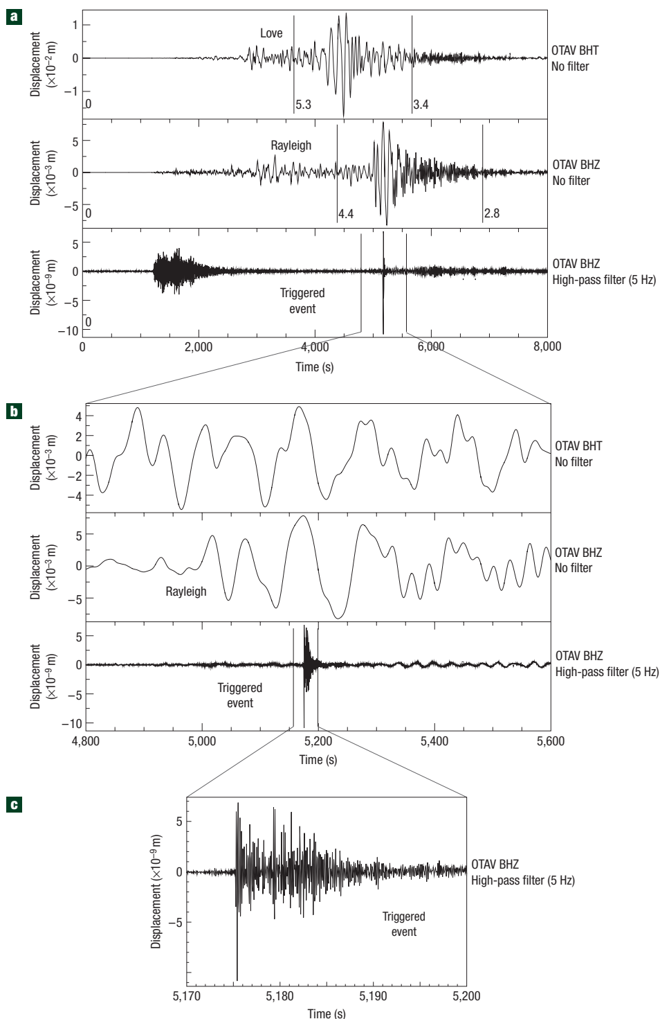
Figure 1 Transverse (BHT) and vertical (BHZ) displacement seismograms for the 26 December 2004, Sumatra ( M = 9.2 ) earthquake. a , Recorded at the station in Otavalu, Ecuador, OTAV ( \Delta = 173^\circ ), showing unfiltered Love and Rayleigh waves and the high-pass-filtered (at 5 Hz) vertical component. b , Same as in a , but with a reduced time (time divided by velocity) window showing the strong Rayleigh-wave arrival and the triggered event. c , Window of only the triggered event.
