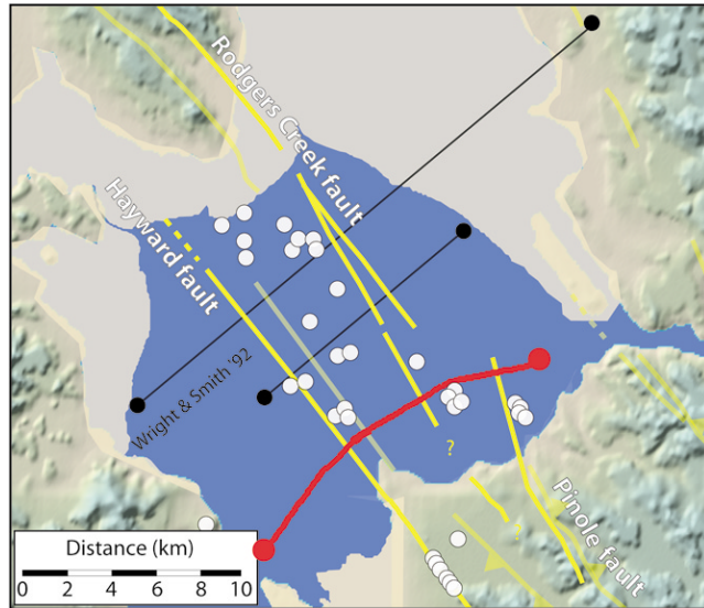
Figure 3. Fault map of San Pablo Bay based on the cross sections of Wright and Smith (1992) (cross-section locations shown with black lines) and our new section in south San Pablo Bay (cross-section location shown with red line). We carry the Pinole fault offshore at least as far north as our cross section, and we connect the Rodgers Creek fault as far south as our section.
