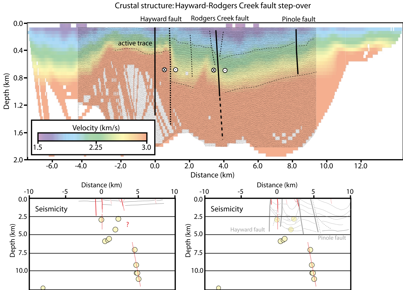
Figure 2. A structural cross section (upper 2 km) across south San Pablo Bay and the Hayward–Rogers Creek step-over (see Fig. 1 for location). Seismic reflection data are overlain on a tomographic seismic velocity section. A significant lateral contrast is observed about 1 km east of the presently active trace of the Hayward fault and may represent an older fault trace. Another fault ~4 km east of the active Hayward fault separates east-dipping from west-dipping bedding within a basin; this structure is located on the Rodgers Creek fault trend projected from two structural sections in central and north San Pablo Bay developed by Wright and Smith (1992). Sparse relocated earthquake hypocenters (Waldhauser and Ellsworth, 2002) are shown in the lower panels with and without the Wright and Smith (1992) interpretation.
