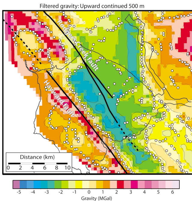
Figure 5. Gravity map of the San Pablo Bay region. An upward continued (500 m) signal was subtracted from the data, which filters out the broader wavelength features and allows us to focus on the shallowest part of the crust. A simplified fault map is shown by the black lines, and gravity gradients are identified by the white dots. A broad gravity low characterizes San Pablo Bay, and a subtly lower anomaly appears to coincide with the region between the Hayward and Rodgers Creek faults. This low is truncated near the north edge of San Pablo Bay by a strong gravity gradient that might be a normal fault boundary of a pull-apart basin.
