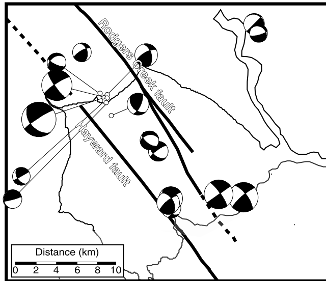
Figure 4. Earthquake focal mechanisms from the Northern California Seismic Network catalog 1967–2002 located within the Hayward–Rodgers Creek fault step-over in San Pablo Bay.
