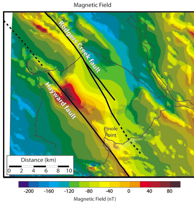
Figure 6. Aeromagnetic map of San Pablo Bay. The continuous magnetic high that trends across central San Pablo Bay between the Hayward and Rodgers Creek faults was interpreted by Jachens et al. (2002) as evidence for the lack of a strike-slip transfer fault across the step-over.
