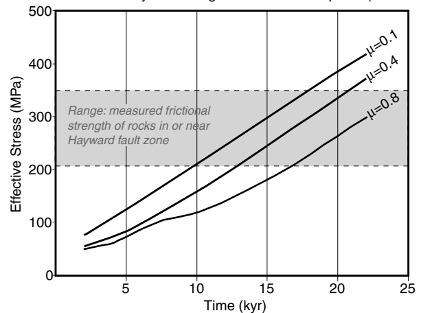
Figure 9. Differential stressing rate within the Hayward–Rodgers Creek step-over predicted from finite-element modeling. Three curves show the rates for different coefficients of friction of the strike-slip faults. In all cases the stressing rate is about 0.02 MPa/yr. The gray area on the plot shows the range of measured frictional strength of rocks near the Hayward fault (Morrow and Lockner, 2001)
