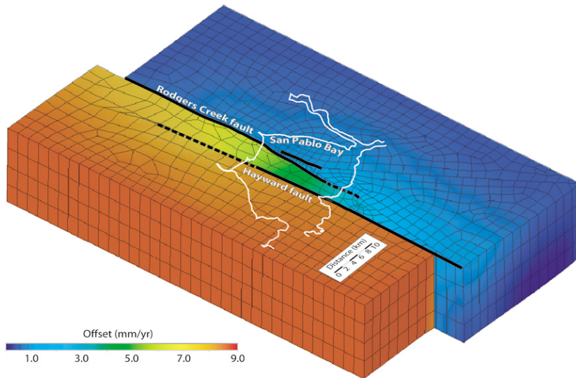
Figure 7. Finite-element model of the elastic part of the Hayward–Rodgers Creek step-over (upper 15 km). The west edge of the model was moved at a 9-mm/yr rate past the fixed east edge. The model is shaded by the relative fault-parallel displacement.
