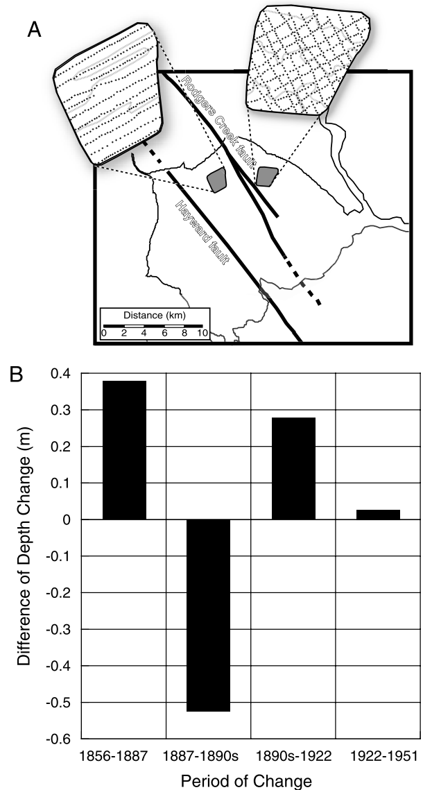
Figure 11. (A) Location of areas where historical hydrographic surveys were used to determine if the 1898 earthquake caused vertical bay-floor displacement. Depth soundings and contours from the 1890s within each shaded area are shown in the expanded views. (B) Difference in depth change in the shaded areas in panel A. A negative value is less deposition (more erosion) or downward vertical displacement in the area between the faults.
