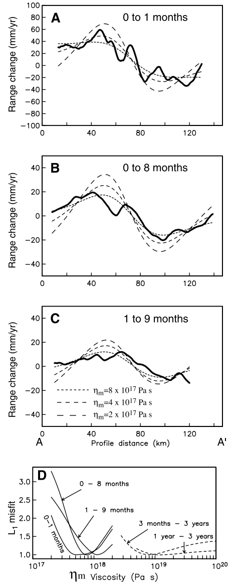
Fig. 3. Observed unwrapped range change along profile A-A' (Fig. 1) for the time periods (A) 20 October 1999 to 24 November 1999 (0 to 1 month), (B) 20 October 1999 to 21 June 2000 (0 to 8 months), and (C) 24 November 1999 to 26 July 2000 (1 to 9 months). Superimposed are viscoelastic model predictions for three possible values of mantle viscosity. (D) Solid curves: L_1 -norm misfit of observed post-Hector Mine range change along profile A-A' with respect to the viscoelastic model as a function of \eta_m , with absolute minima normalized to unity. Dashed curves: misfit of observed post-Landers range change with respect to the viscoelastic model derived with interferograms from 3 months to 3 years (16) and 1 year to 3 years (33) after the Landers earthquake. In all cases, a fixed ratio of \eta_c/\eta_m = 27 is assumed.
