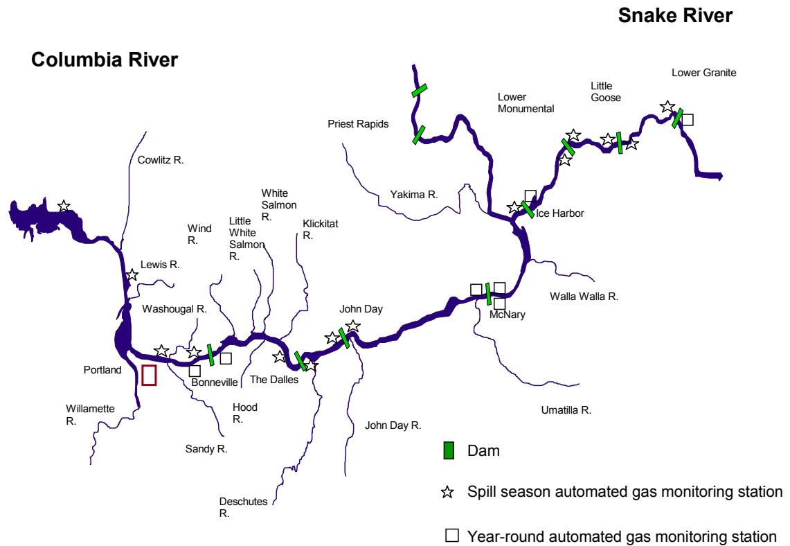
Figure 6. Locations of dissolved gas monitoring stations in the Lower Columbia and Snake rivers.
