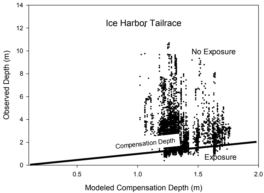
Figure 12. Relationship between the MASS2 modeled compensation depth (depth where there is complete hydrostatic compensation) relative to the actual recorded depth of adult spring-summer Chinook salmon in the Bonneville Dam tailrace (top) and the Ice Harbor Dam tailrace (bottom) during the spring and summer of 2000.
