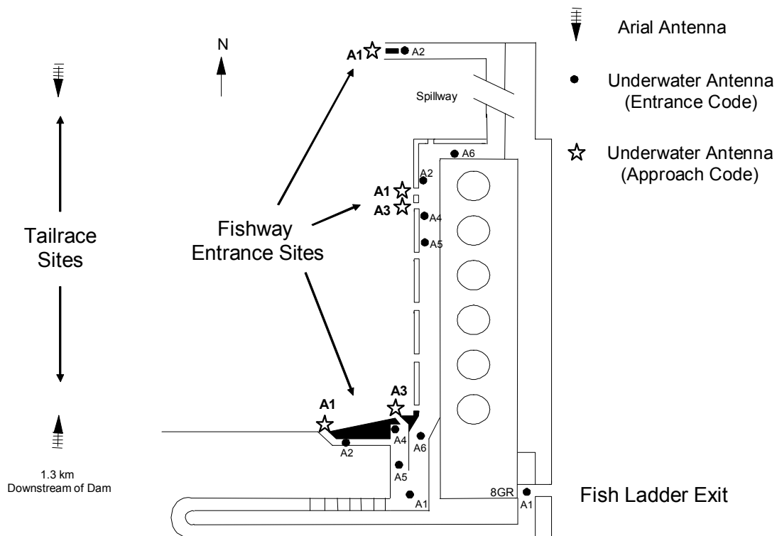
Figure 5. Diagram of Lower Granite Dam with location of aerial tailrace antennas and fixed underwater antennas.
