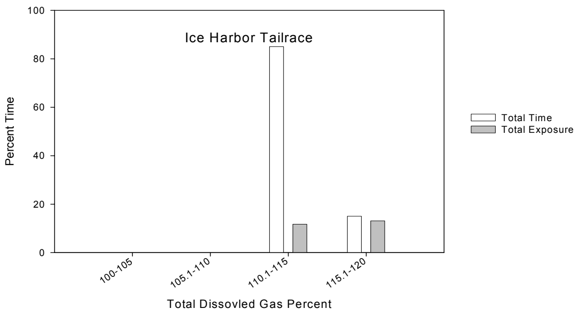
Figure 13. Total exposure relative to the amount of time at various categories of dissolved gas supersaturation.
