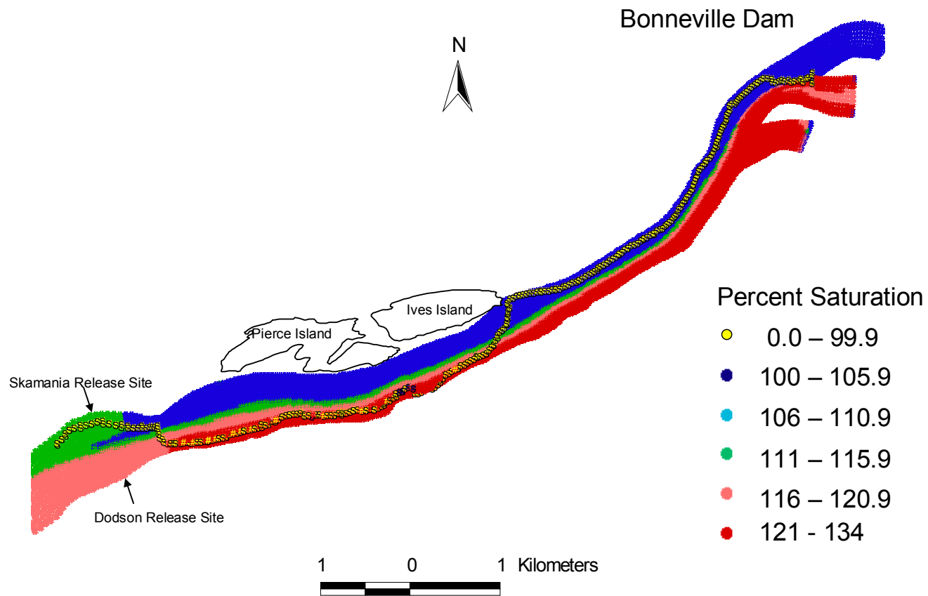
Figure 4. Simulated (MASS2) percent saturation on 24 July 2000 downstream from Bonneville Dam. Circles represent locations for fish (RDST #2435A). The circle color represents the magnitude of post compensation exposure (percent saturation equivalent to what the fish would experience after taking into consideration hydrostatic compensation).
